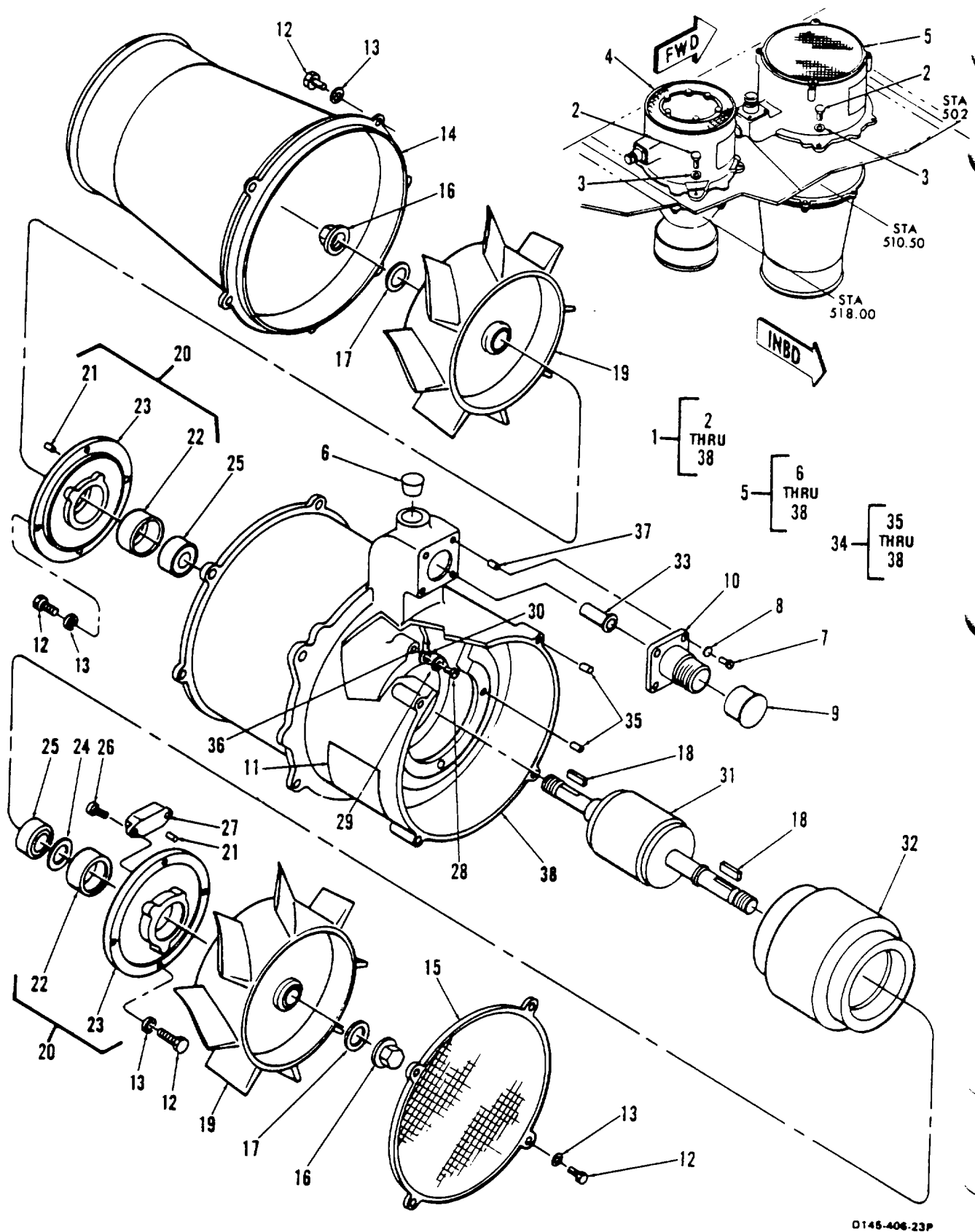
Figure 241. Equipment Instl, Cooling Fan, Aft Pylon
