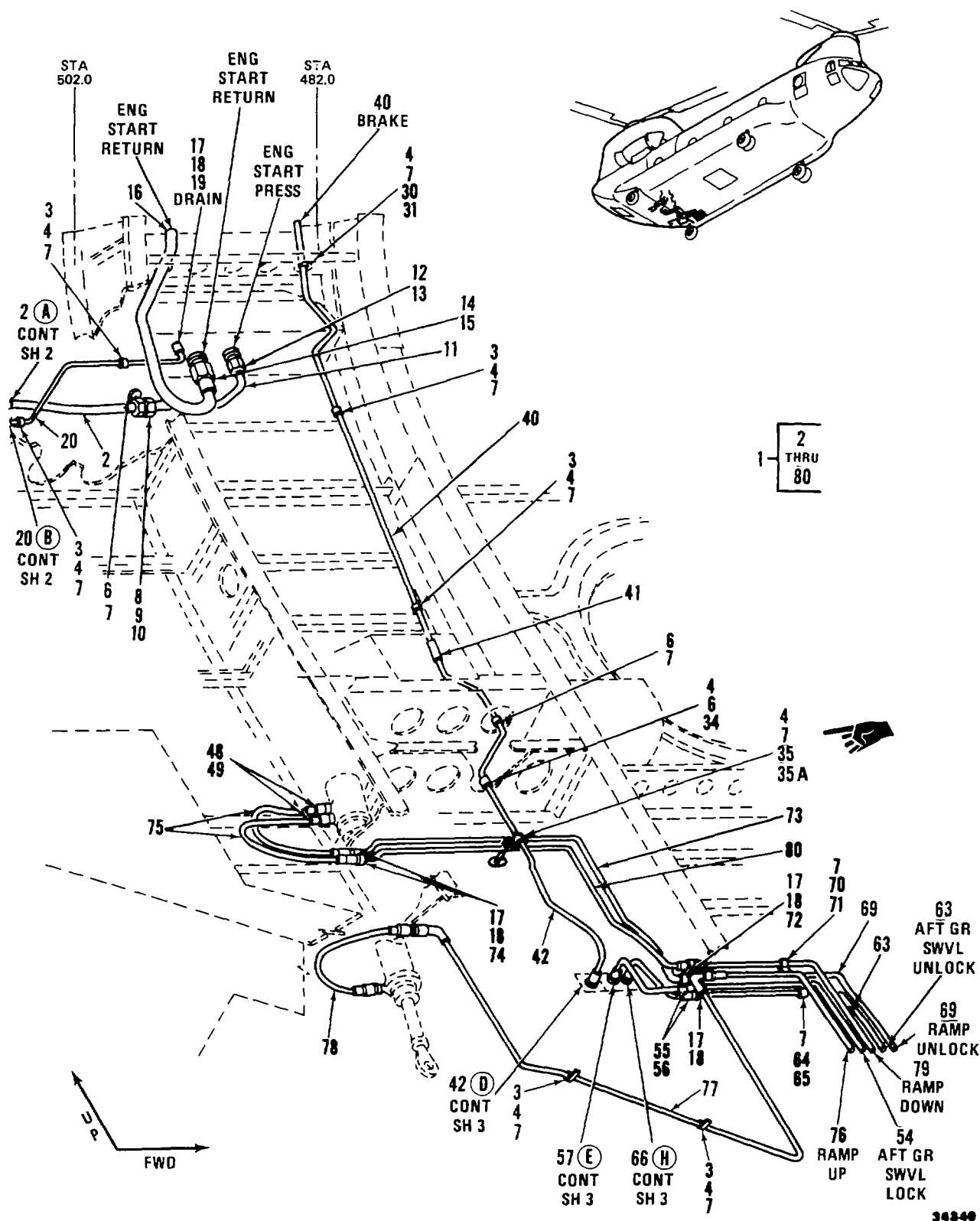
Figure 267. Tubing Instl, Lower Aft Fuselage, Sta 440 to 594 (Sheet 1 of 3)
