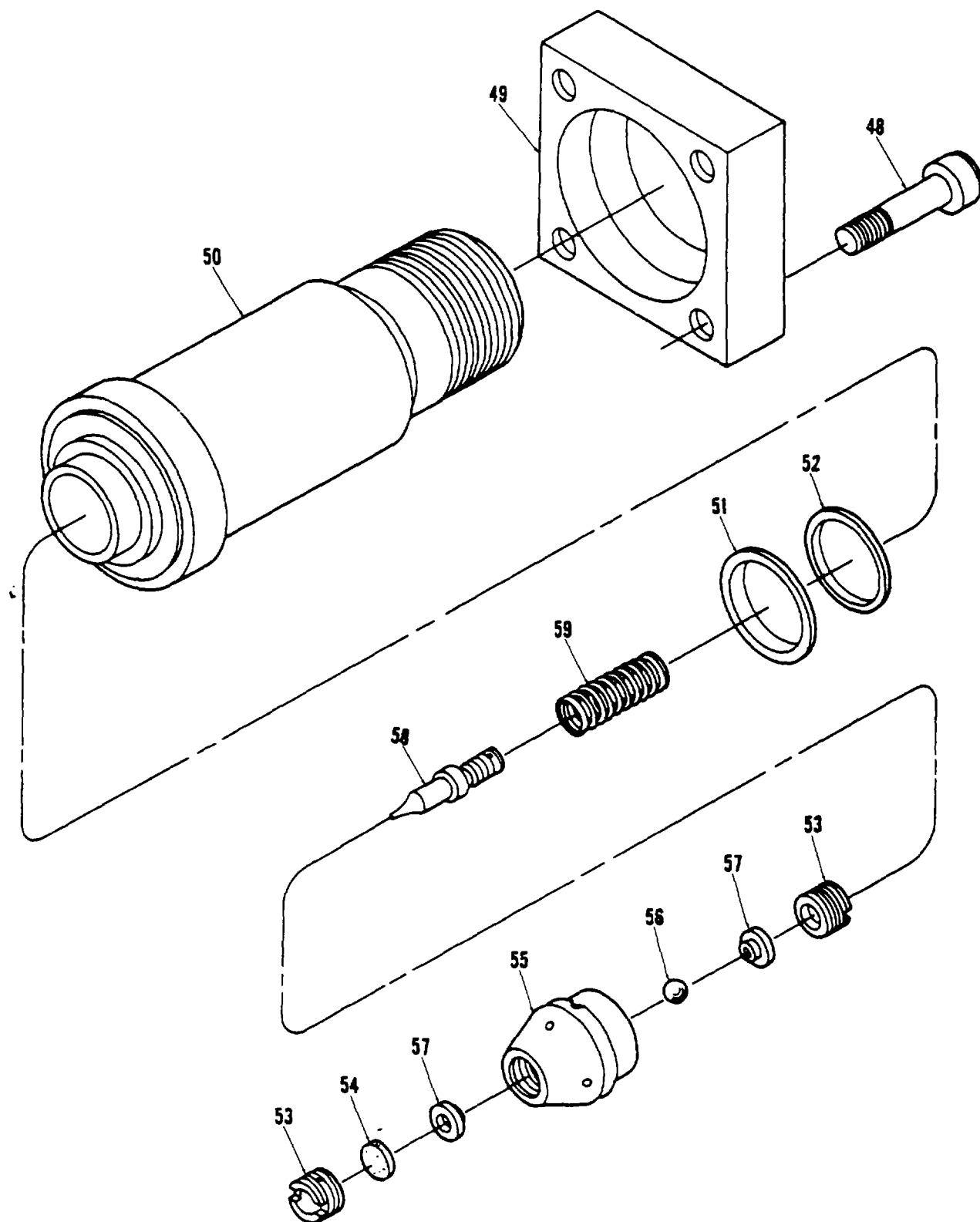
Figure 204. Valve, Solenoid HP1322100-6 (Sheet 4 of 4)
