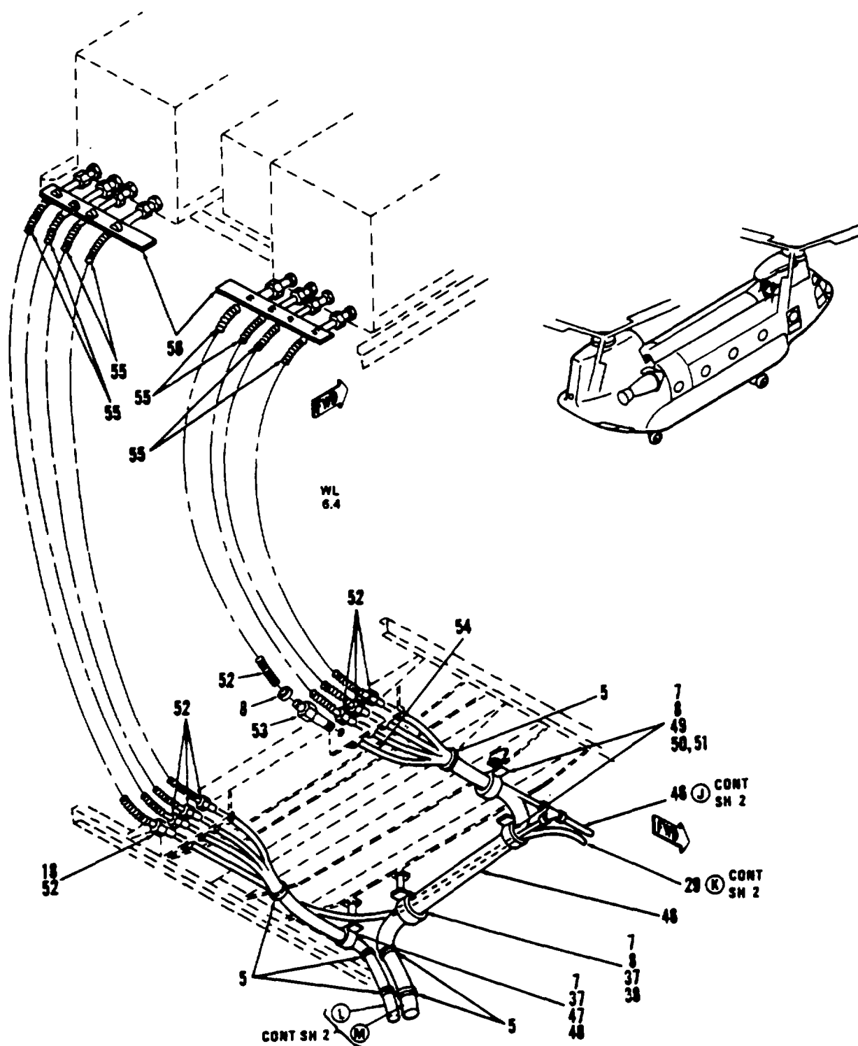
Figure 296. Tubing Instl, Equipment, Crown Panel and Side, LH Sta 120 to 160 (Sheet 3 of 3)
