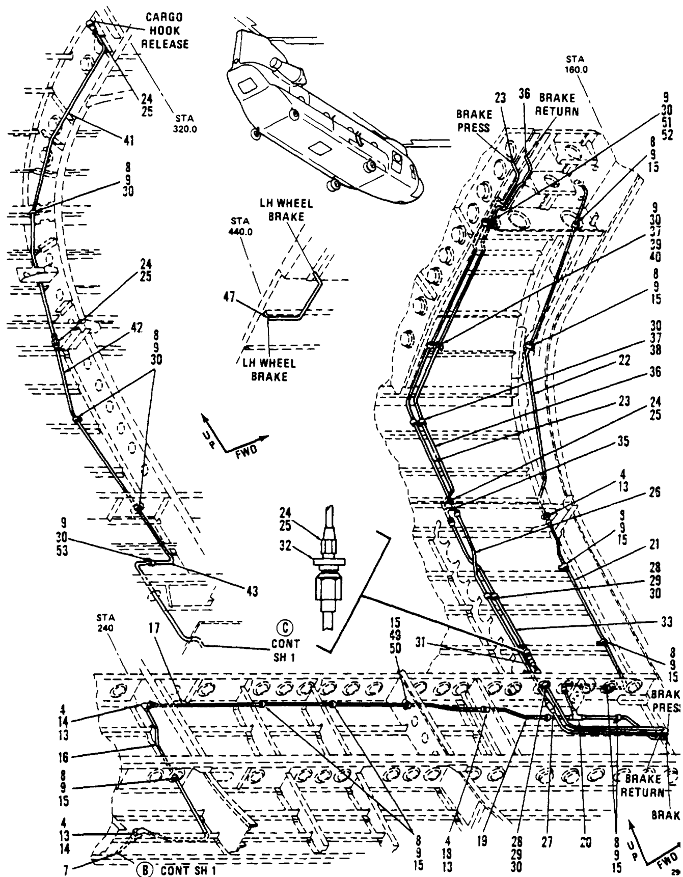
Figure 263. Tubing Instl, Hydraulic, Cabin Ceiling and Side, Lower, LH, Sta 160 to 440 (Sheet 2 of 2)
