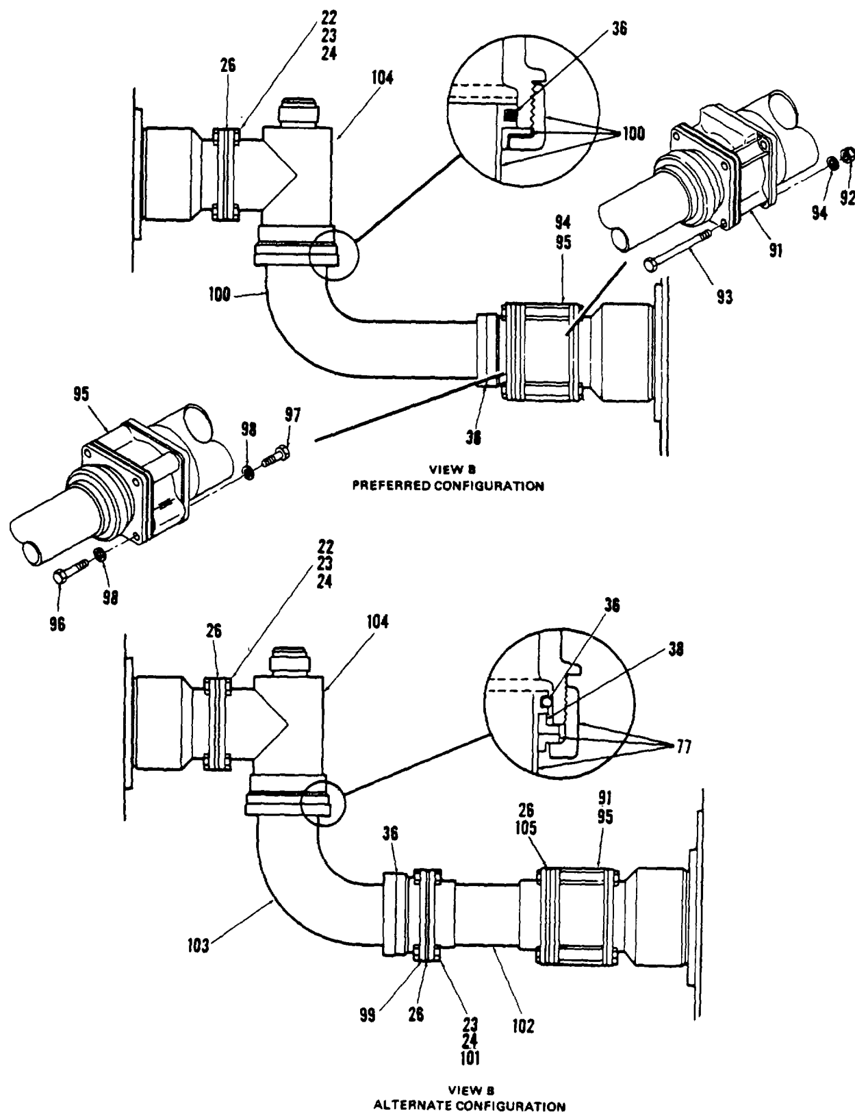
Figure 347. Intertank connection Instl, LH (Sheet 3 of 5)
