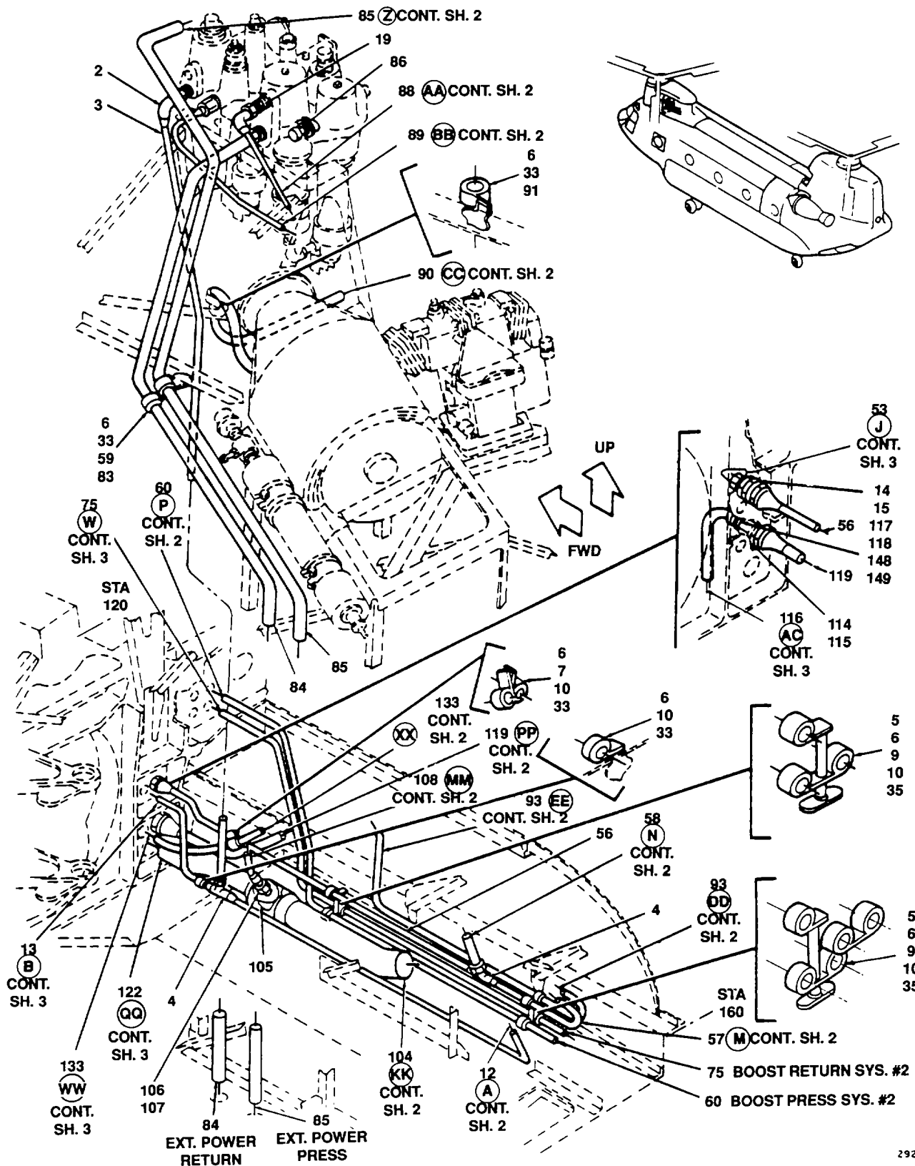
Figure 262. Tubing Instl, Hydraulics, Actuators, Fwd Transmission, Flight Controls Compartment, and Fwd Pylon (Sheet 1 of 6)
