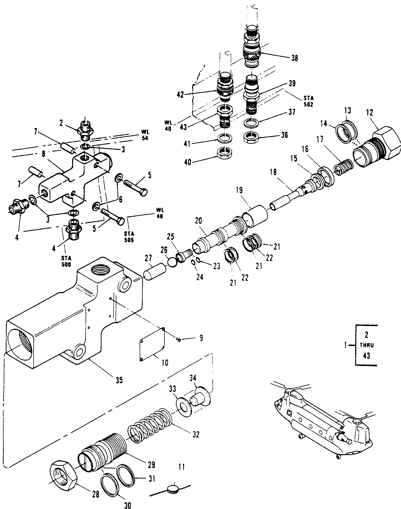
Figure 208. Equipment Instl, Sta 502, LH, Below WL 72
