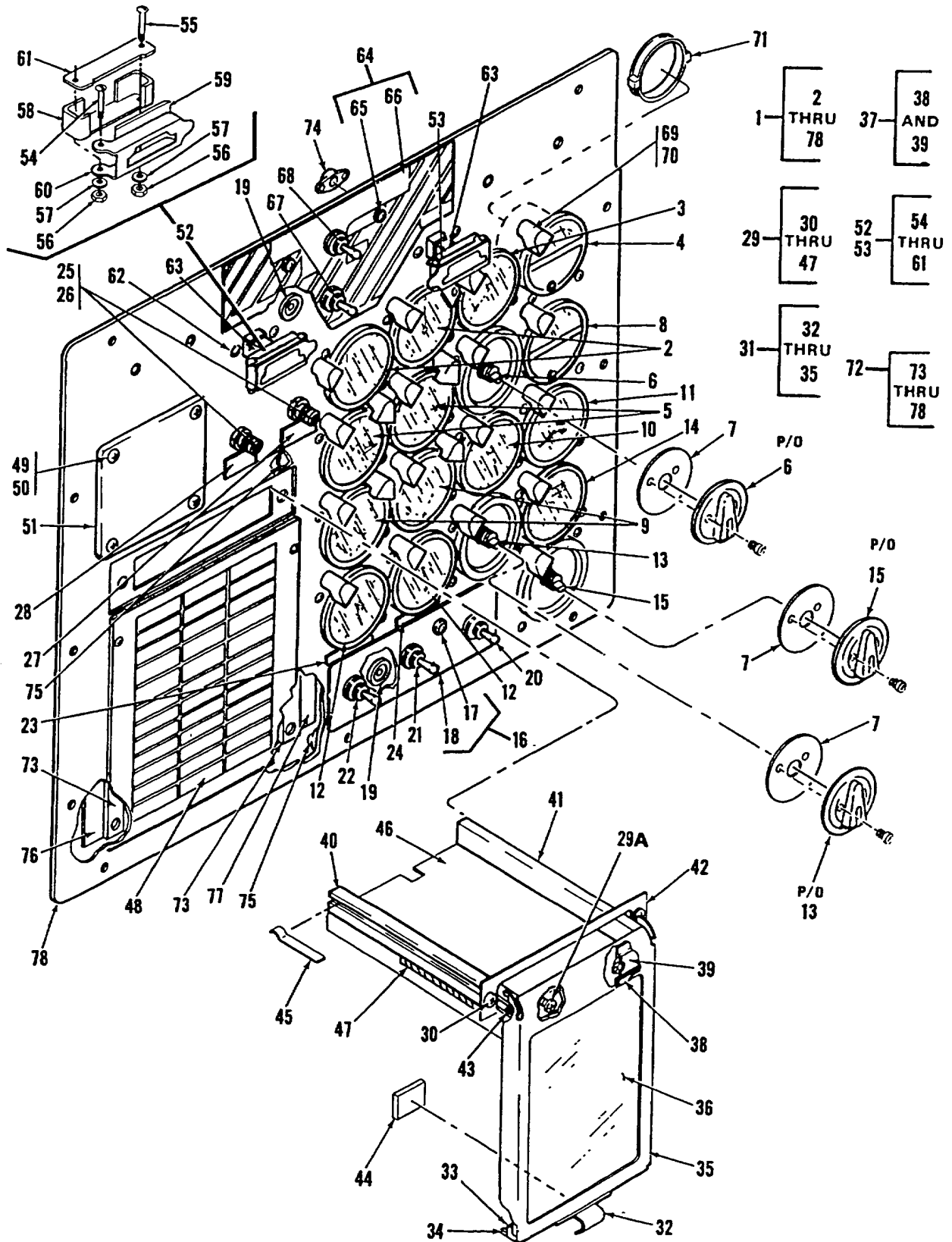
Figure 276. Panel, Instrument, Center (T55-L-712 Engine)
