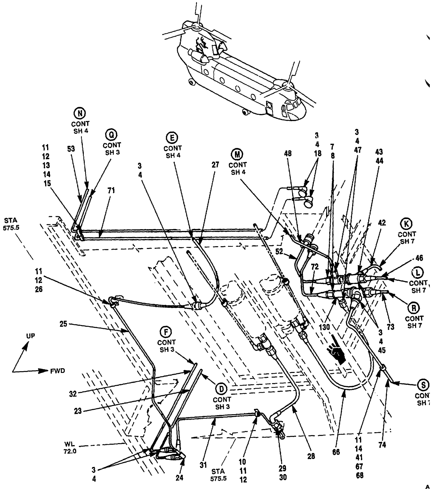
Figure 273. Tubing Instl, Aft Pylon and Combining Transmission Area (Sheet 5 of 7)
