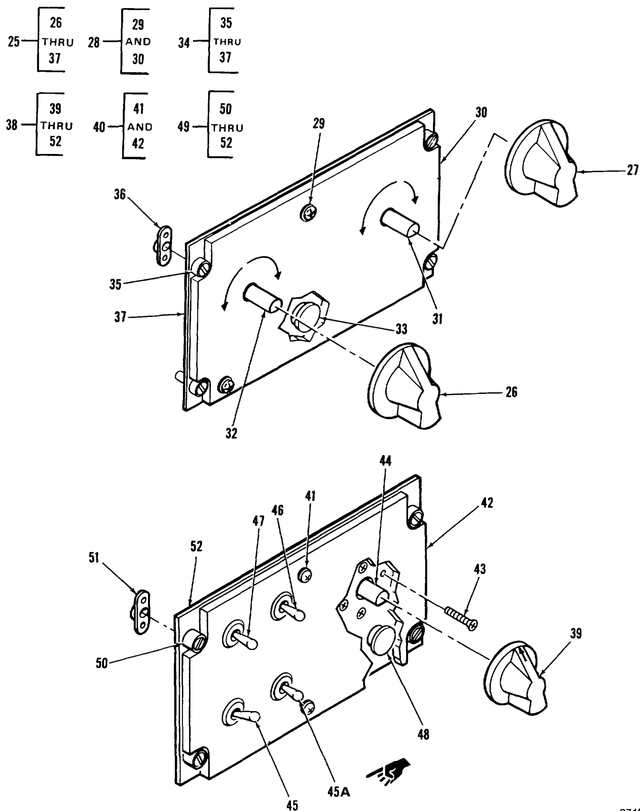
Figure 317. Panel, Anti-Ice, Interior Lighting and Stick Position Indicator (Sheet 2 of 2)
