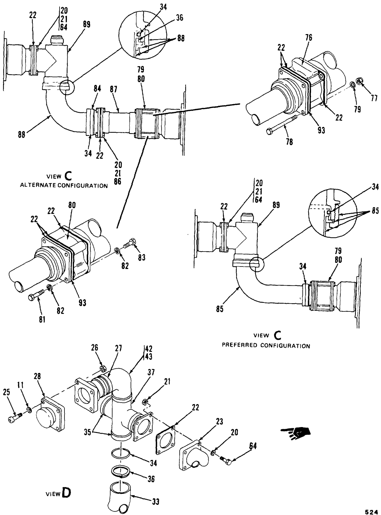
Figure 348. Intertank Connection Instl, RH (Sheet 3 of 5)
