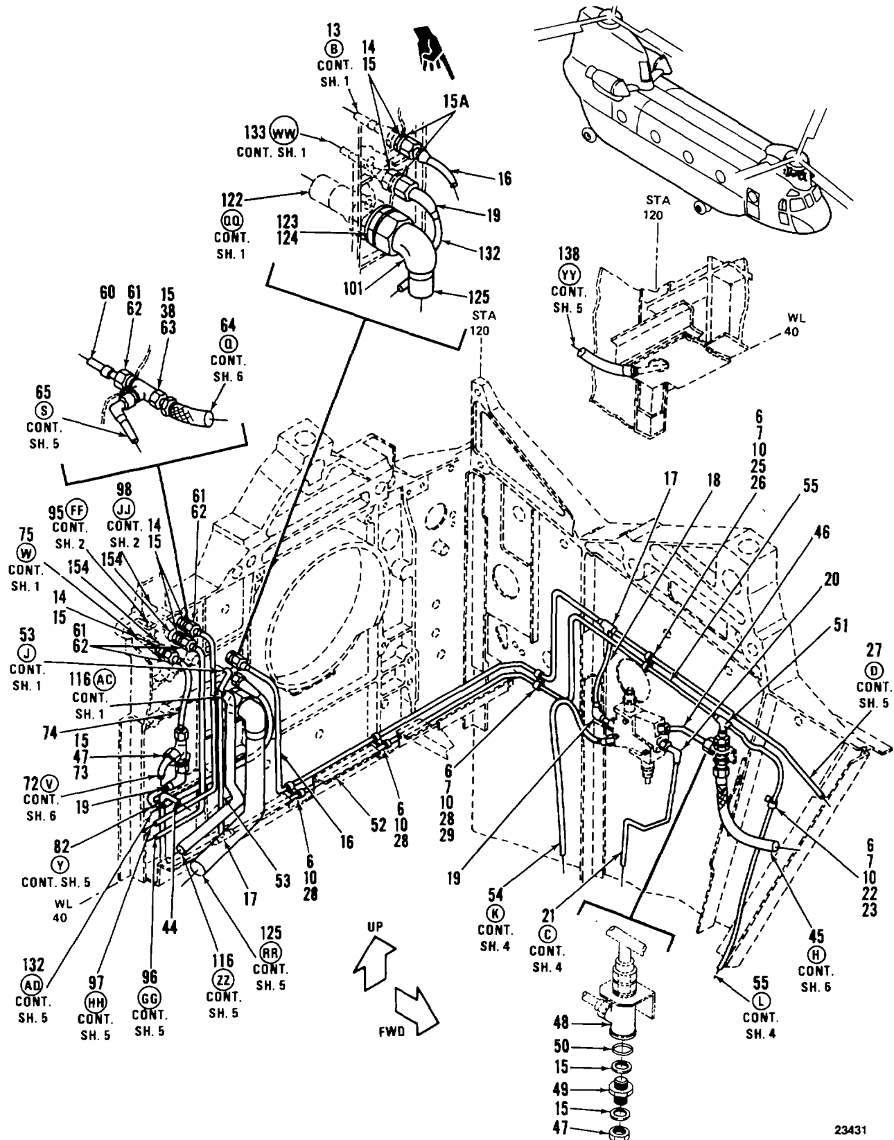
Figure 262. Tubing Instl, Hydraulics, Actuators, Fwd Transmission, Flight Controls Compartment, and Fwd Pylon (Sheet 3 of 6)
