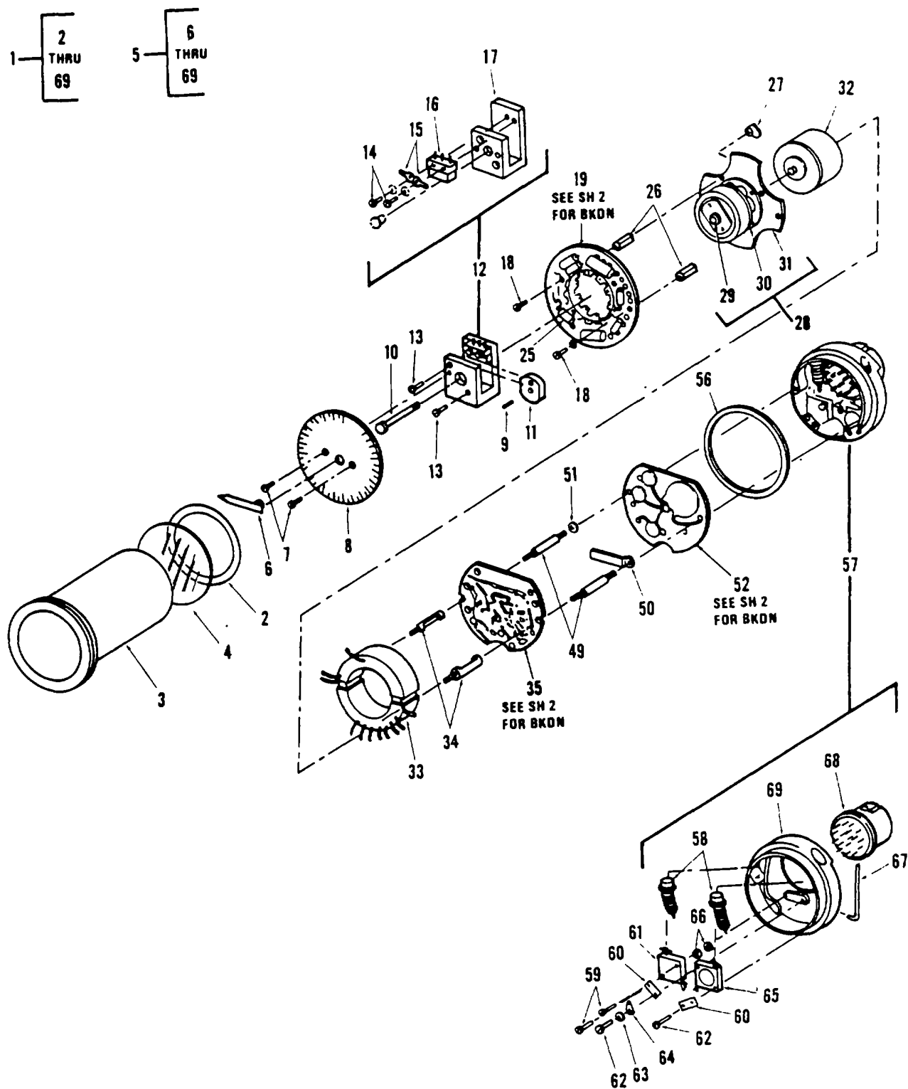
Figure 279. Indicator, Oil Temperature (Sheet 1 of 2)
