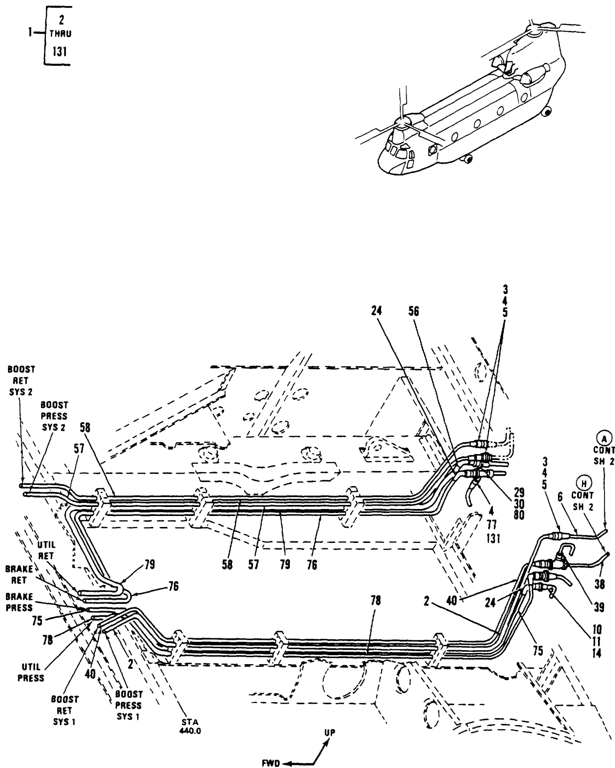
Figure 273. Tubing Instl, Aft Pylon , and Combing Transmission Area (Sheet 1 of 7)
