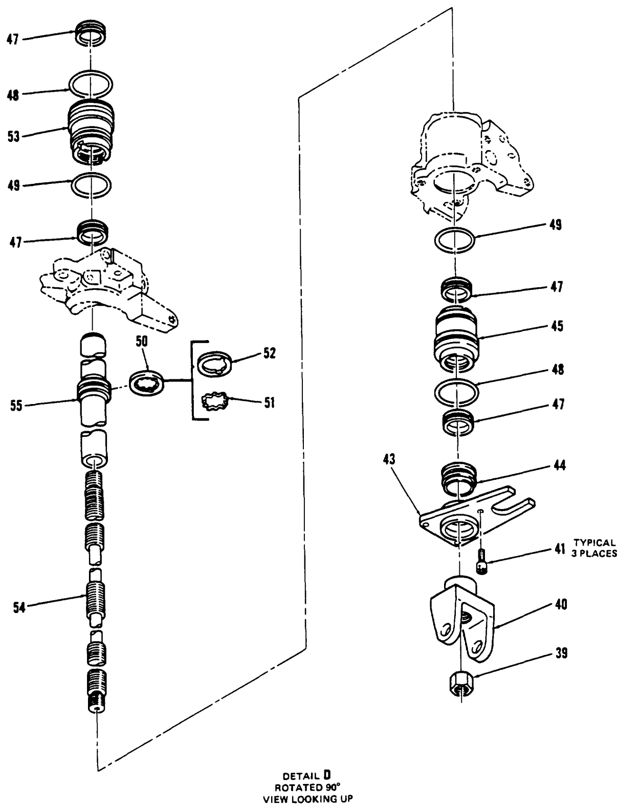
Figure 252. Actuator, Thrust (Sheet 4 of 5)
