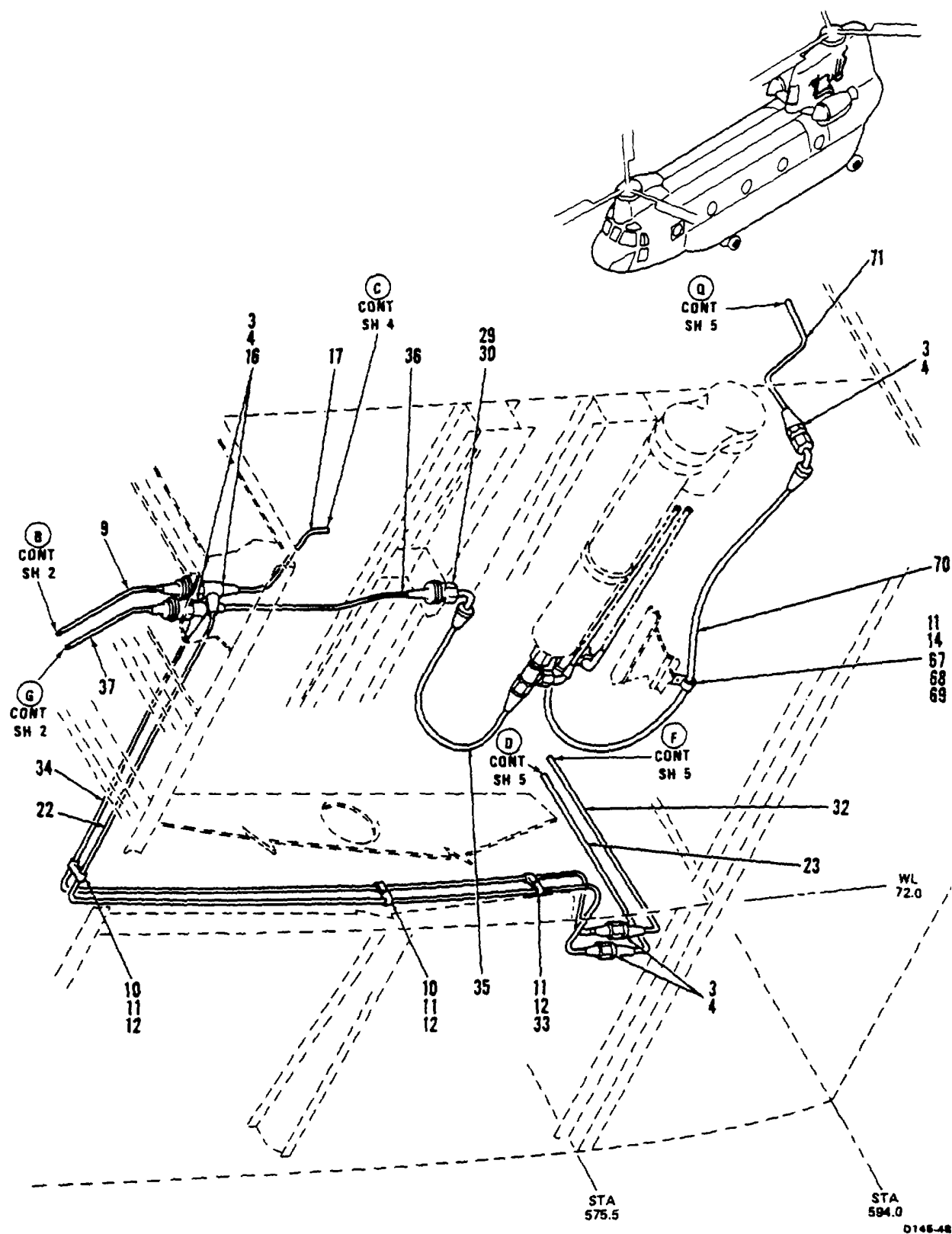
Figure 273. Tubing Instl, Aft Pylon , and Combing Transmission Area (Sheet 3 of 7)
