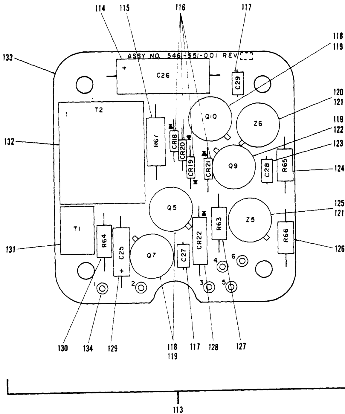
Figure 289. Signal Conditioner, Indicator, Liquid (Sheet 3 of 5)
