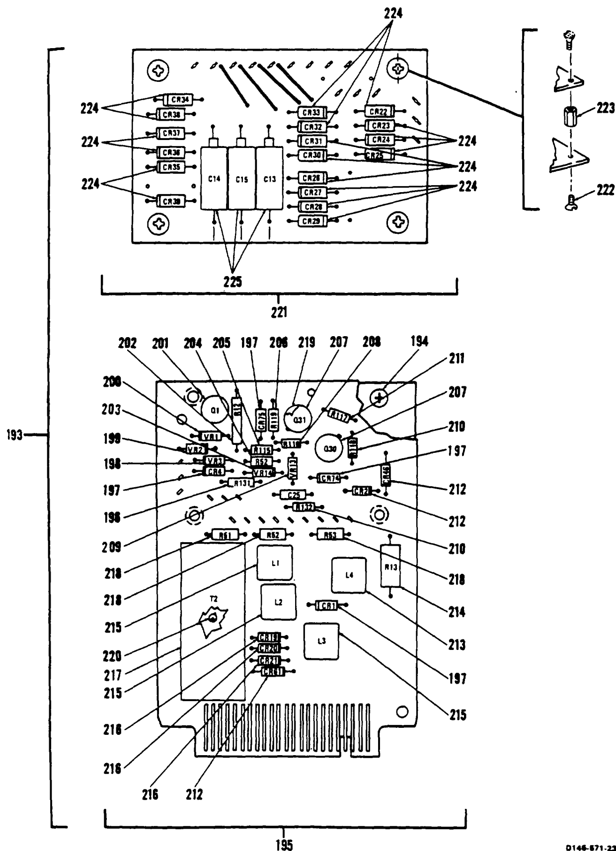
Figure 322. Panel, Generator Control (Sheet 5 of 5)
