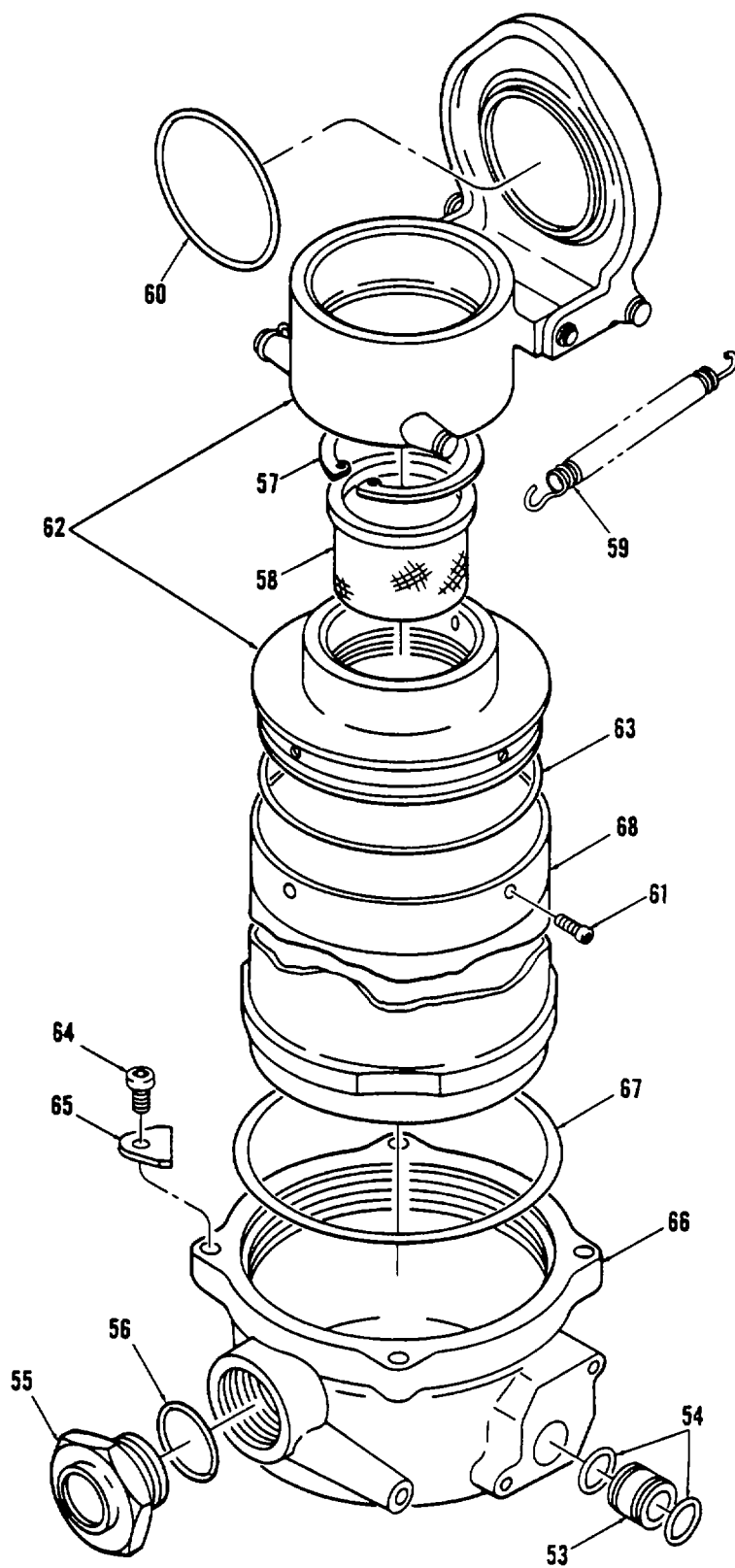
Figure 211. Fill Module, Hyd Pump (Sheet 2 of 2)
