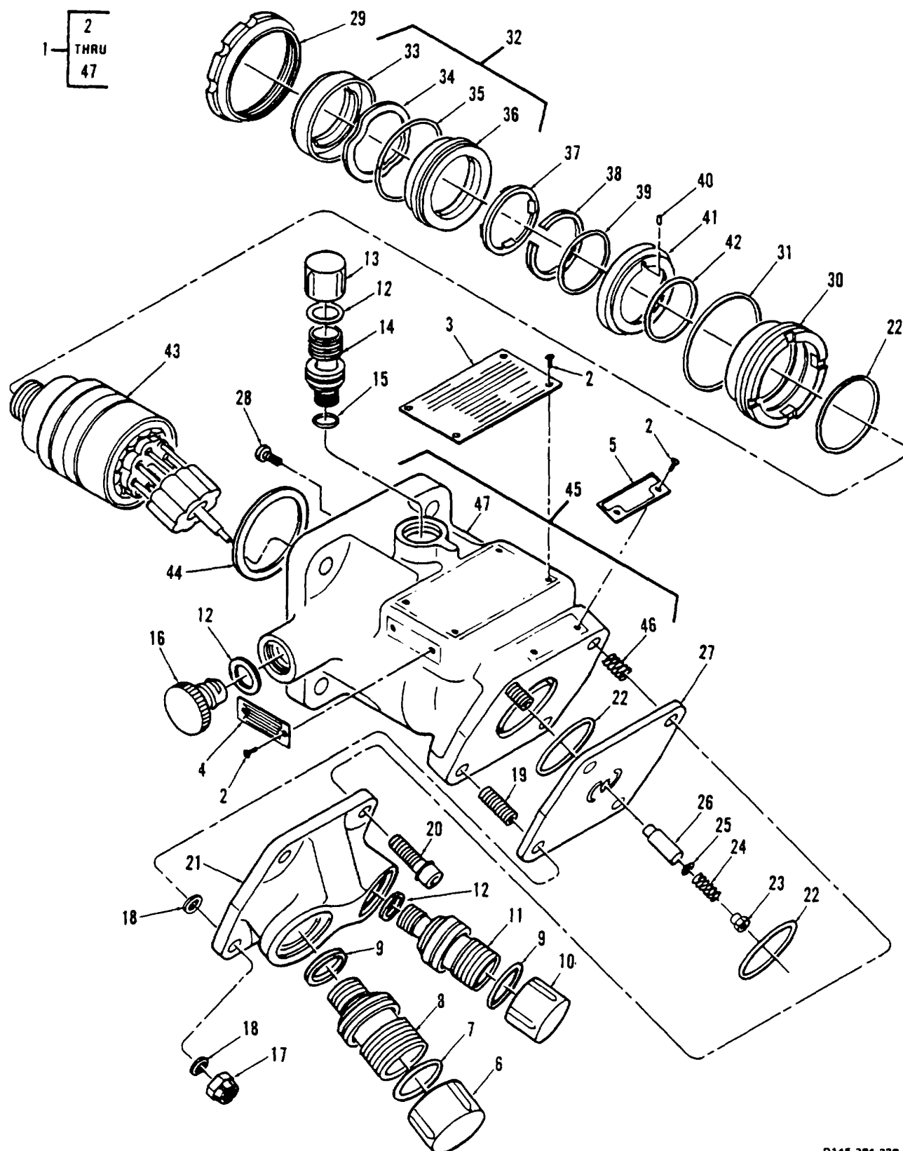
Figure 220. Pump, Axial Piston
