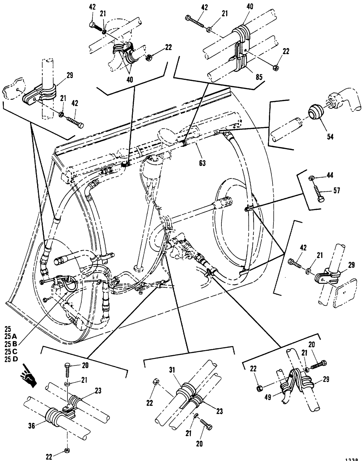
Figure 346. Fuel Cell, Aft Auxiliary (Sheet 5 of 6)
