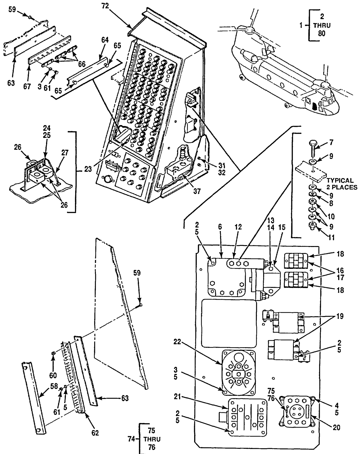
Figure 309A. Panel, Power Distribution, RH (T55-GA-714A Engine) (Sheet 1 of 2)
