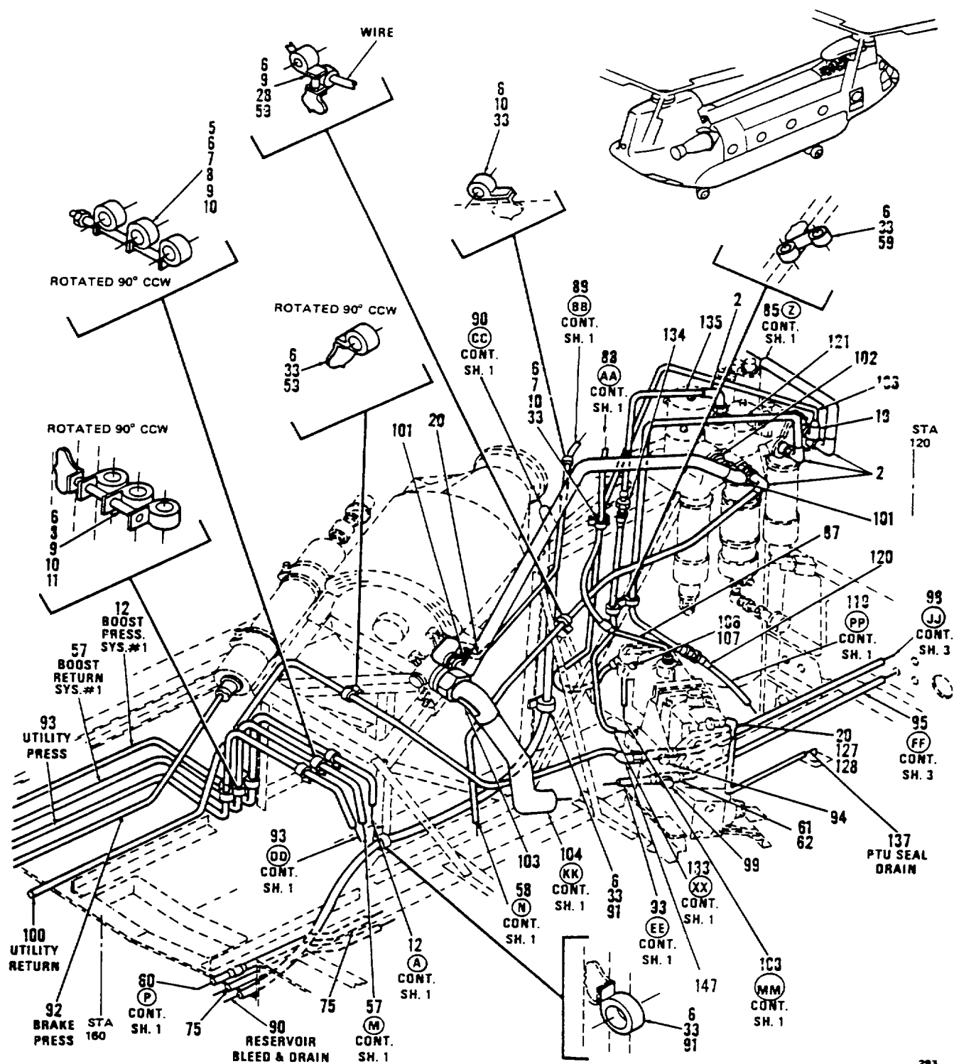
Figure 262. Tubing Instl, Hydraulic, Actuators, Fwd Transmission, Flight Controls Compartment, and Fwd Pylon (Sheet 2 of 6)
