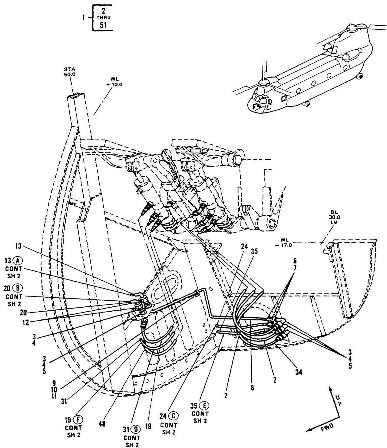
Figure 258. Tubing Instl, Hydraulic, Nose Compartment Sta 0 to 52 (Sheet 1 of 3)
