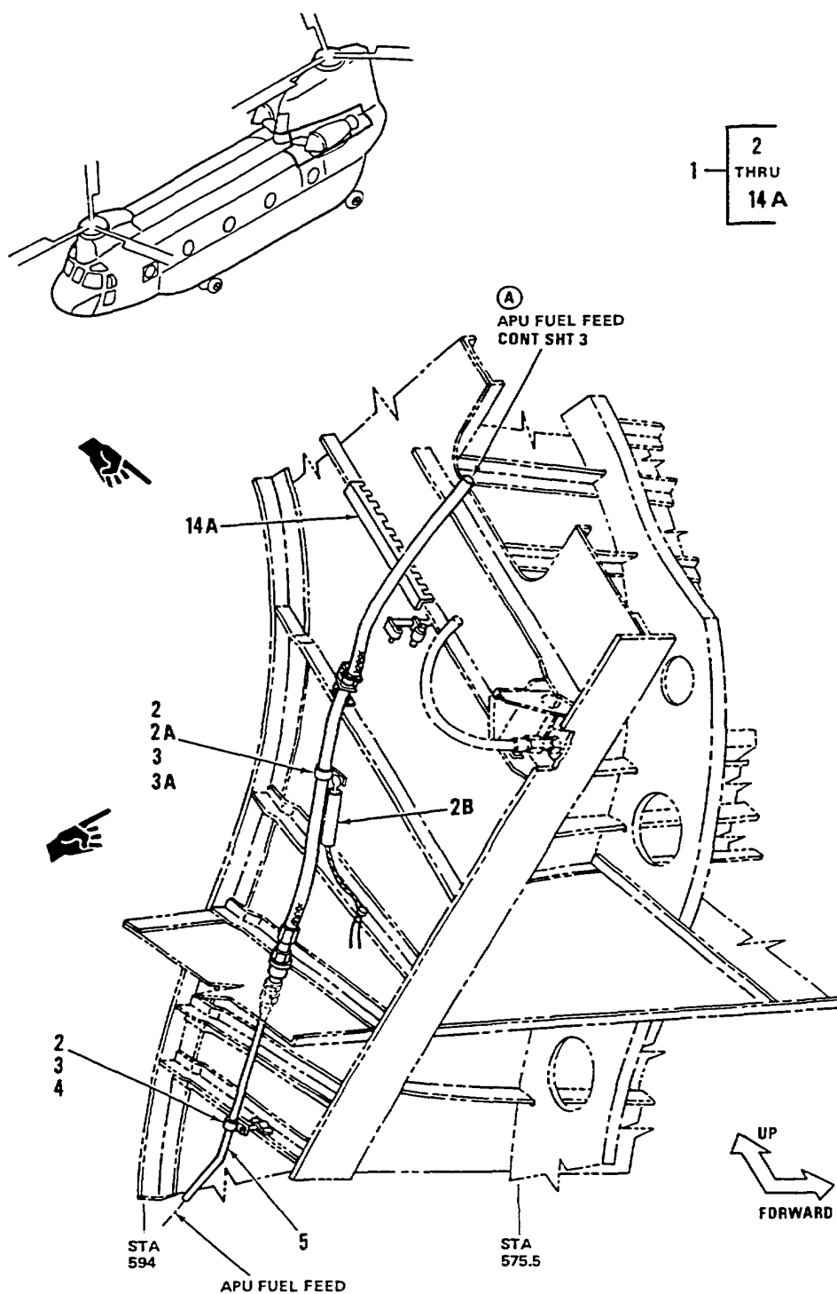
Figure 358. Tubing Instl, Powerplant (Sheet 1 of 3)
