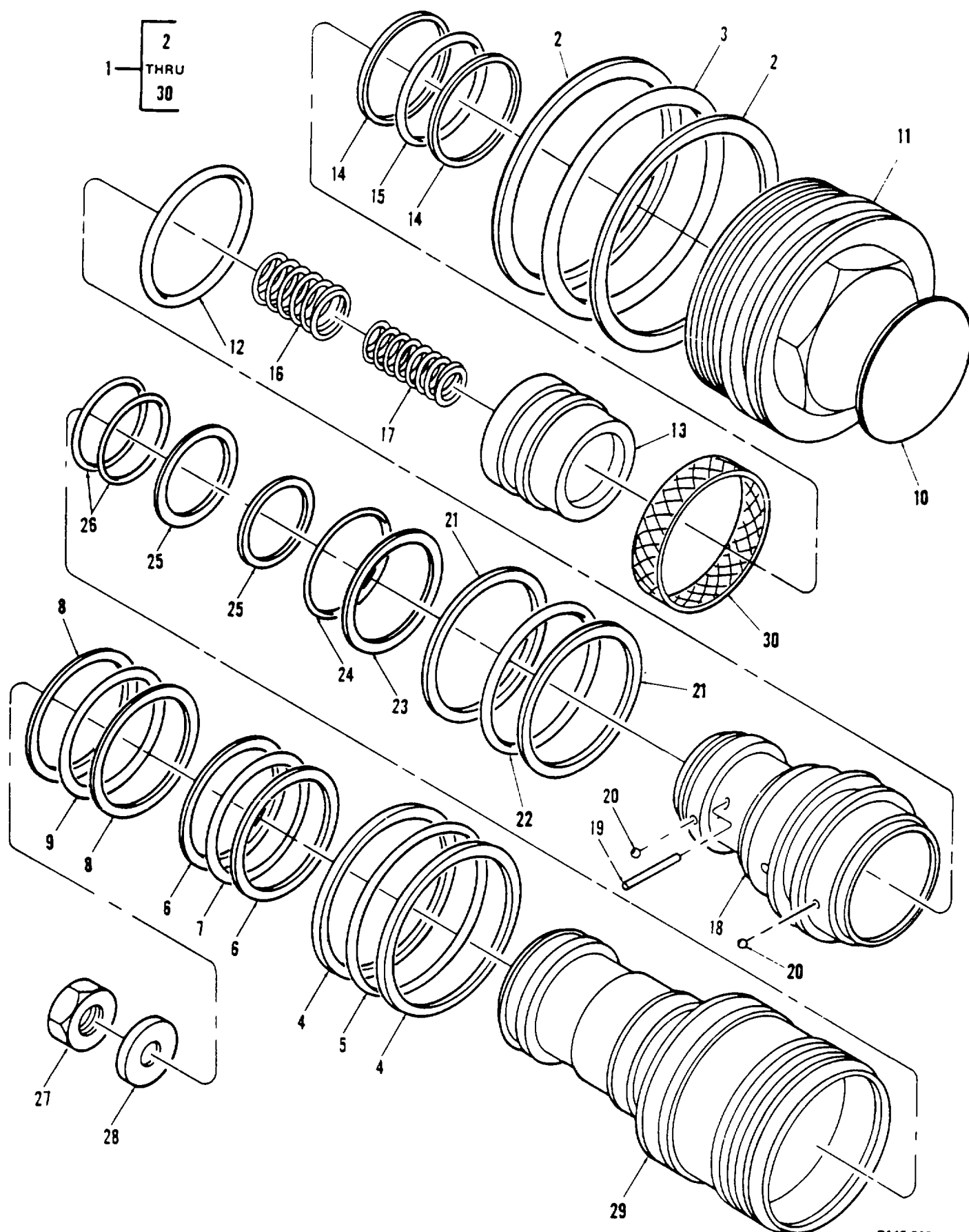
Figure 233. Valve, Engine and APU M1750-01
