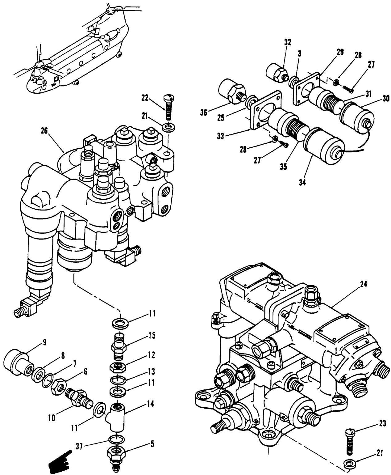
Figure 206. Equipment Instl, Sta 120 to 160 (Sheet 2 of 2)
