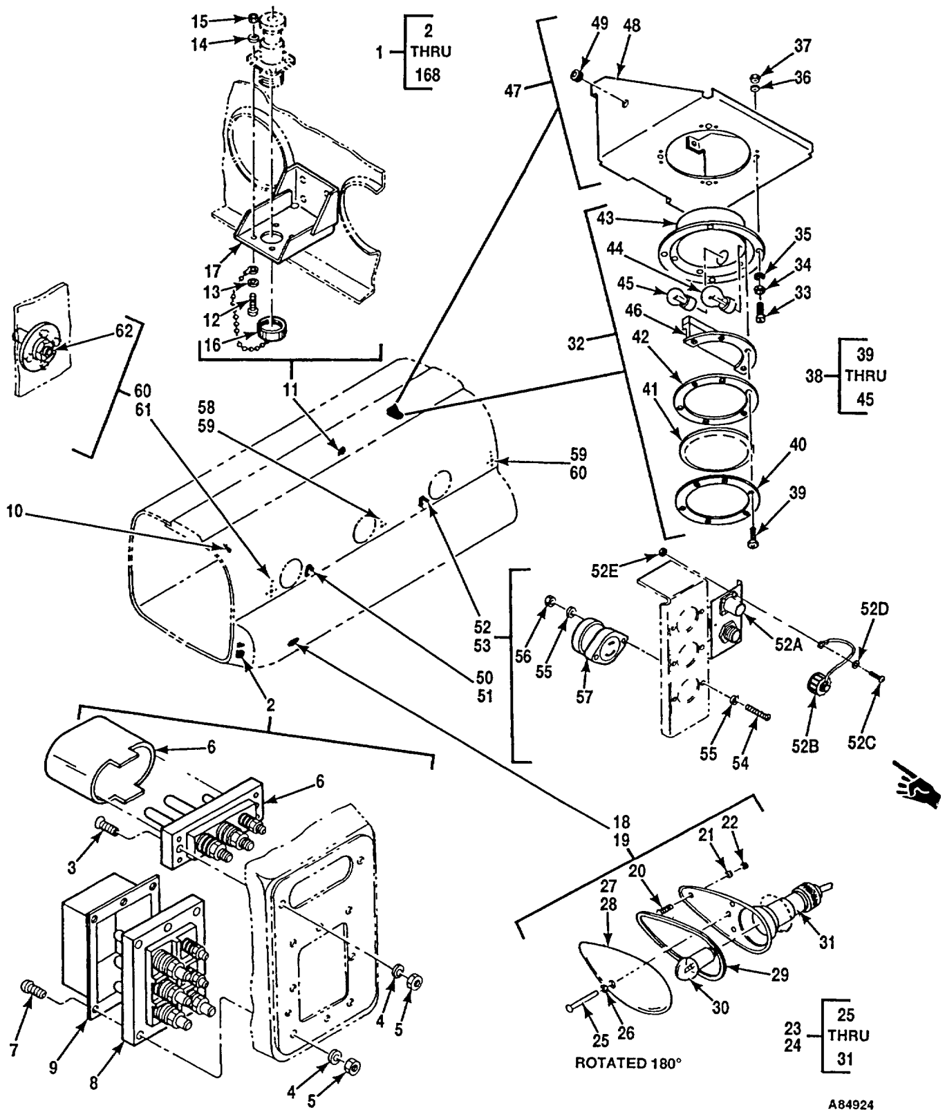
Figure 323. Equipment Instl, Cabin (Sheet 1 of 4)
