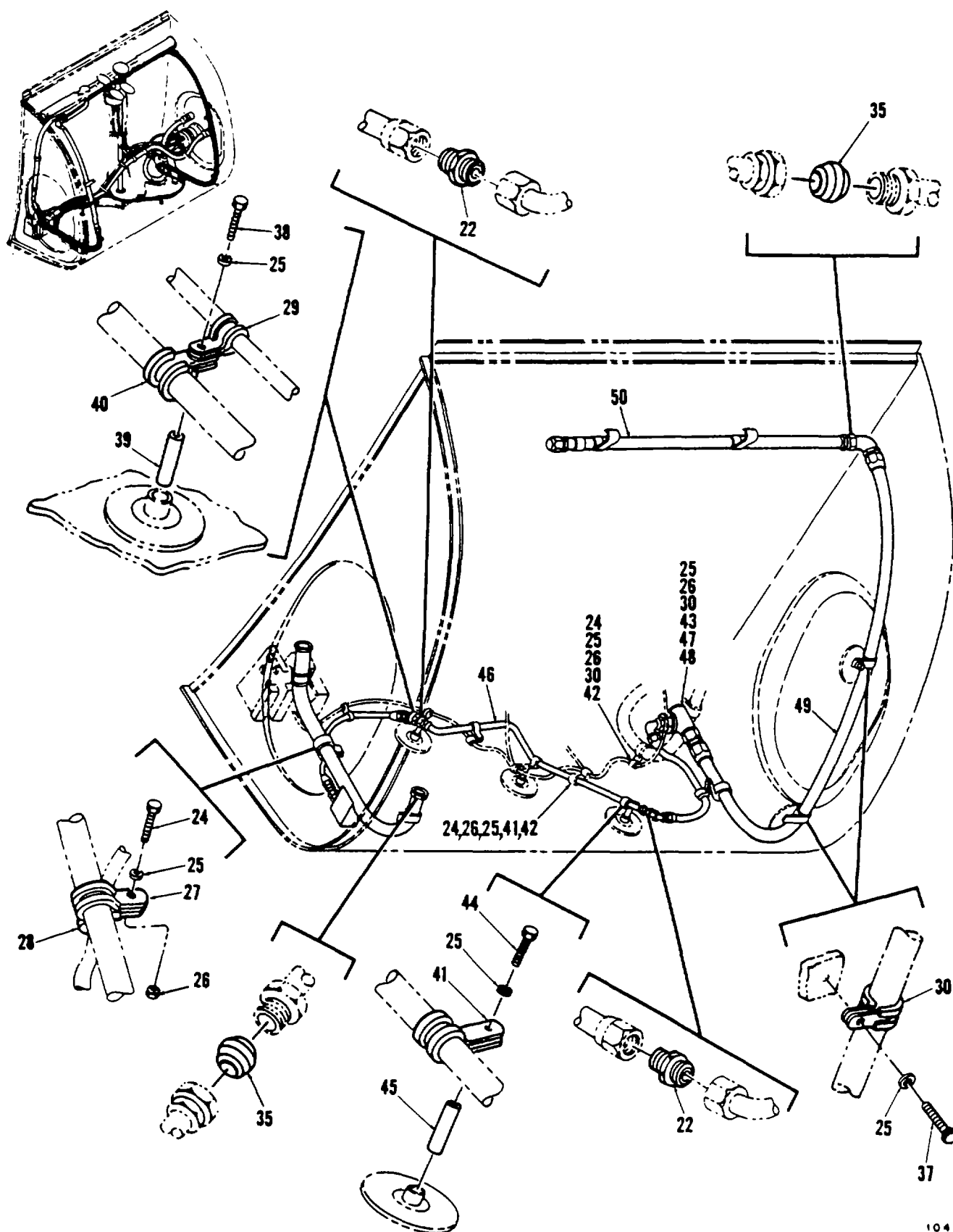
Figure 340. Fuel Cell, Fwd Auxiliary (Sheet 3 of 9)
