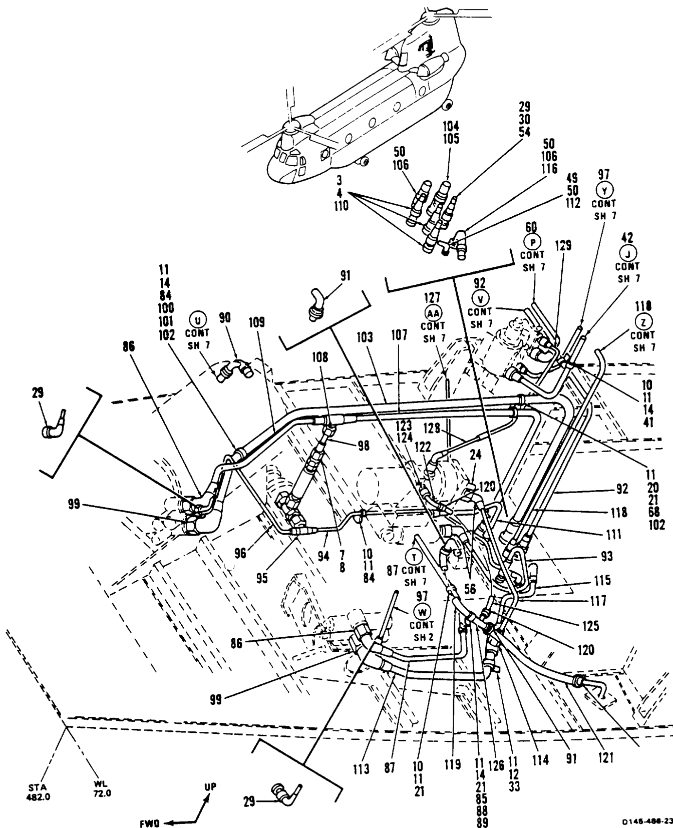
Figure 273. Tubing Instl, Aft Pylon and Combining Transmission Area (Sheet 6 of 7)
