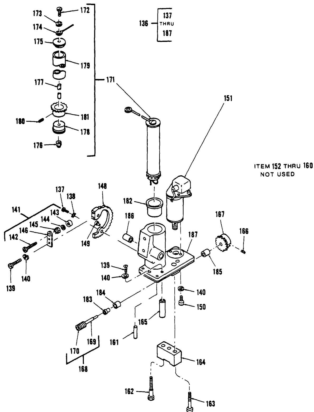
Figure 311. Light Instl, Landing and Search (Sheet 4 of 5)
