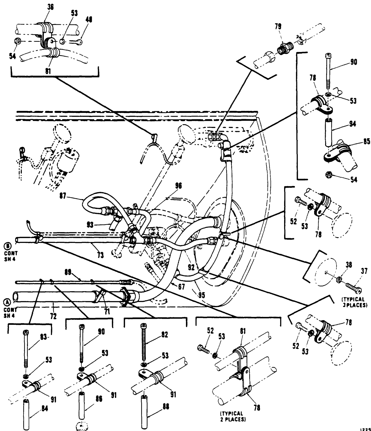
Figure 345. Fuel Cell, Main (Sheet 5 of 8)
