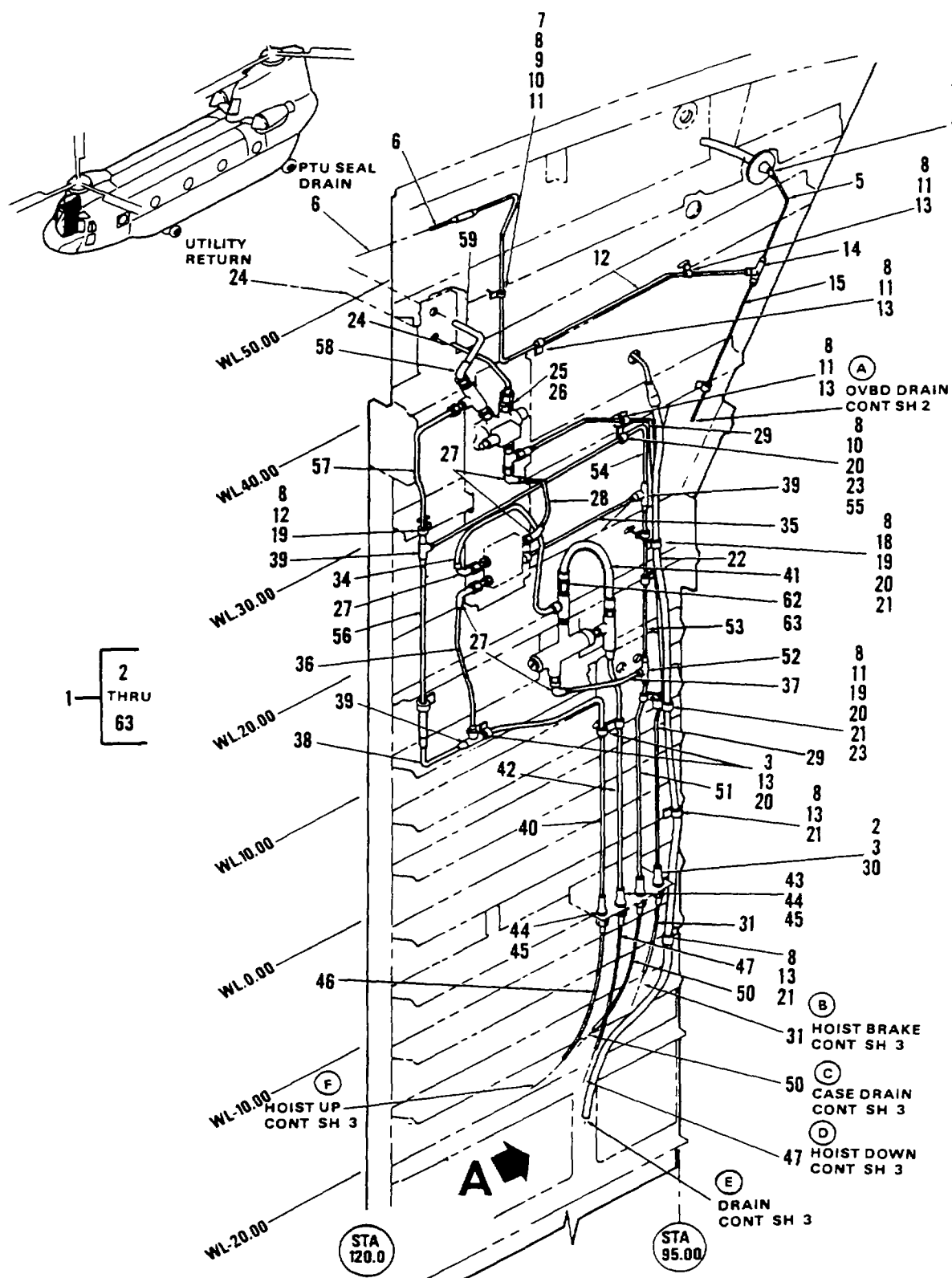
Figure 260. Tubing Instl, Hydraulic, Heater Compartment, RH Sta 95 to 120 (Sheet 1 of 3)
