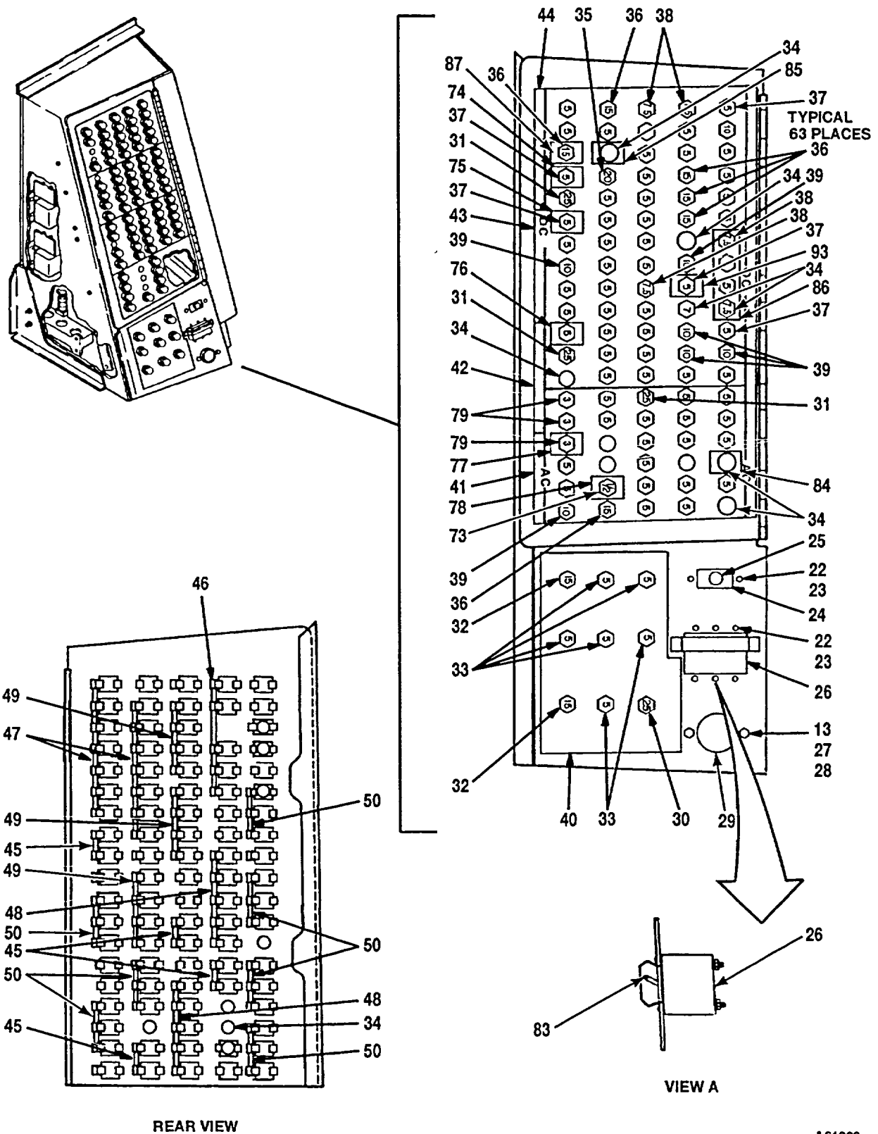
Figure 307A. Panel, Power Distribution, LH (T55-GA-714A Engine) (Sheet 2 of 2)
