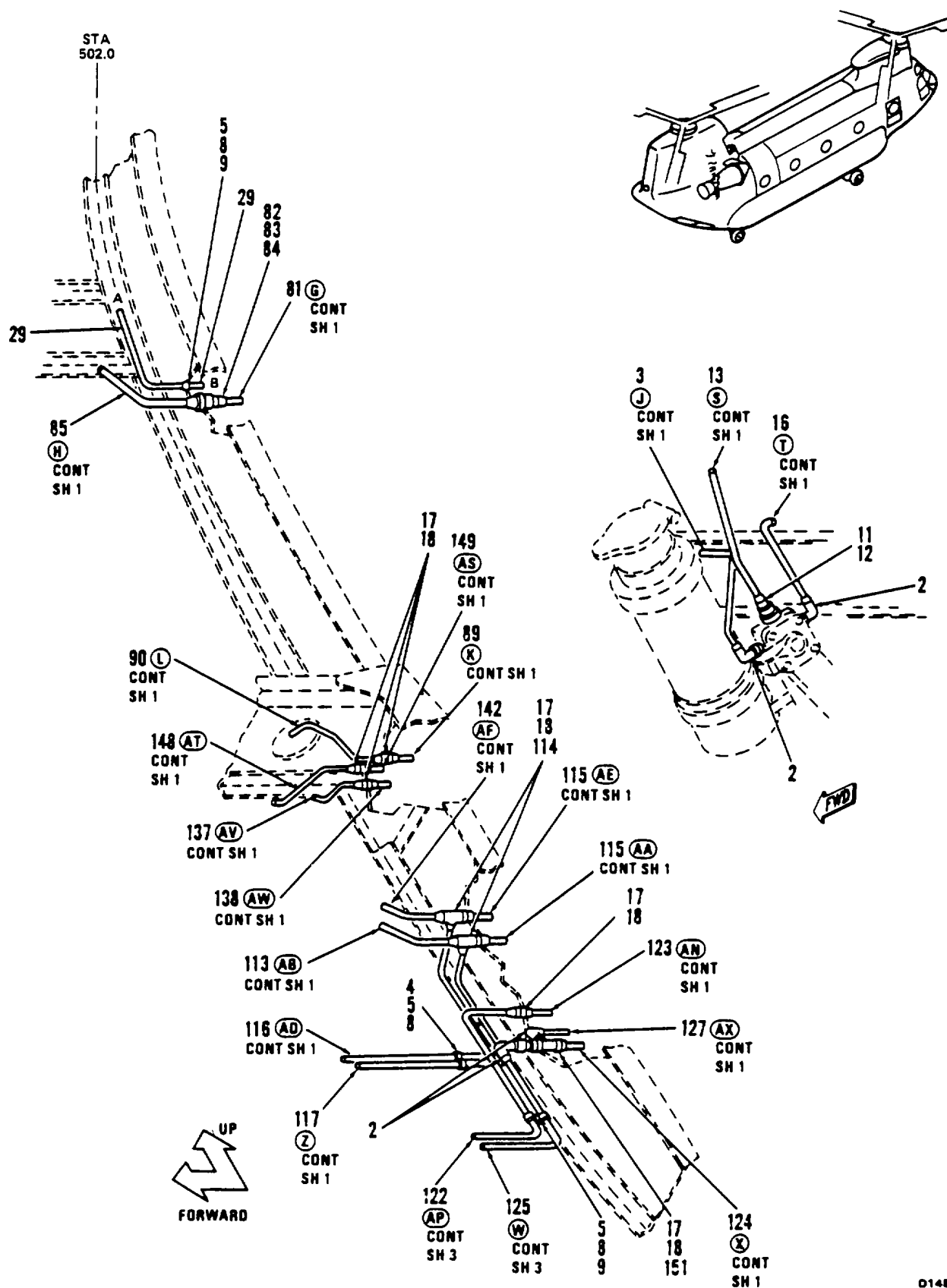
Figure 268. Tubing Instl, Hydraulic, Aft Fuselage, Lower, RH Sta 440 to 594 (Sheet 2 of 5)
