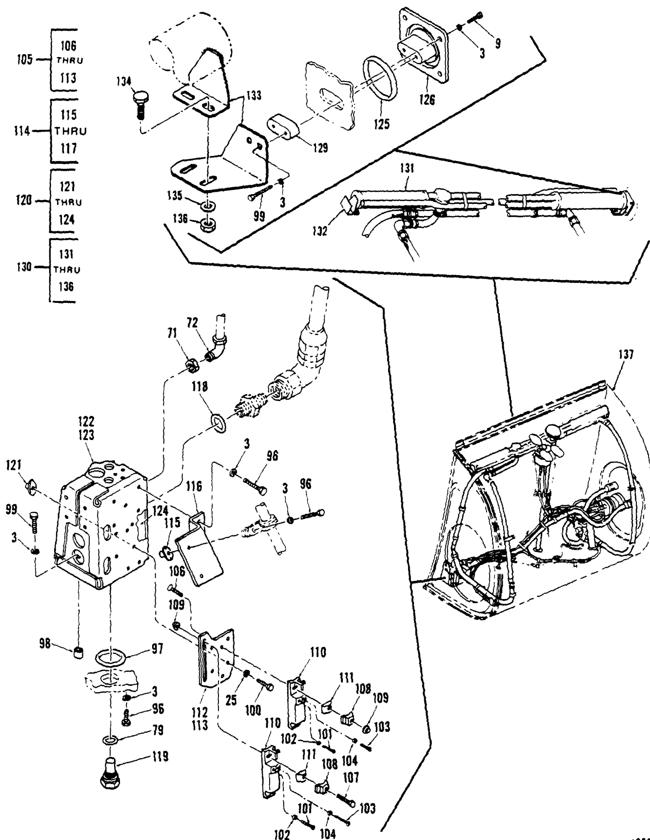
Figure 340. Fuel Cell, Fwd Auxiliary (Sheet 9 of 9)
