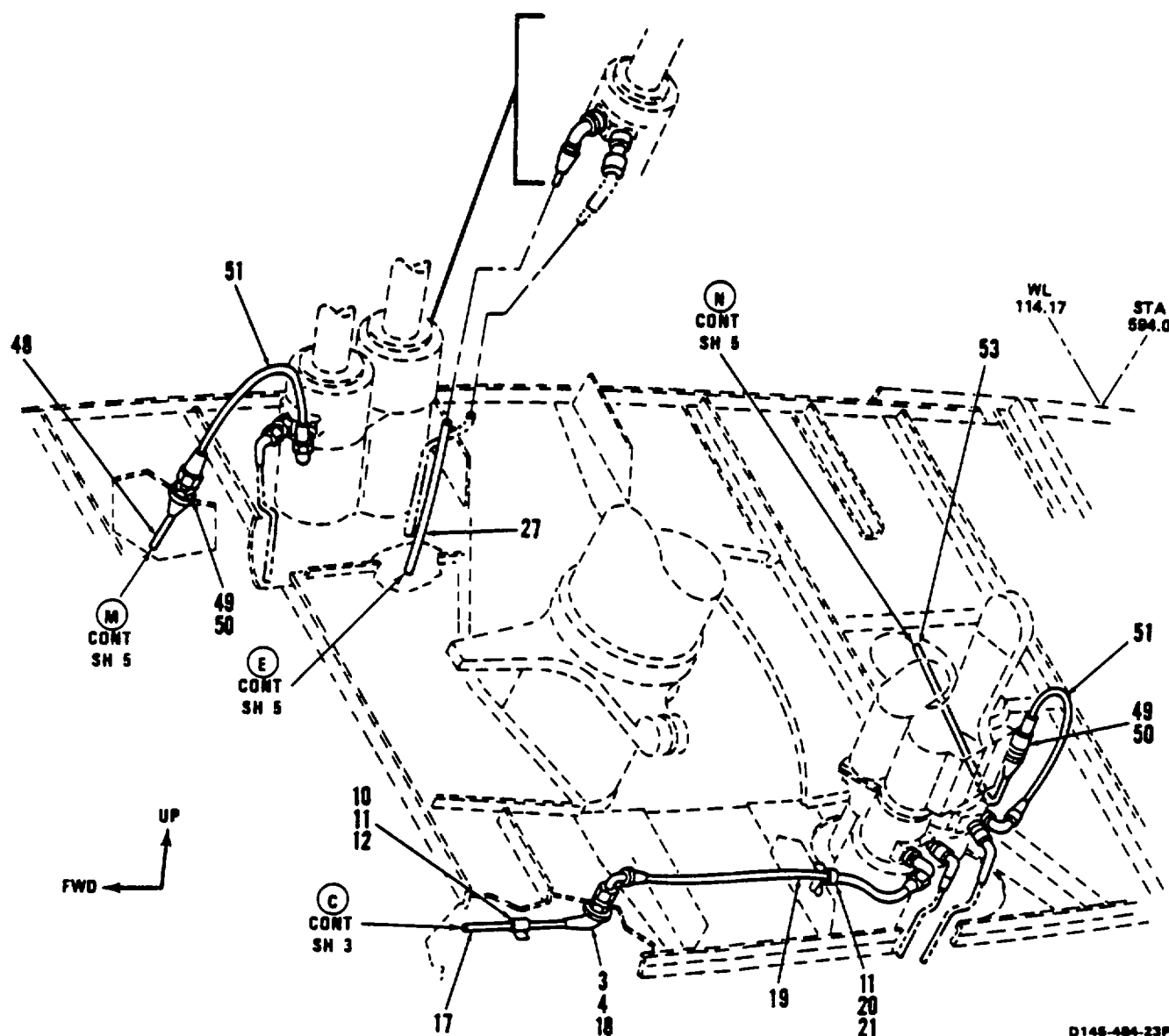
Figure 273. Tubing Instl, Aft Pylon and Combining Transmission Area (Sheet 4 of 7)
