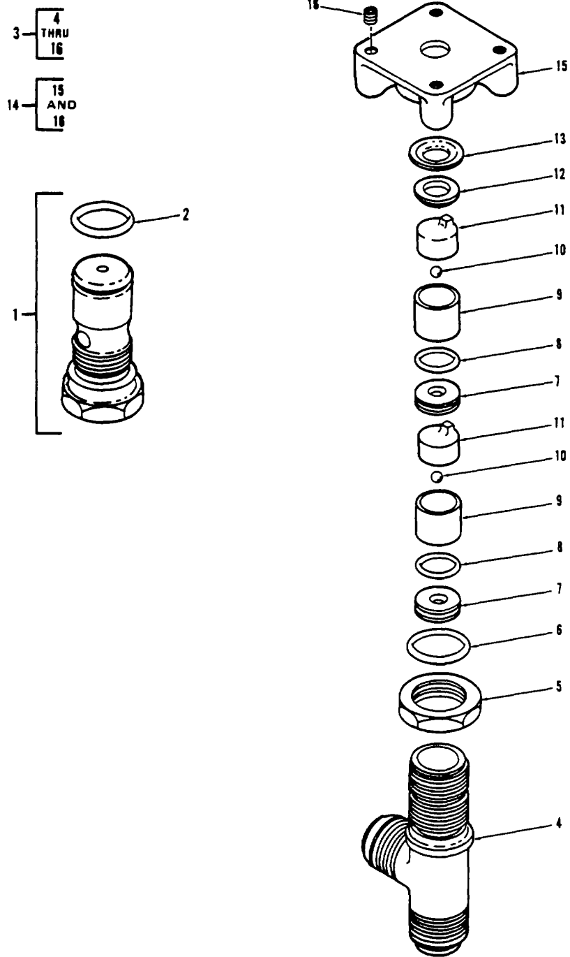
Figure 343. Valve, Drain
