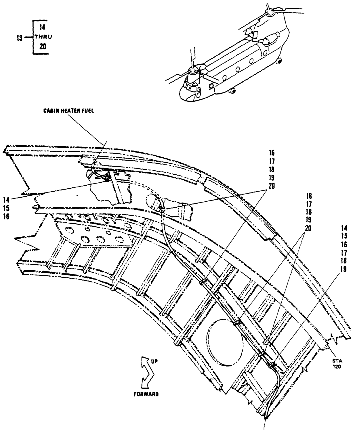
Figure 353. Tubing Instl, Crown, Sta 120 to 160, LH Heater Compartment, Sta 95 to 120, RH (Sheet 2 of 2)
