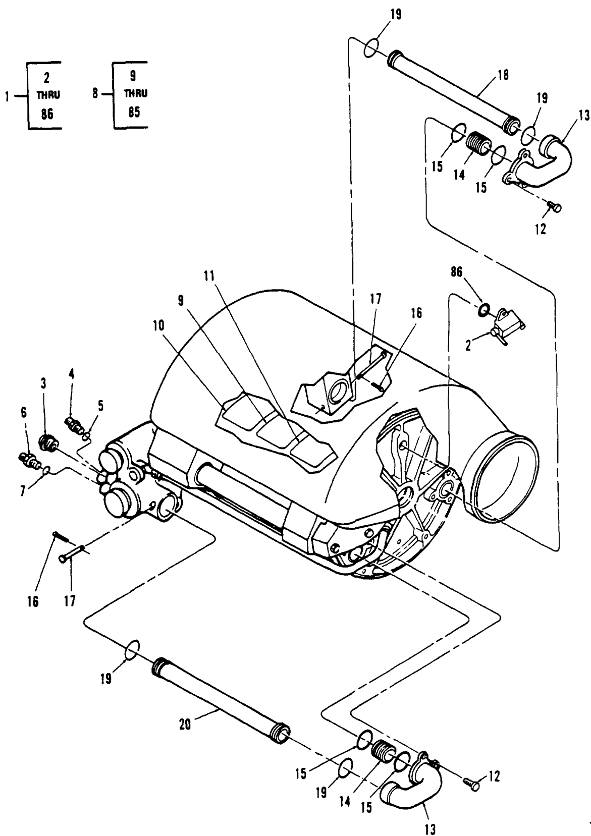
Figure 216. Reservoir/Cooler 1711018-002 (Sheet 1 of 3)
