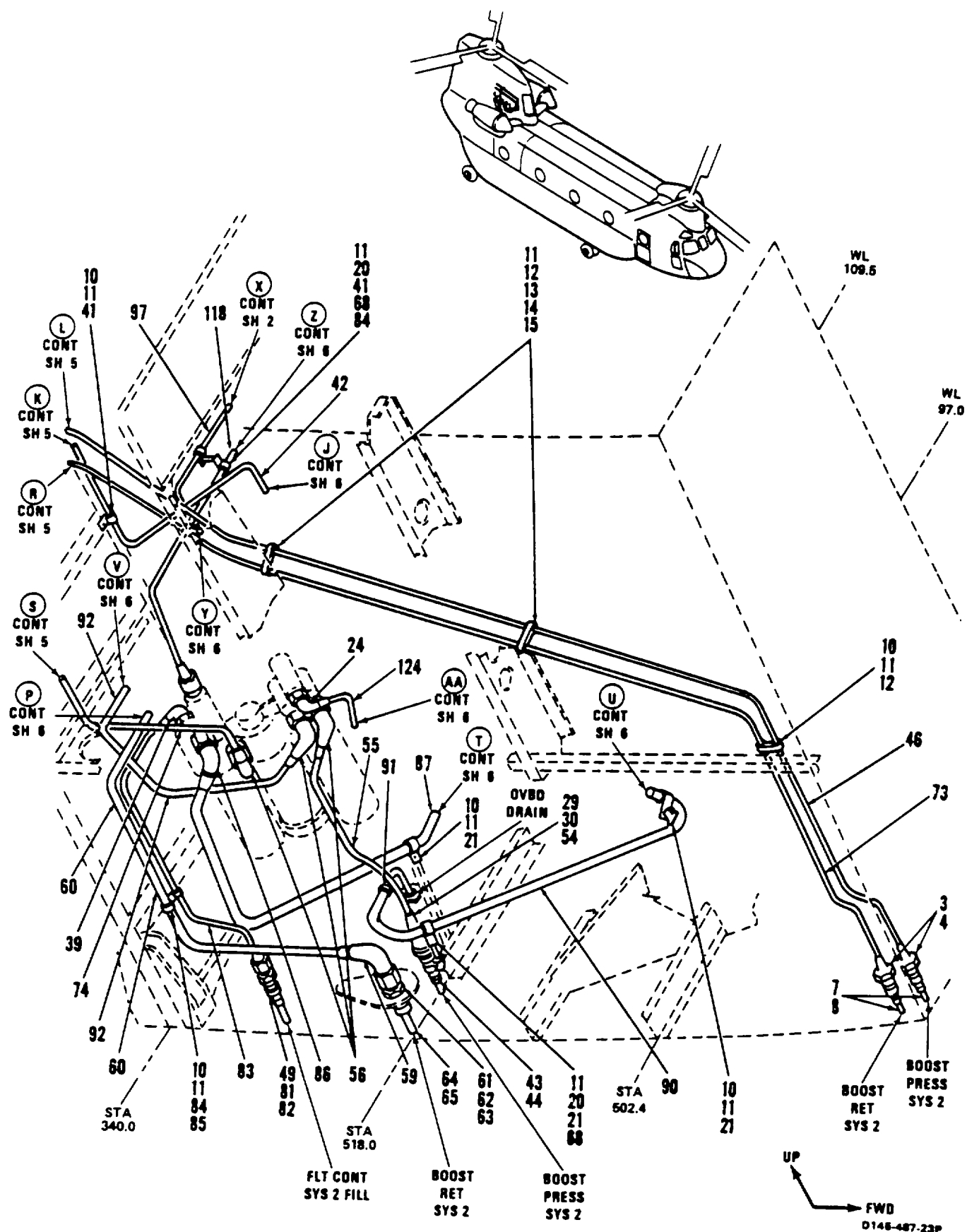
Figure 273. Tubing Instl, Aft Pylon and Combining Transmission Area (Sheet 7 of 7)
