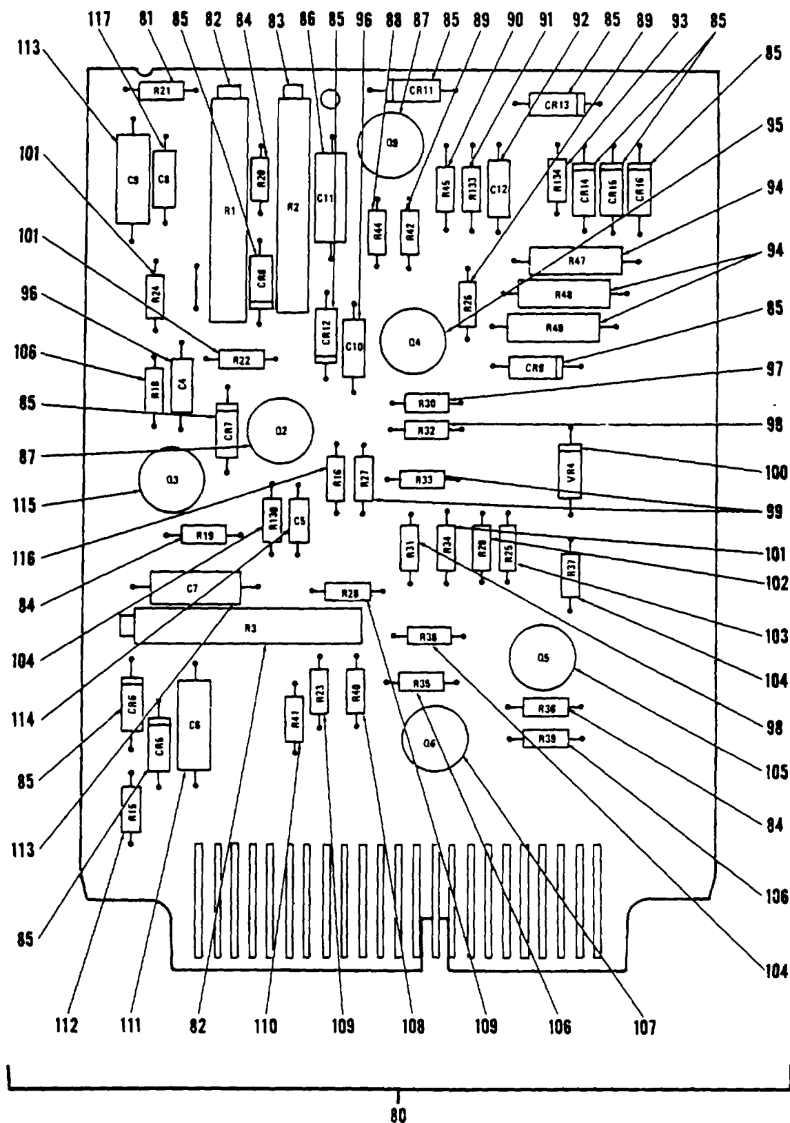
Figure 322. Panel, Generator Control (Sheet 2 of 5)
