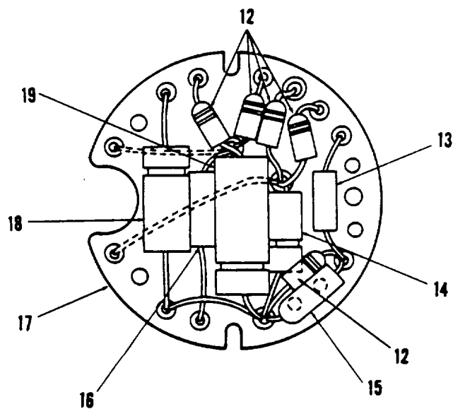
11 COMPONENT ASSEMBLY 392801
