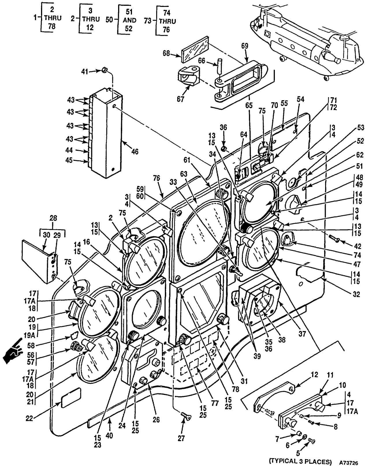
Figure 275. Panel, Instrument, Copilots
