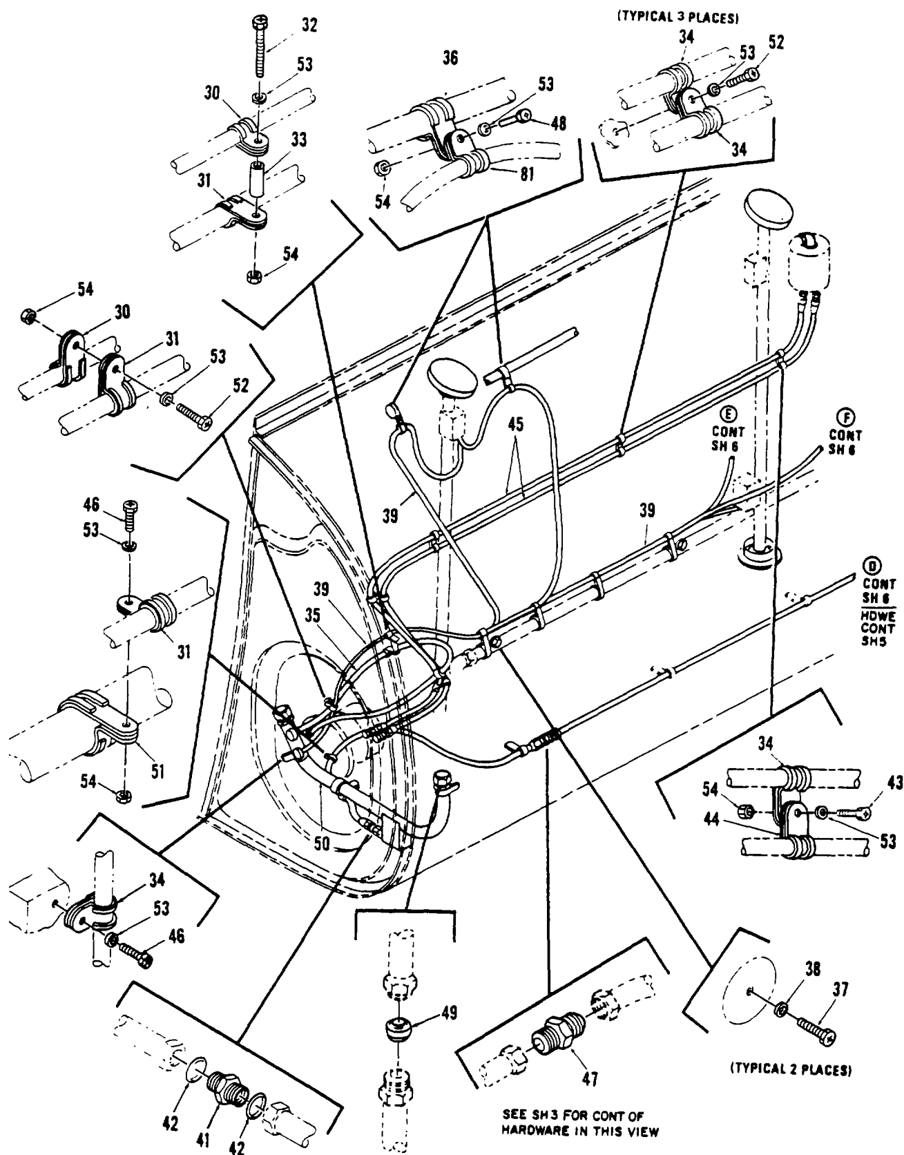
Figure 345. Fuel Cell, Main (Sheet 2 of 8)
