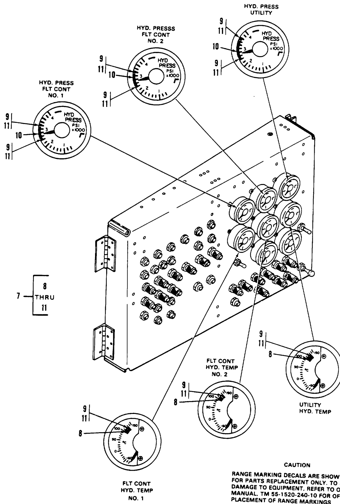
Figure 292. Range Markings, Instrument (Sheet 2 of 2)
