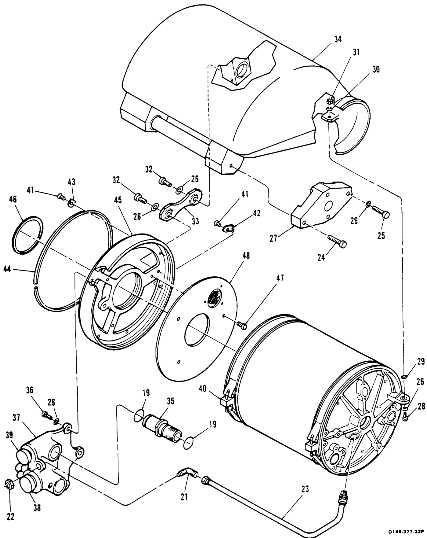
Figure 216. Reservoir/Cooler 1711018-002 (Sheet 2 of 3)
