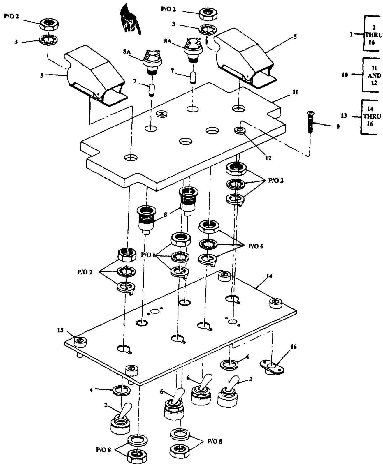
Figure 302. Panel, Engine Trim
