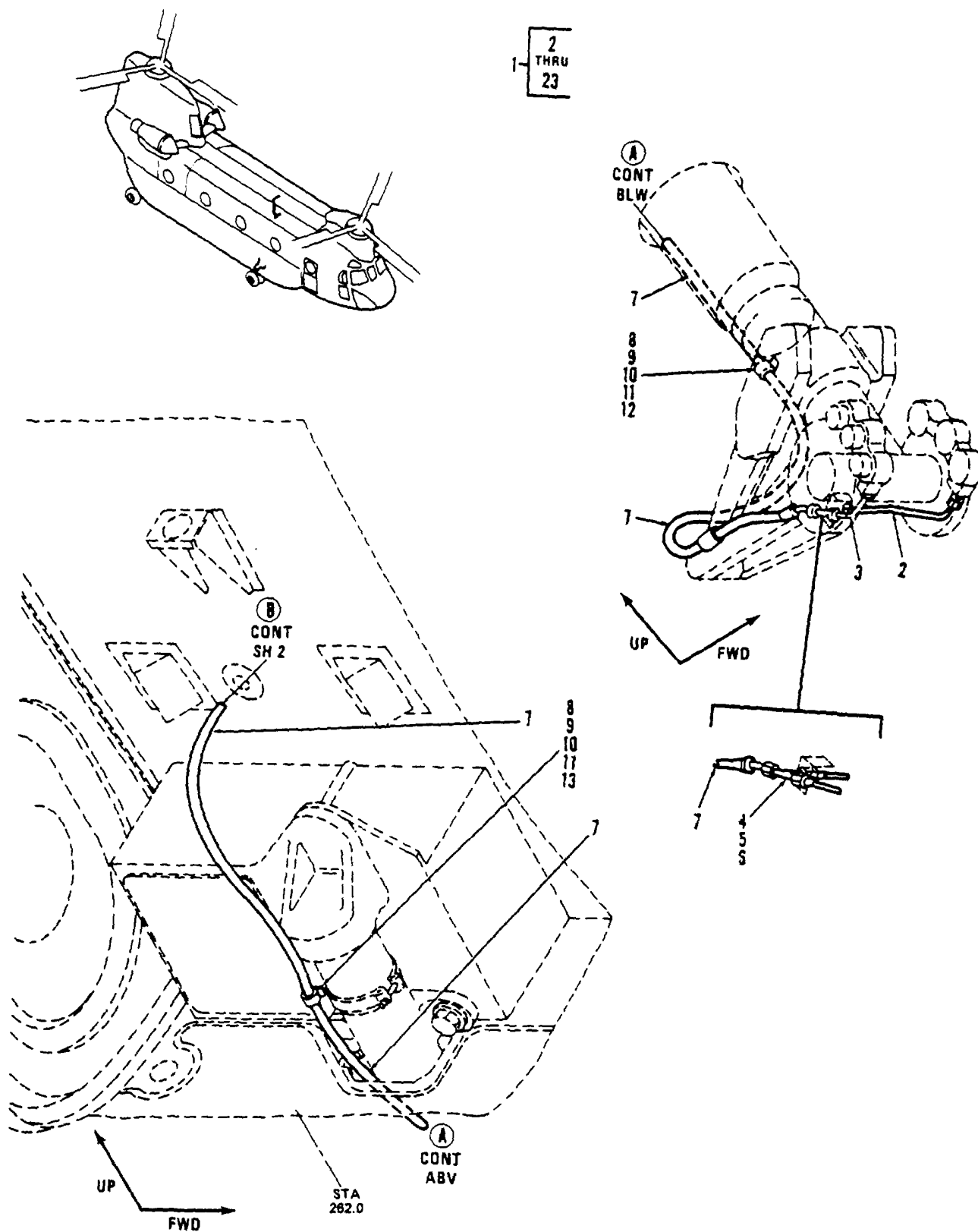
Figure 264. Tubing Instl, Hydraulic, Cabin Ceiling and Side, Lower, LH, Sta 160 to 440 (Sheet 1 of 2)
