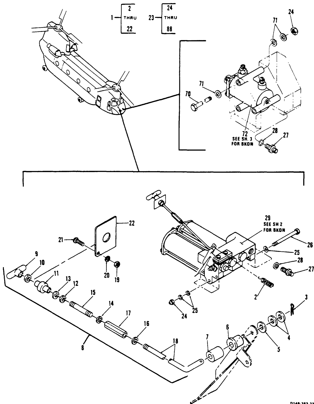
Figure 201. Control Instl, Wheel Brake (Sheet 1 of 3)
