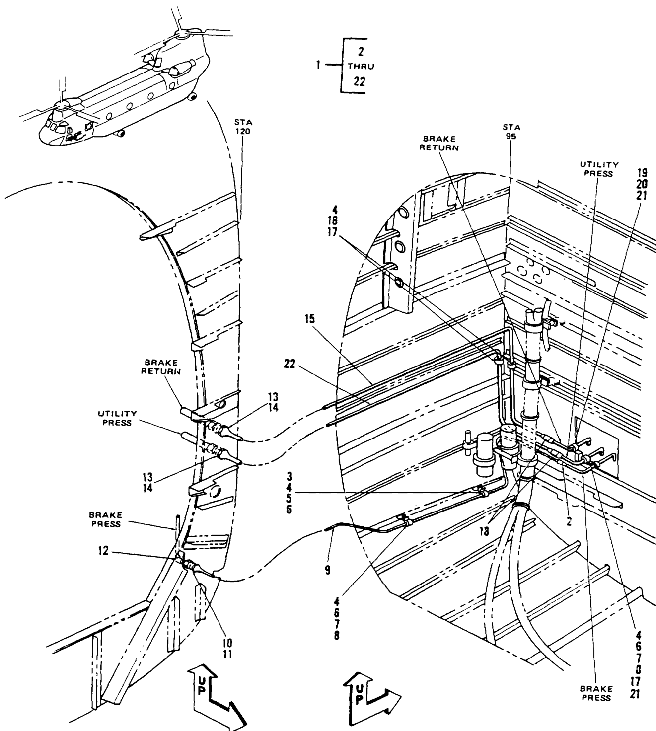
Figure 261. Tubing Instl, Hydraulic, Electronics and Flight Compartment, LH, Sta 95-120
