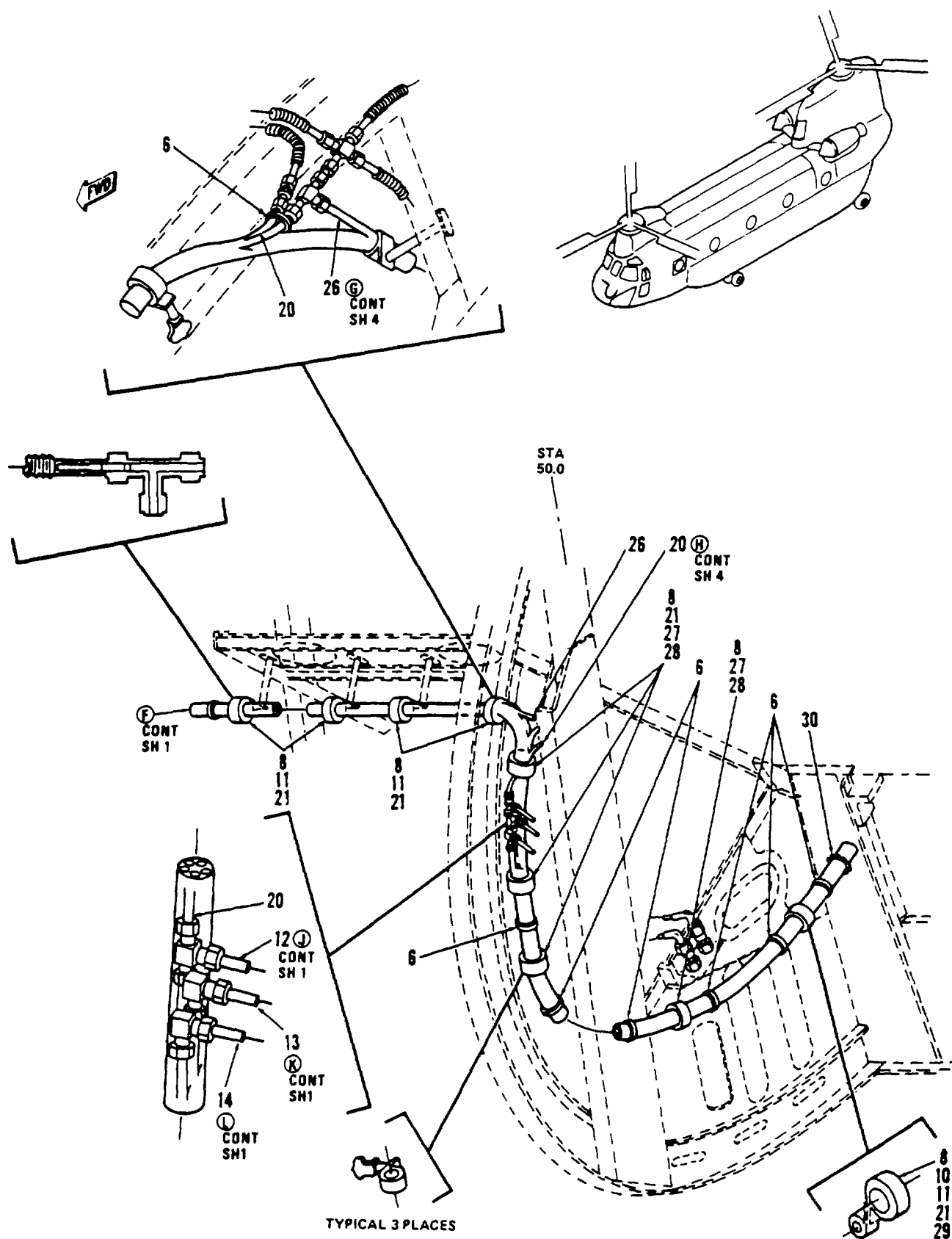
Figure 294. Tubing Instl equipment, Nose Compartment (Sheet 2 of 4)
