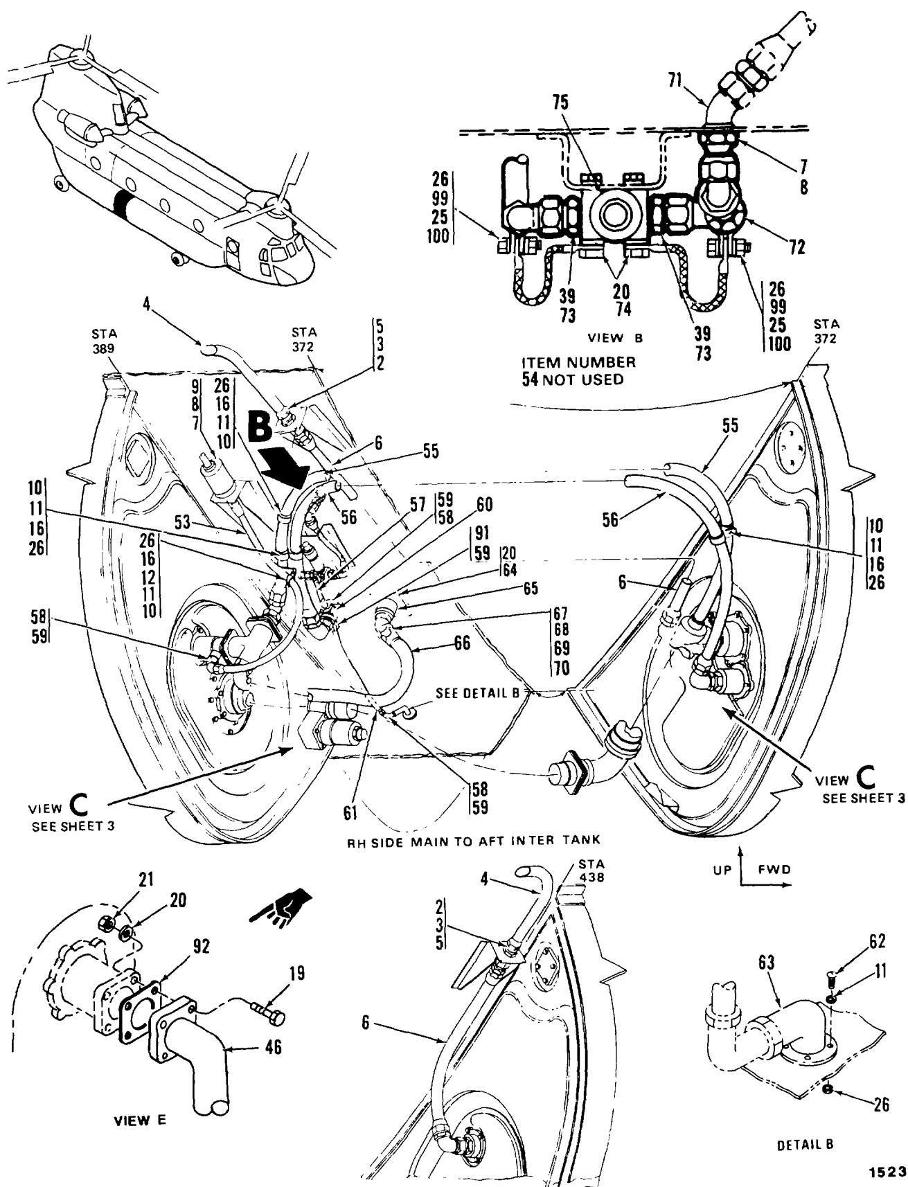
Figure 348. Intertank Connection Instl, RH (Sheet 2 of 5)
