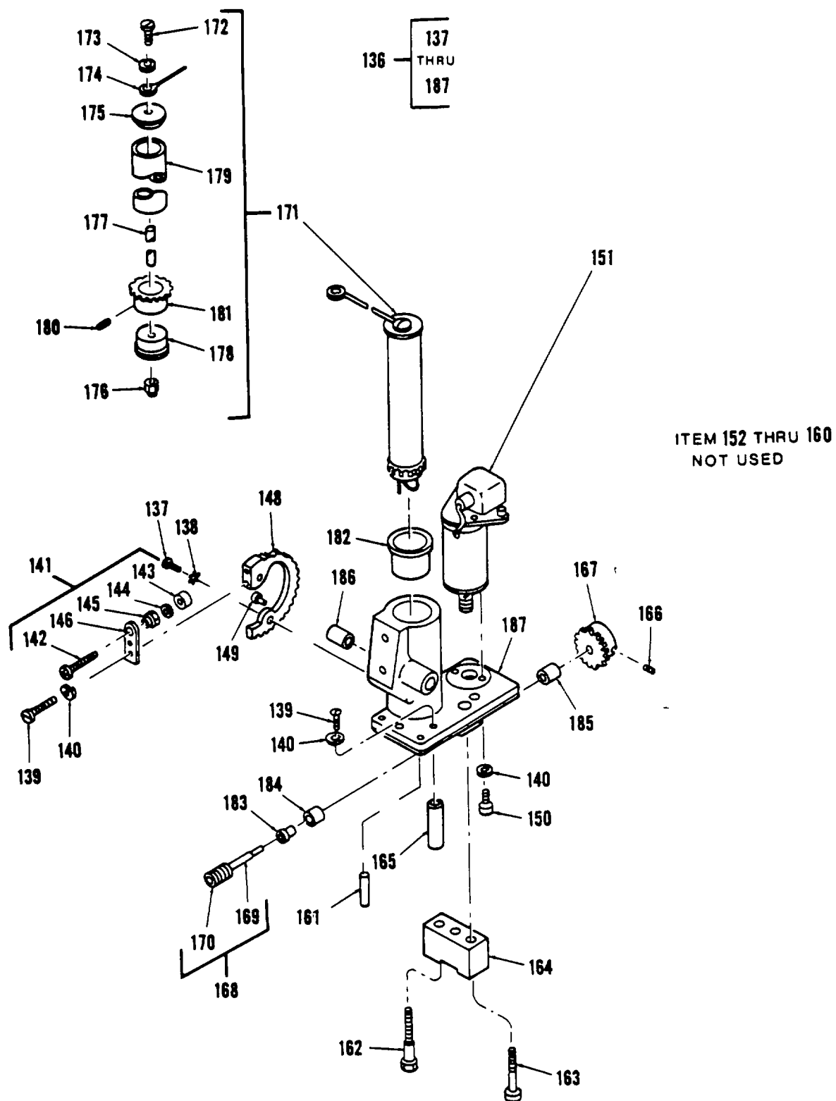
Figure 311. Light Instl, Landing and Search (Sheet 4 of 5)
