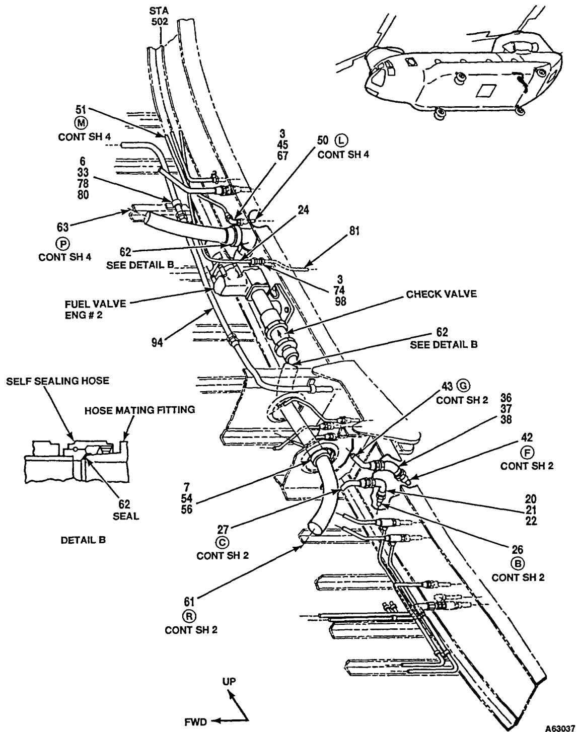
Figure 357. Tubing Instl, Aft Fuselage (Sheet 3 of 5)
