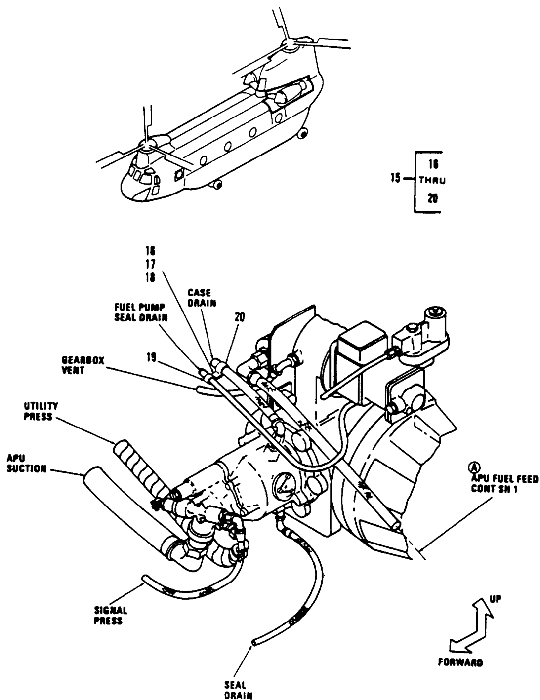
Figure 358. Tubing Instl, Powerplant (Sheet 3 of 3)
