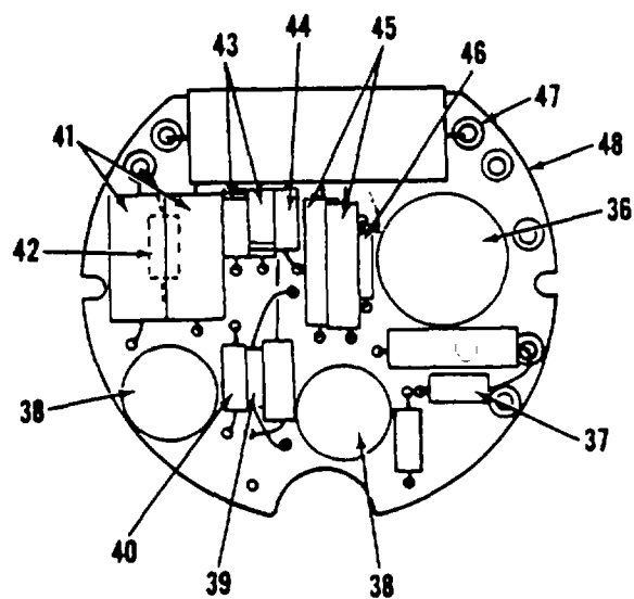
35 AMPLIFIER ASSY. 397967-03019
