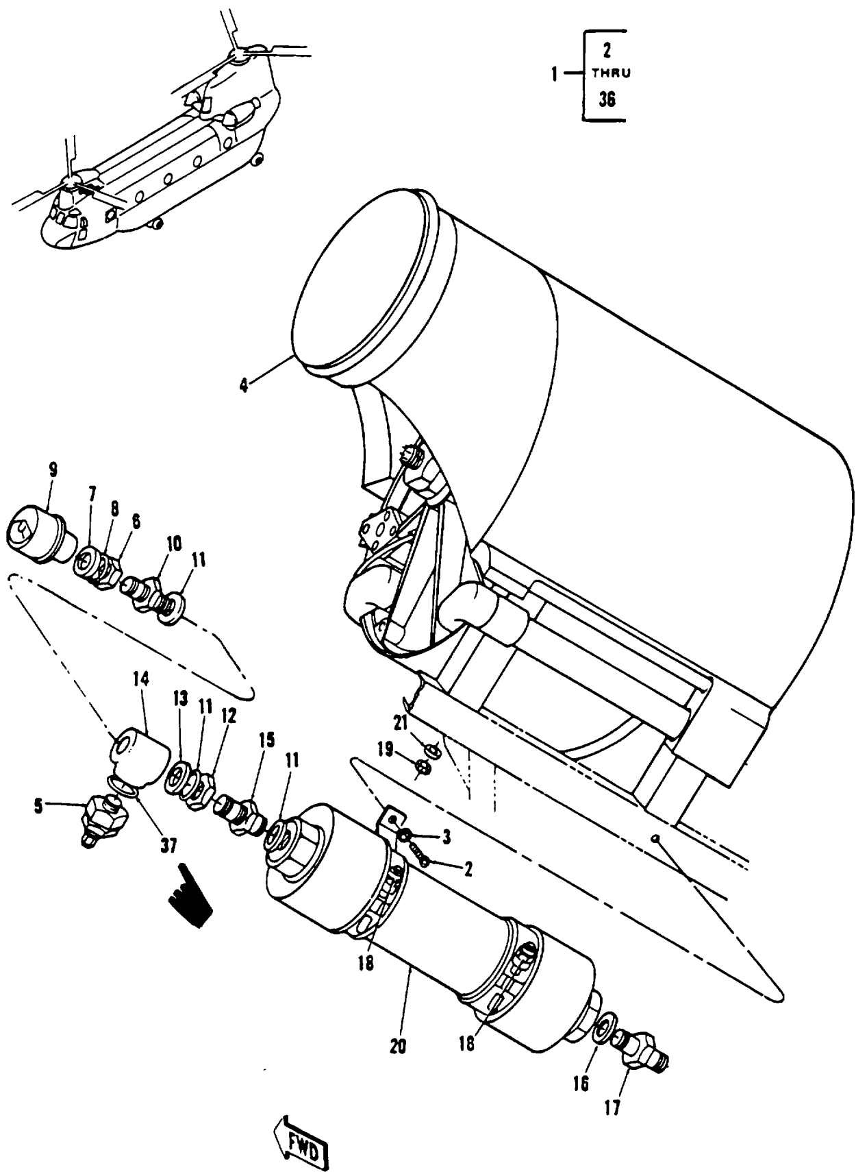
Figure 206 Equipment Instl, Sta 120 to 160 (Sheet 1 of 2)
