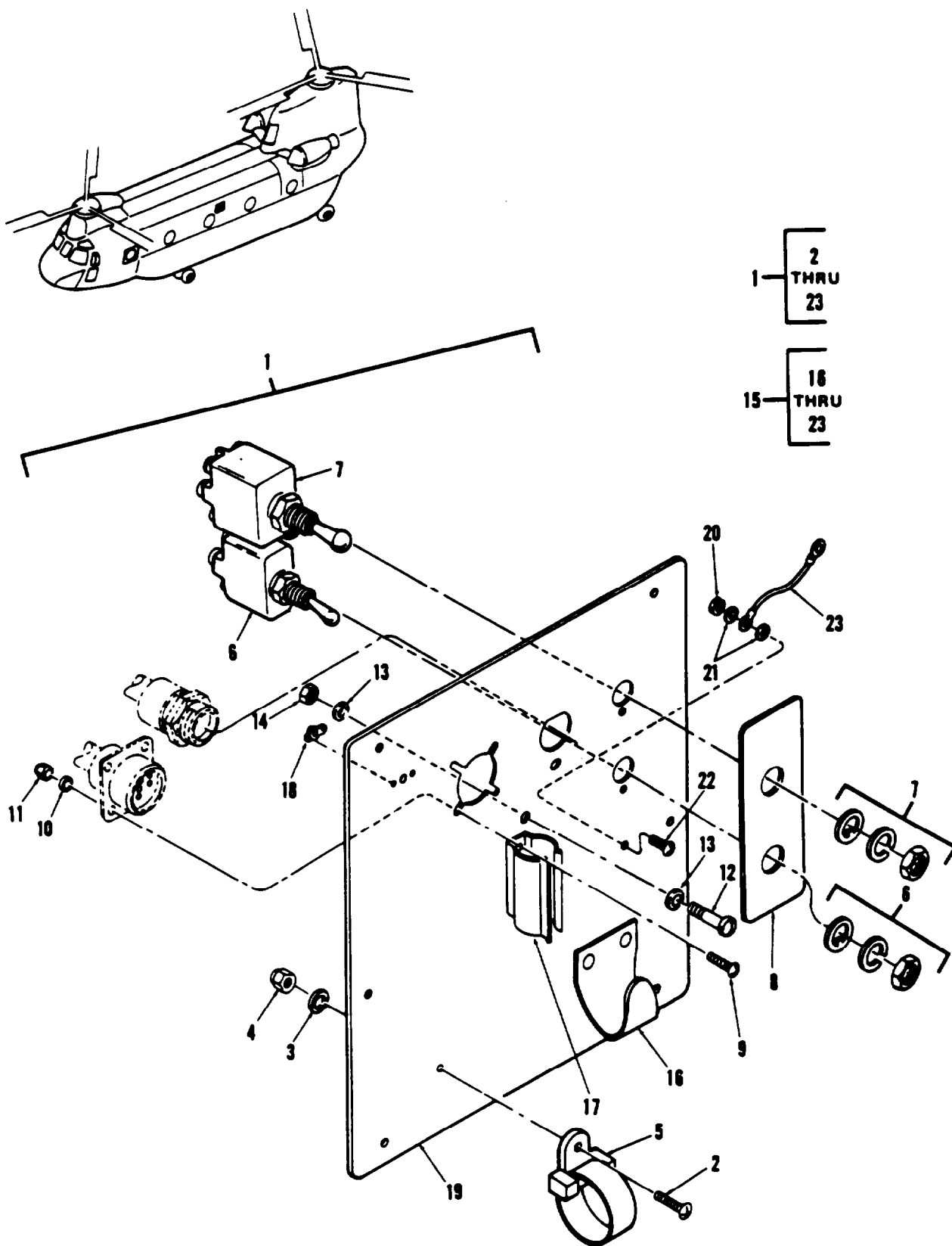
Figure 327. Panel, Hoist Operator
