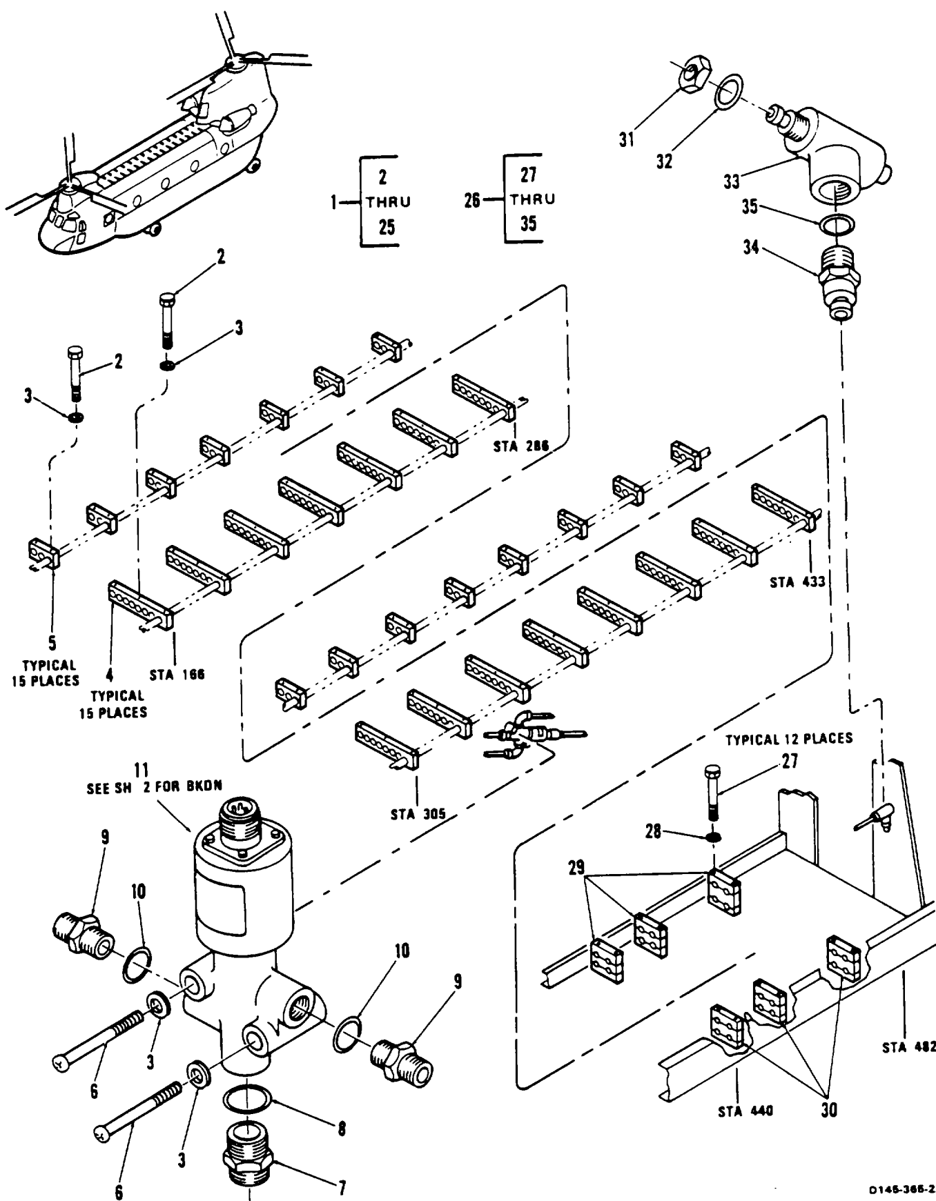
Figure 207. Equipment Instl, Tunnel, Sta 160 to 440 (Sheet 1 of 2)
