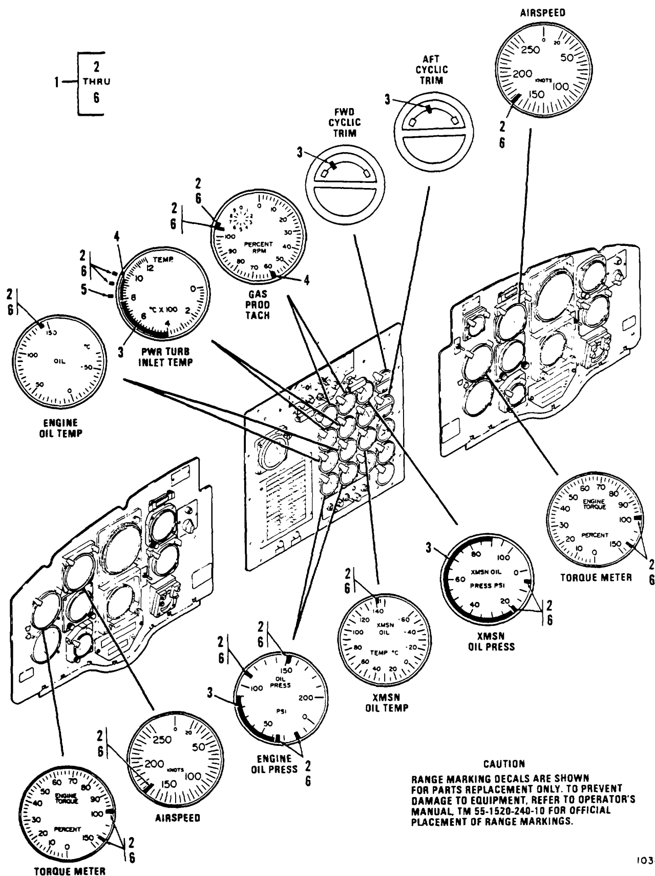
Figure 292. Range Markings, Instrument (Sheet 1 of 2)
