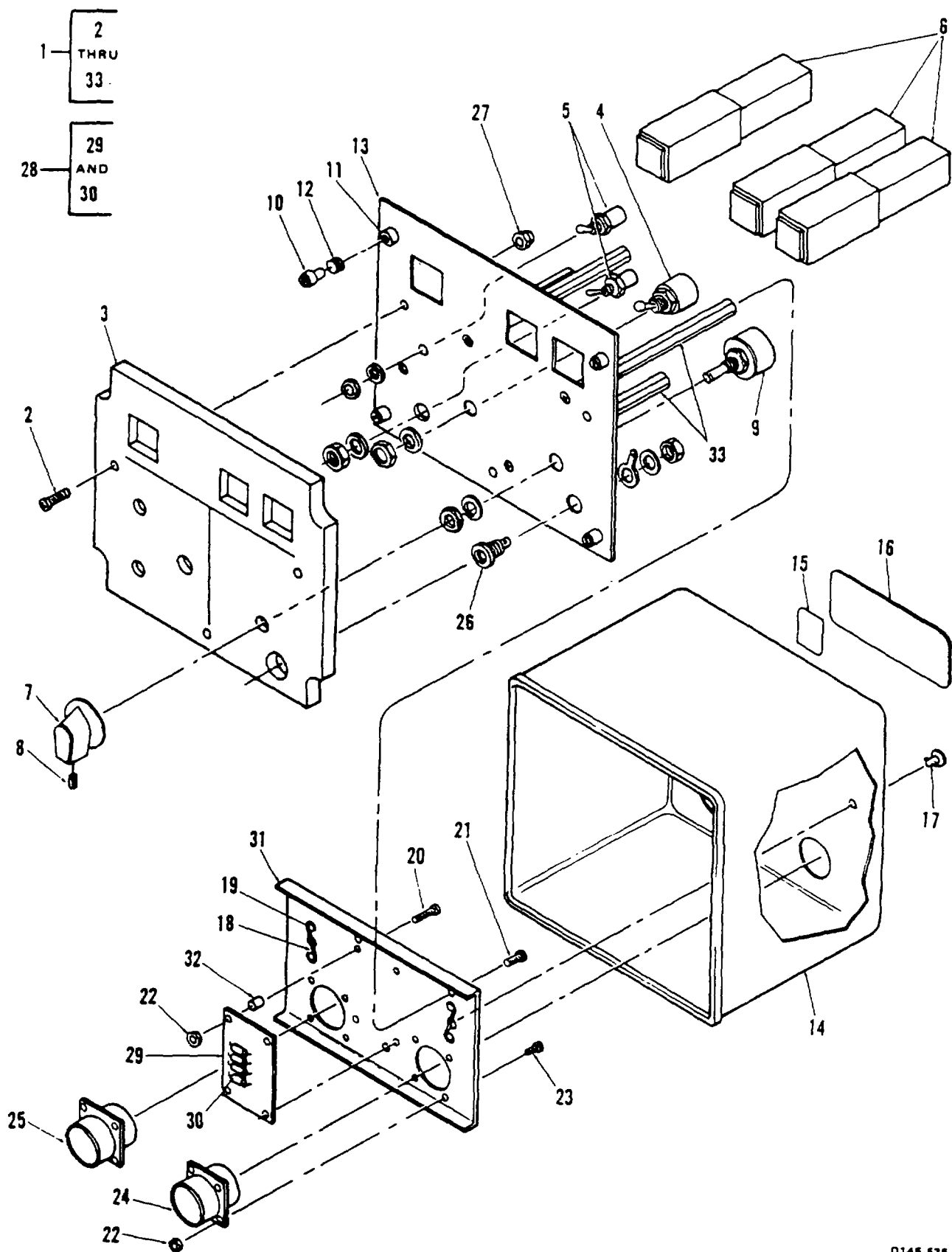
Figure 300. Panel AFCS
