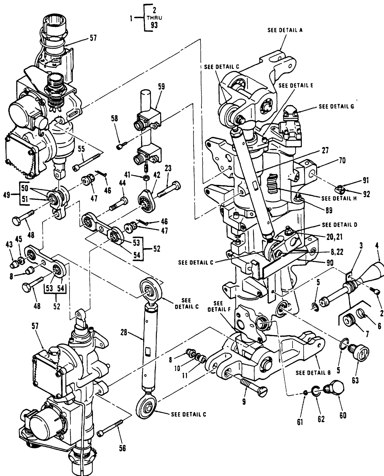
Figure 245. Actuator, Pitch Axis (Sheet 1 of 5)
