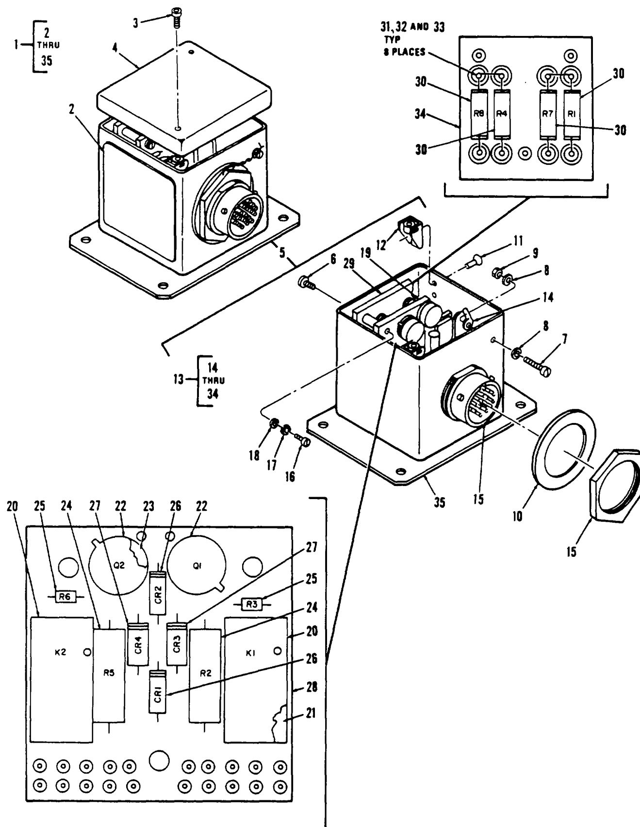
Figure 335. Control Unit, Level Sensing
