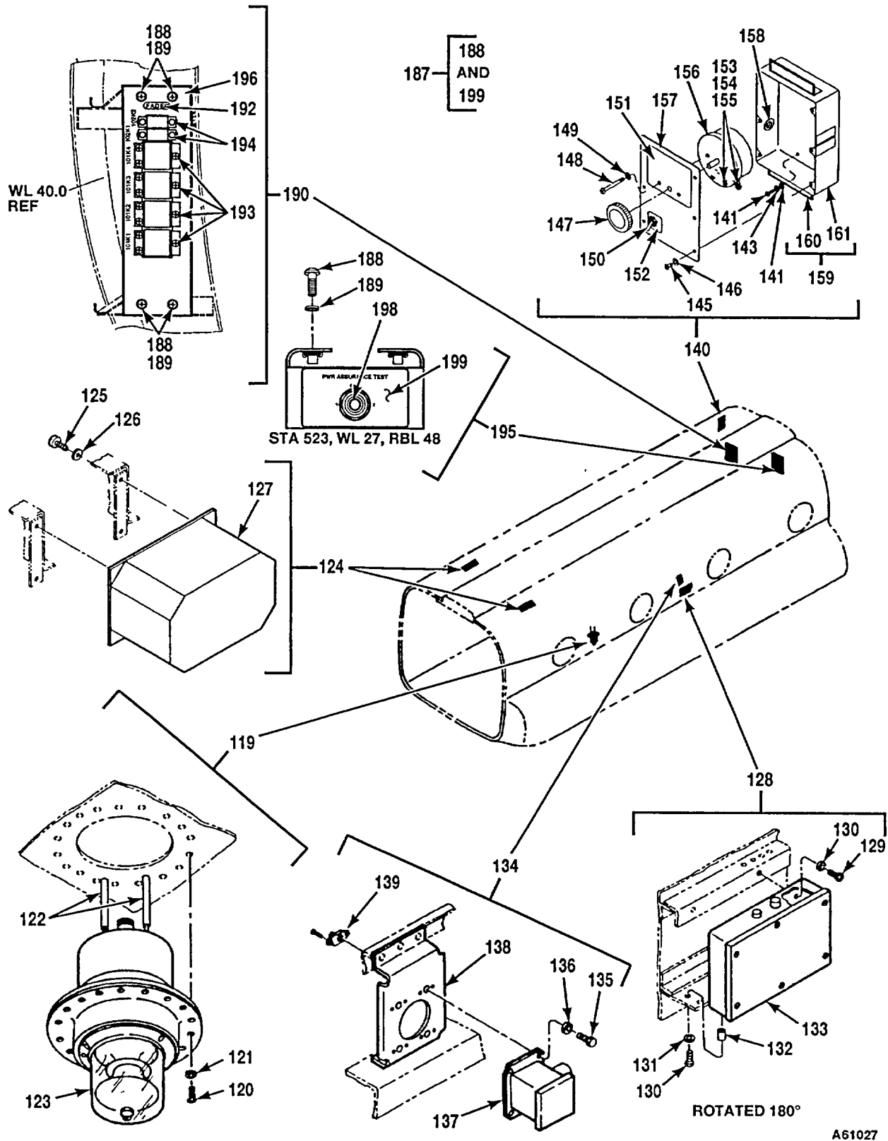
Figure 323. Equipment Instl, Cabin (Sheet 4 of 4)
