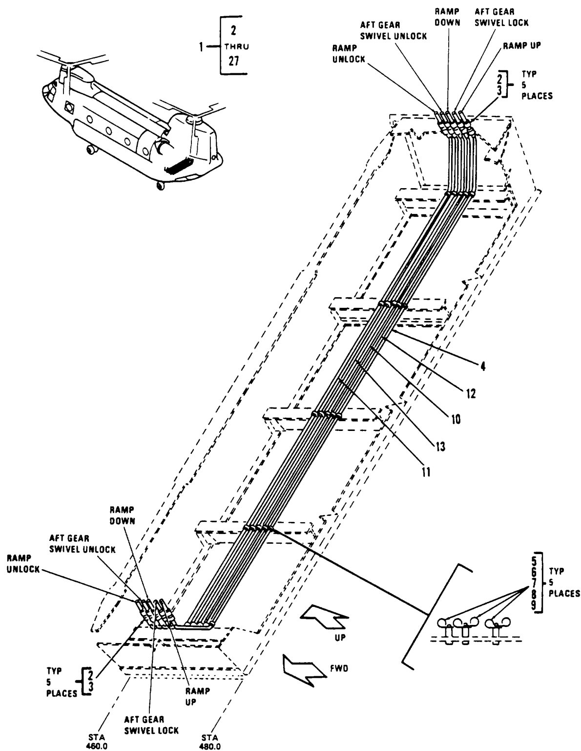
Figure 271. Tubing Instl, Hydraulic, Cabin Lower Panel, and Ramp (Sheet 1 of 2)
