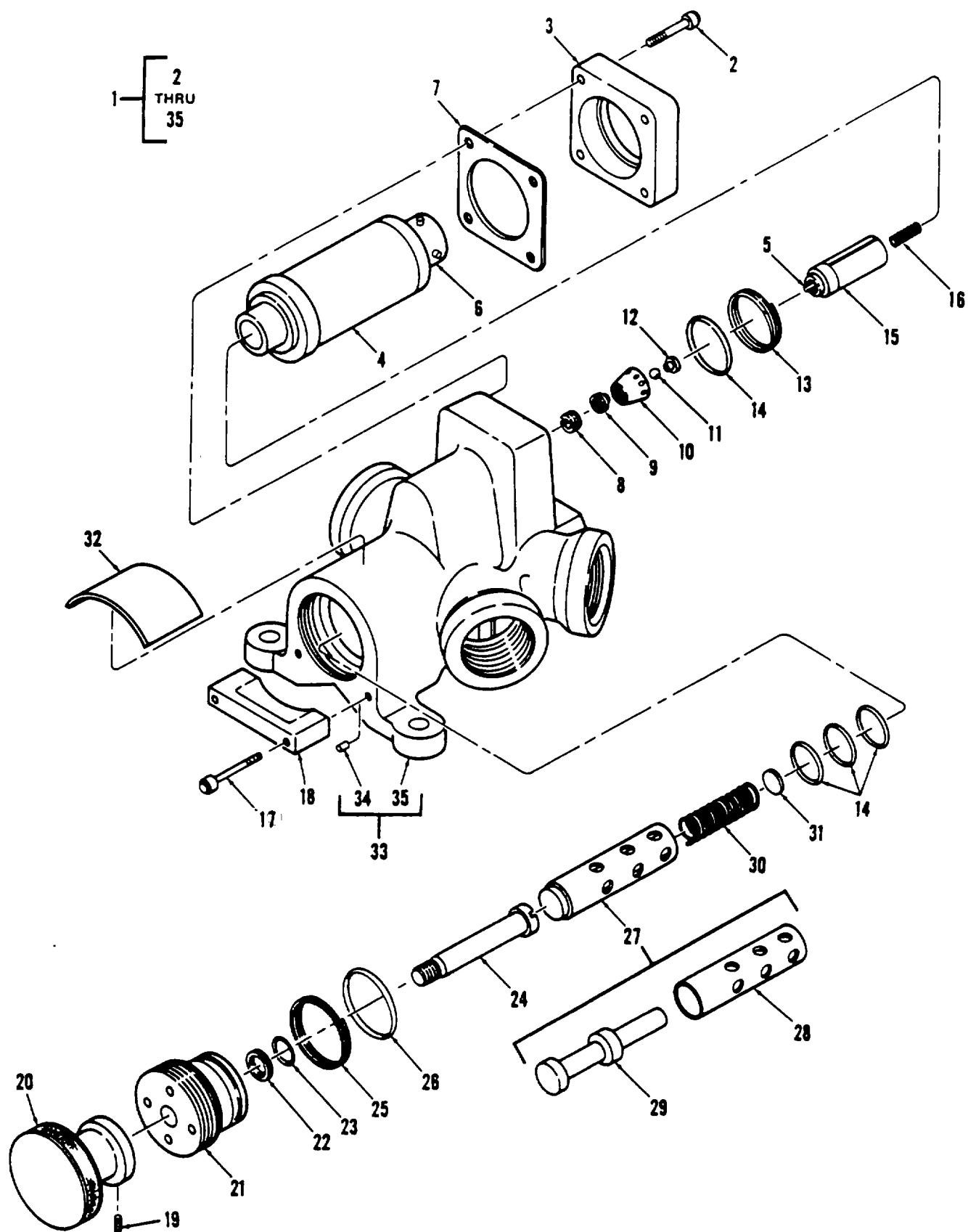
Figure 239. Valve, Solenoid HP942500-2
