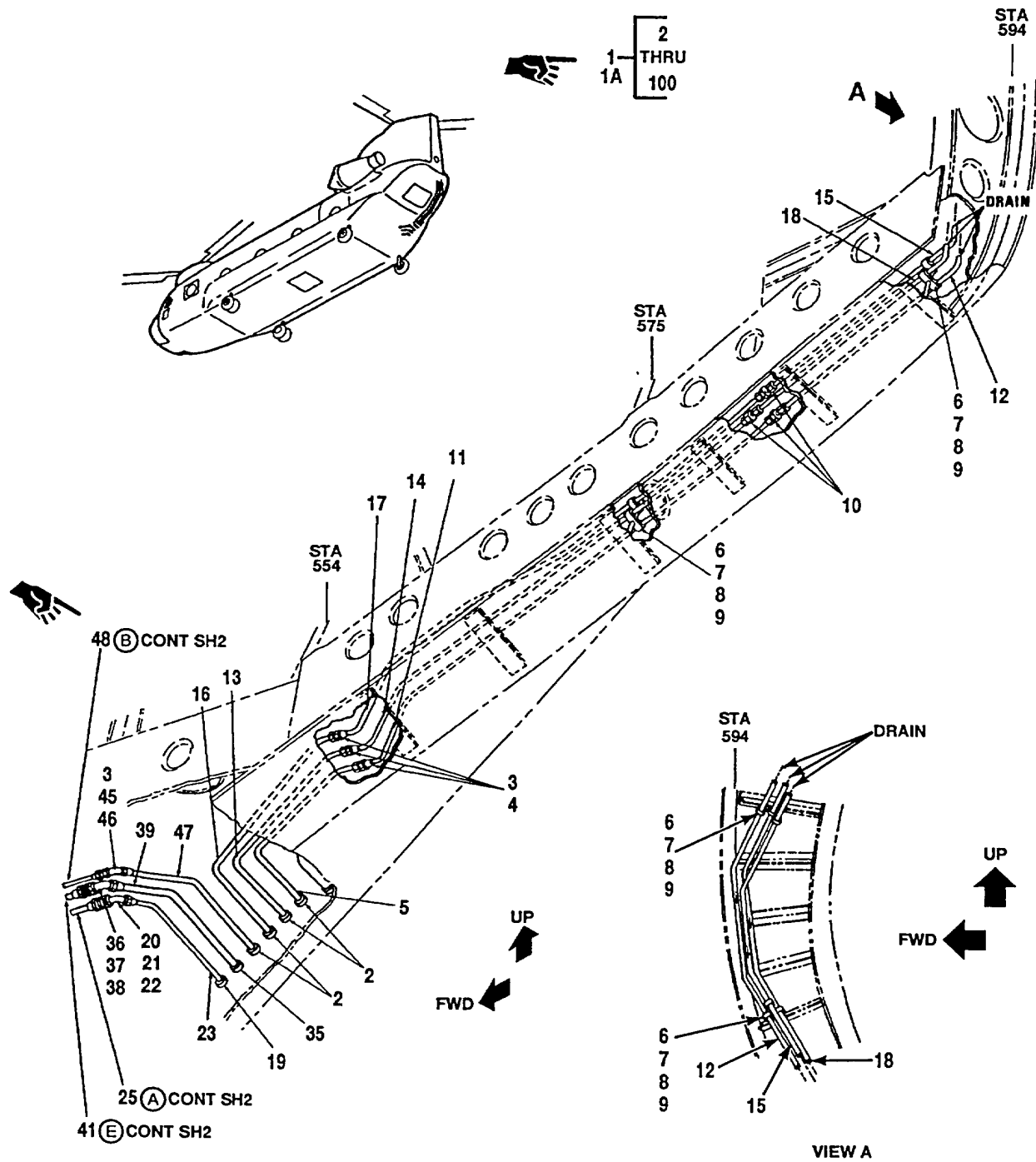
Figure 357. Tubing Instl, Aft Fuselage (Sheet 1 of 5)
