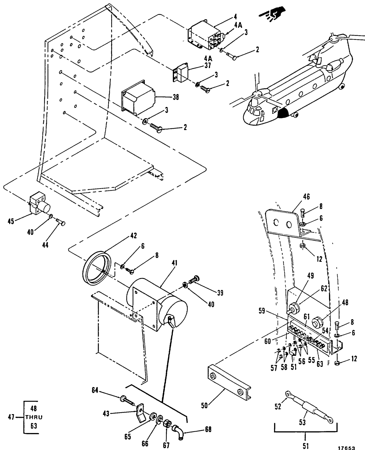
Figure 320. Equipment Installation, LH Pod, Electrical (Sheet 2 of 2)
