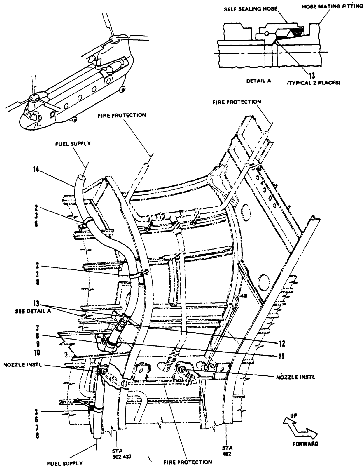
Figure 358. Tubing Instl, Powerplant (Sheet 2 of 3)
