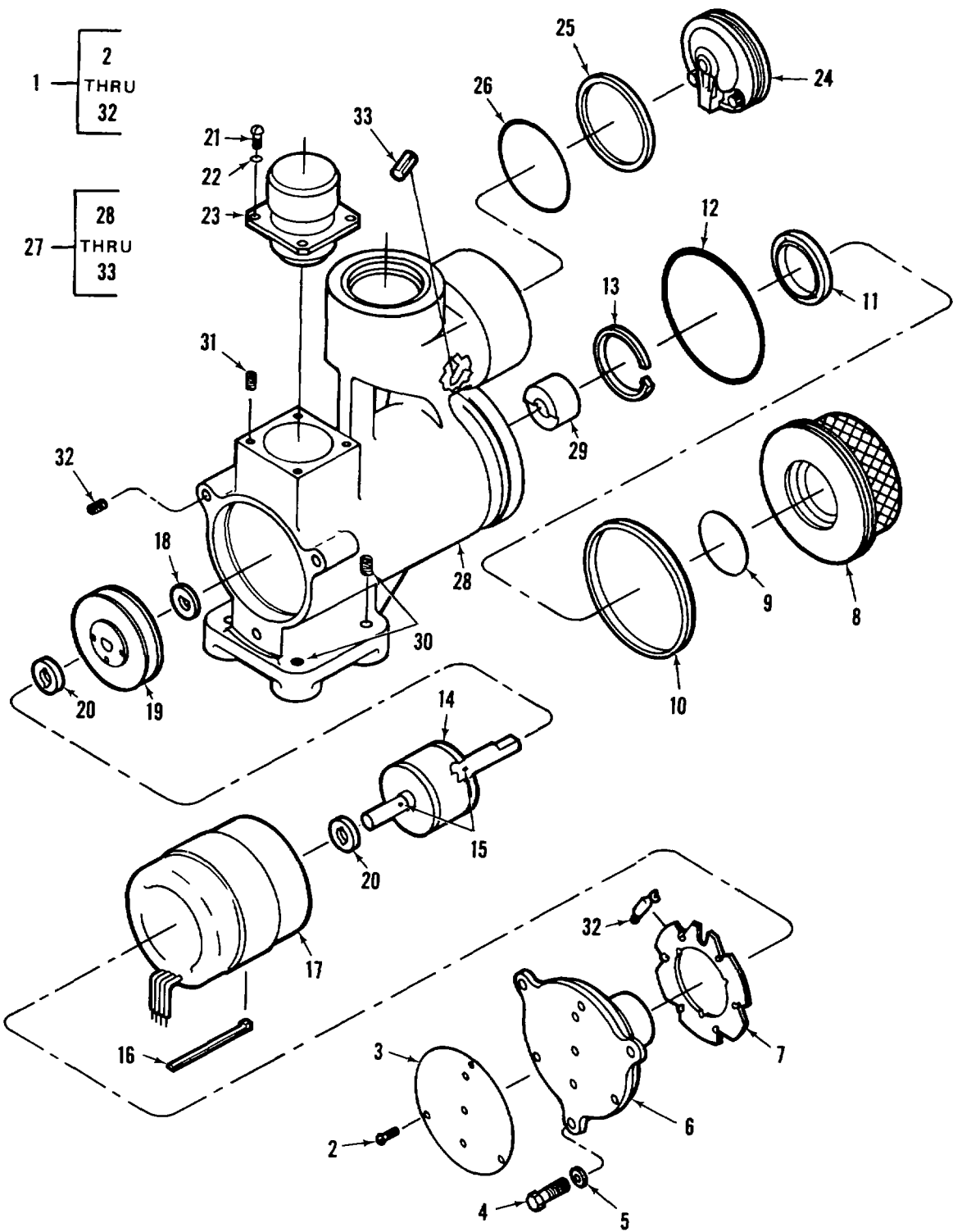
Figure 341A. Pump, Submerged
