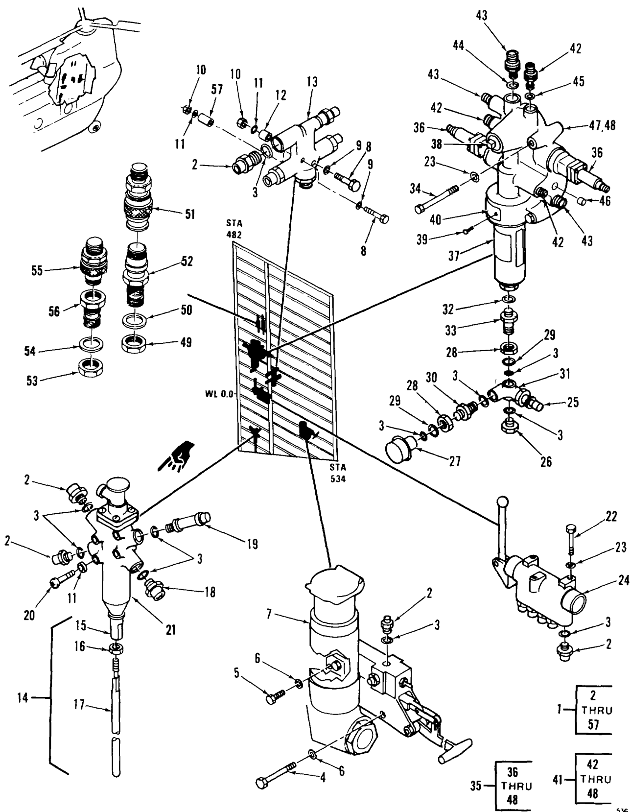
Figure 210. Equipment Instl, Sta 482 to 534, Below W/L 72
