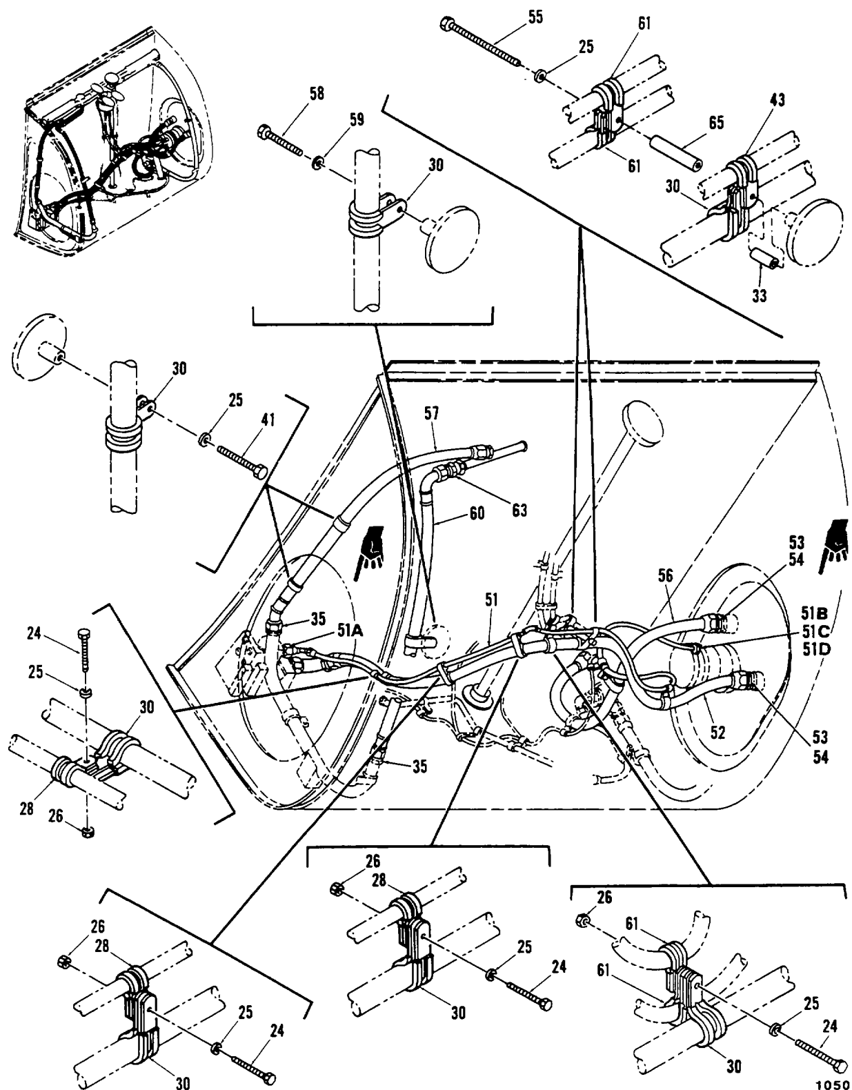
Figure 340. Fuel Cell, Fwd Auxiliary (Sheet 4 of 9)
