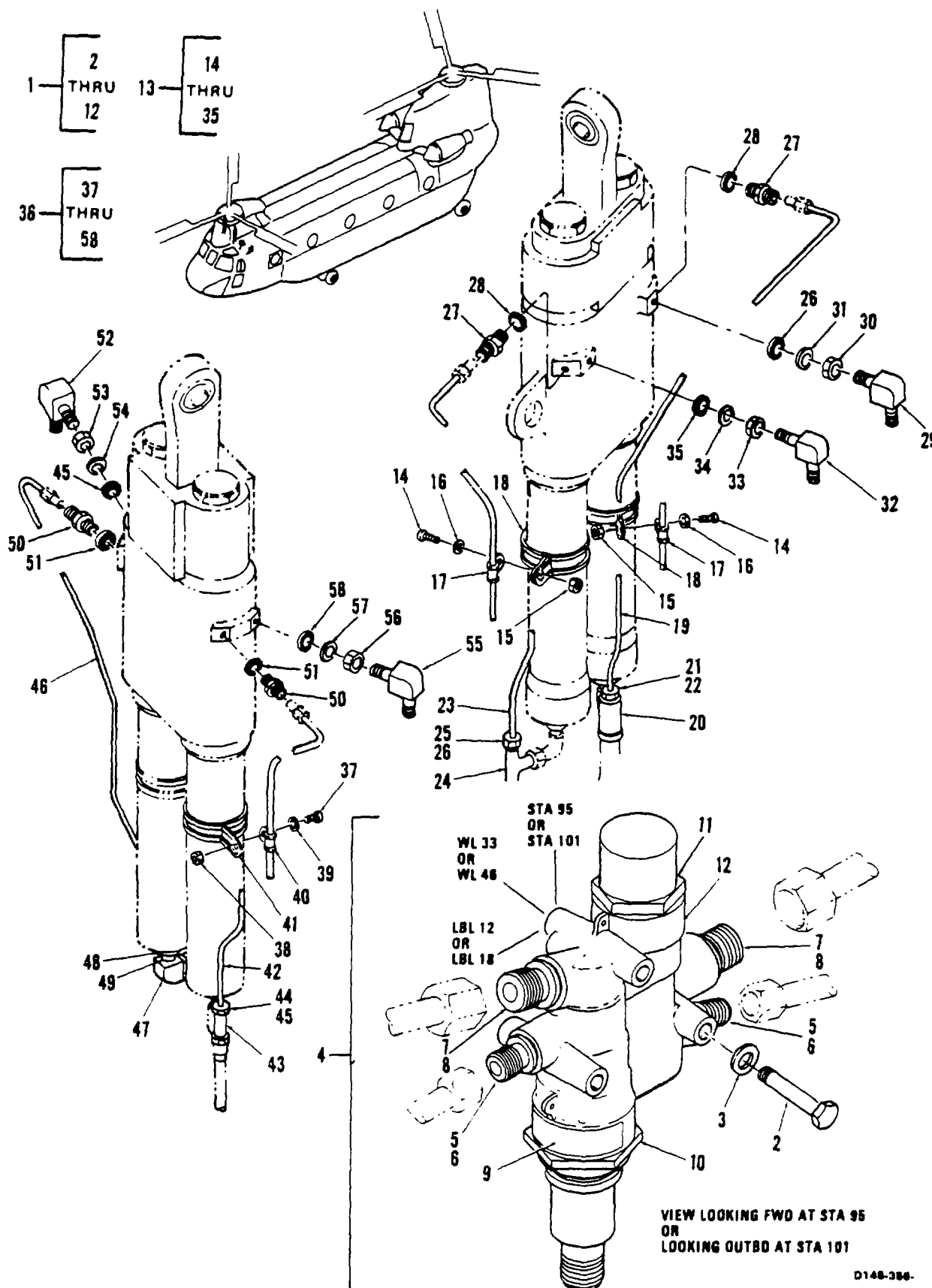
Figure 202. Equipment Instl, Sta 95 to 120
