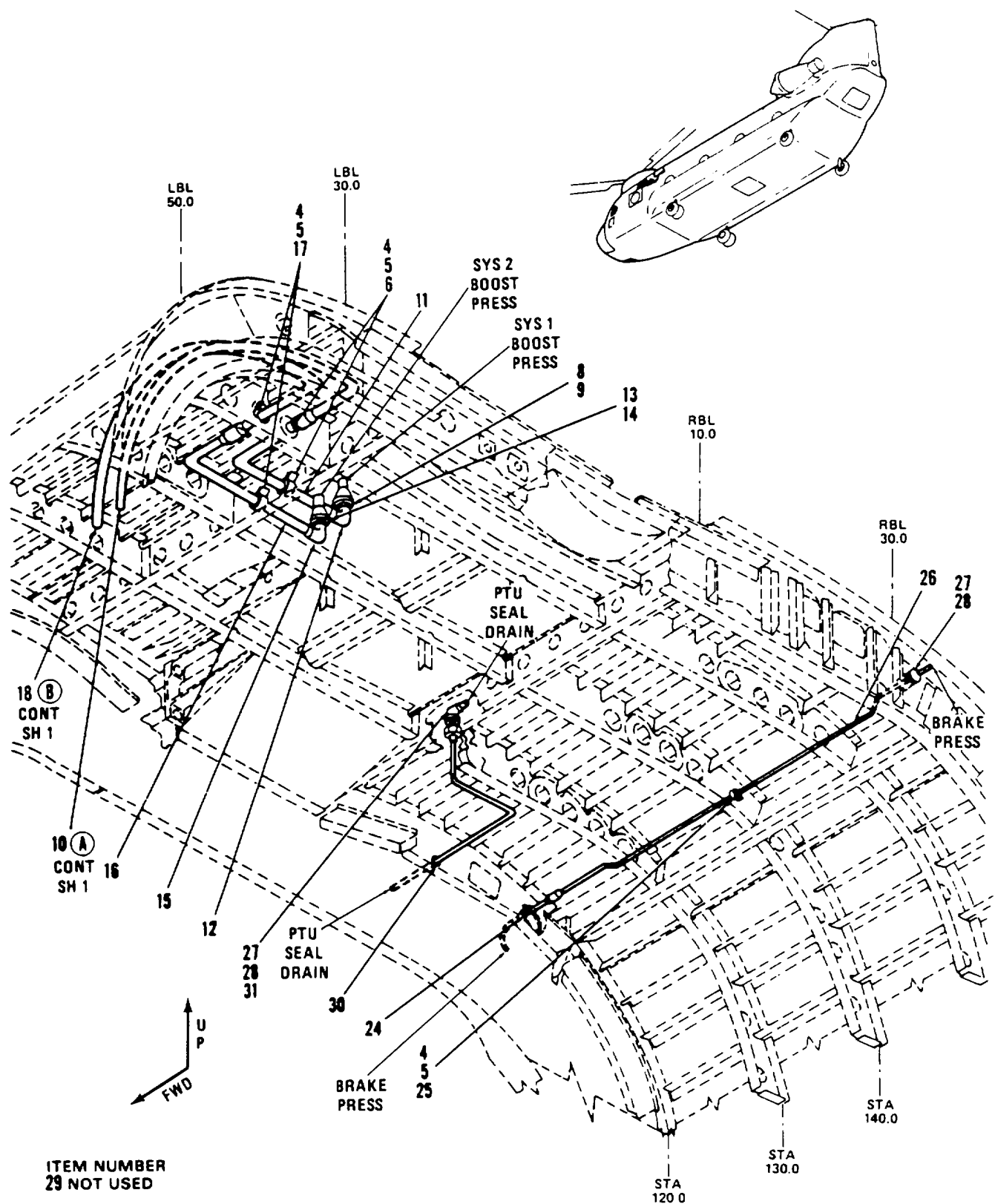
Figure 265. Tubing Instl, Hydraulic, Crown Panel and Side, LH, Sta 120 to 160 (Sheet 1 of 2)
