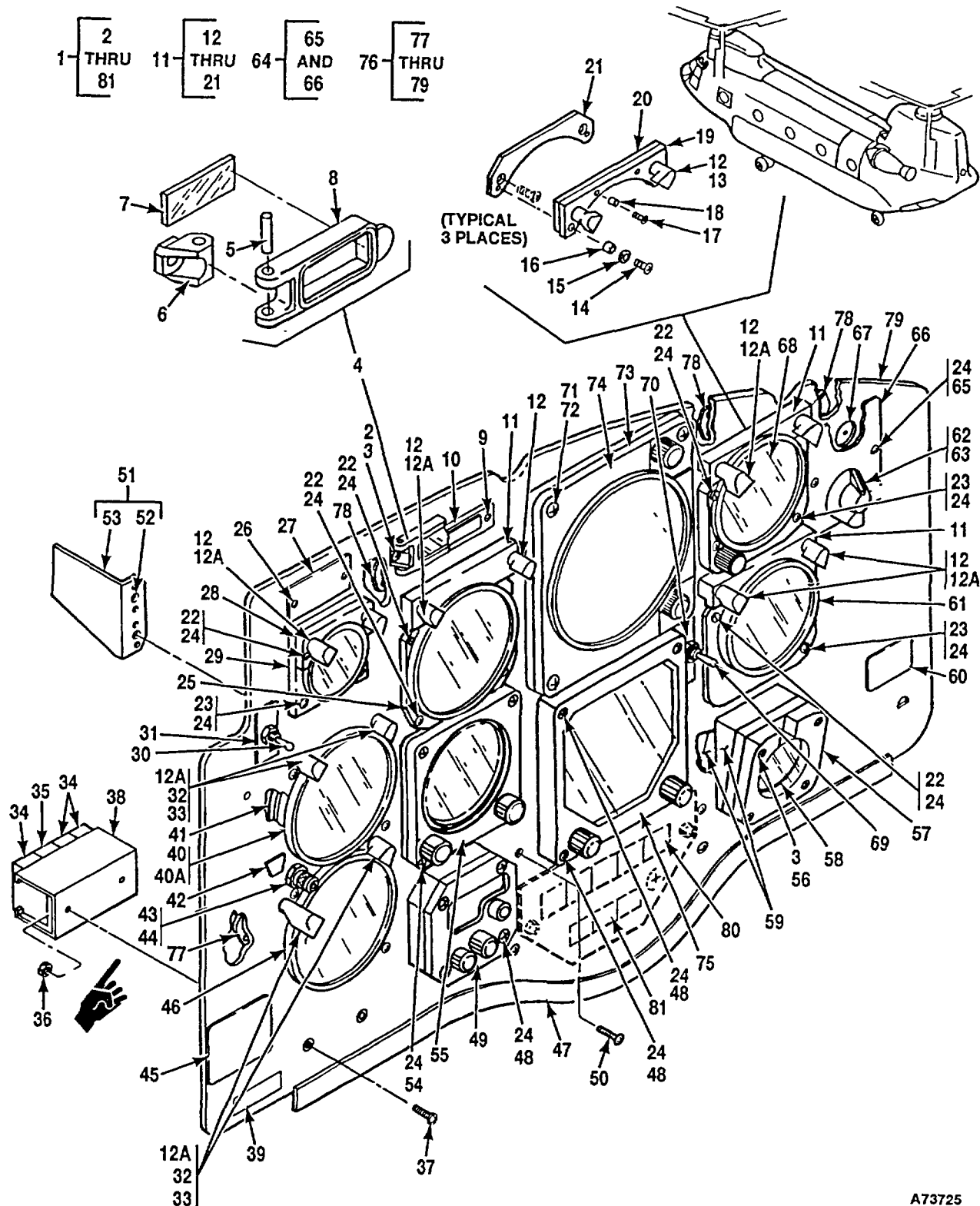
Figure 274. Panel, Instrument, Pilots
