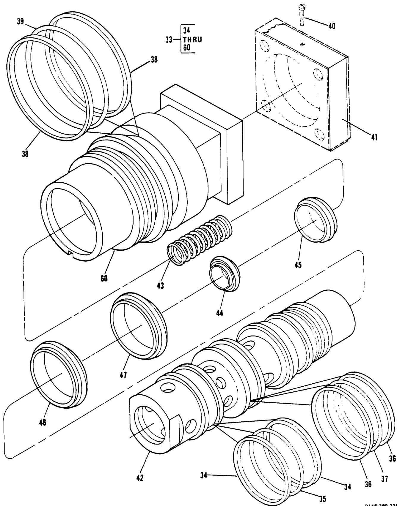
Figure 204. Valve, Solenoid HP1322100-6 (Sheet 3 of 4)
