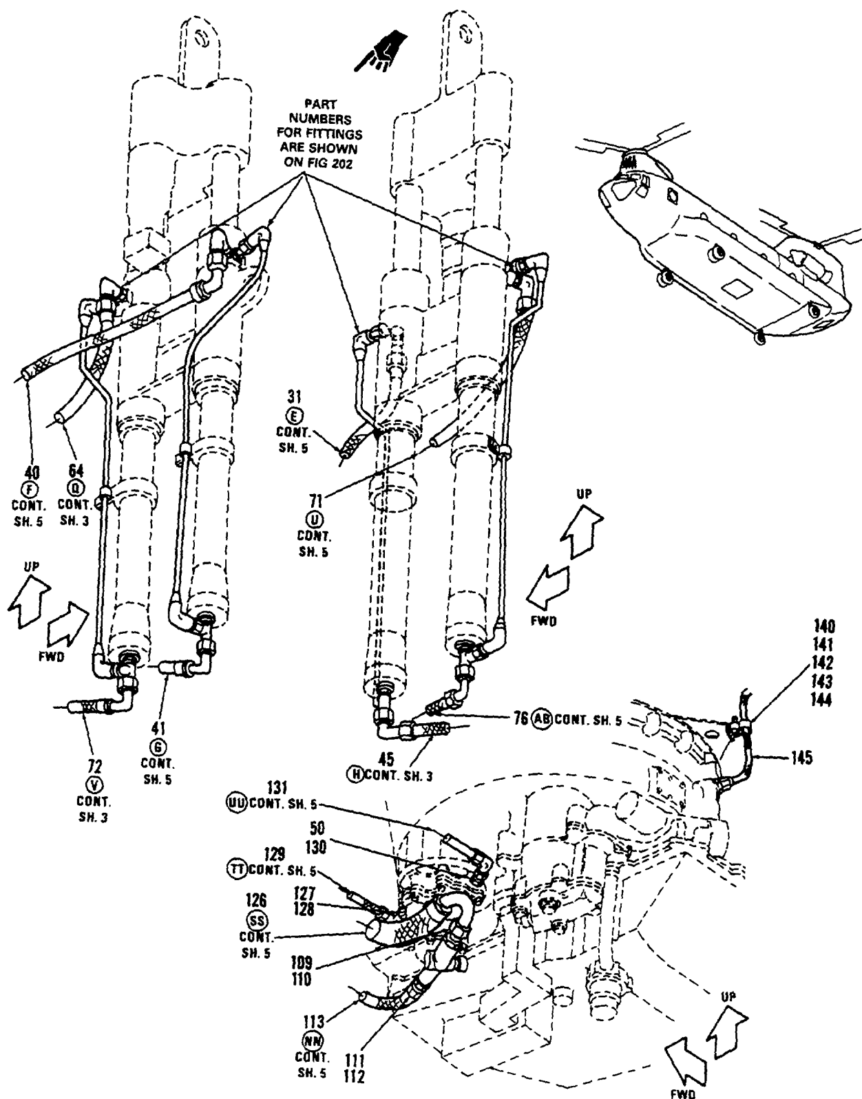
Figure 262. Tubing Instl, Hydraulics, Actuators, Fwd Transmission, Flight Controls Compartment, and Fwd Pylon (Sheet 6 of 6)
