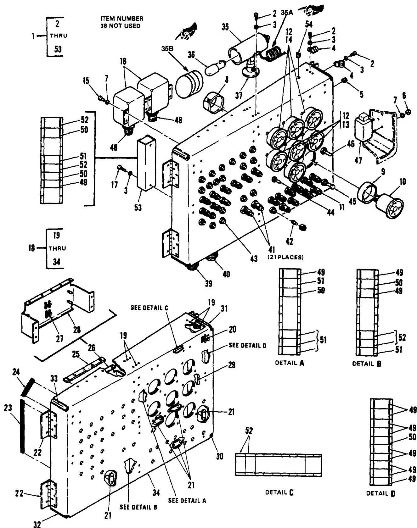
Figure 334. Panel, Transmission and Hydraulic Maintenance
