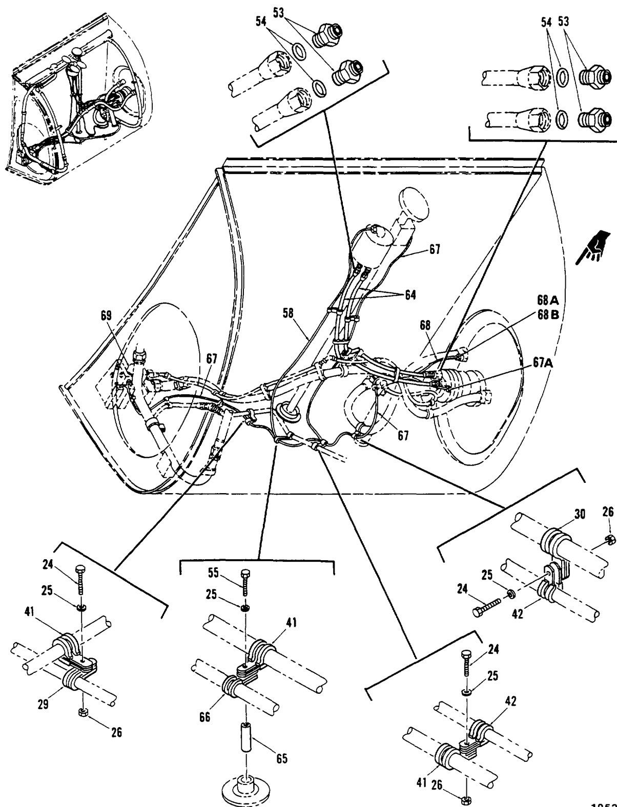
Figure 340. Fuel Cell, Fwd Auxiliary (Sheet 6 of 9)
