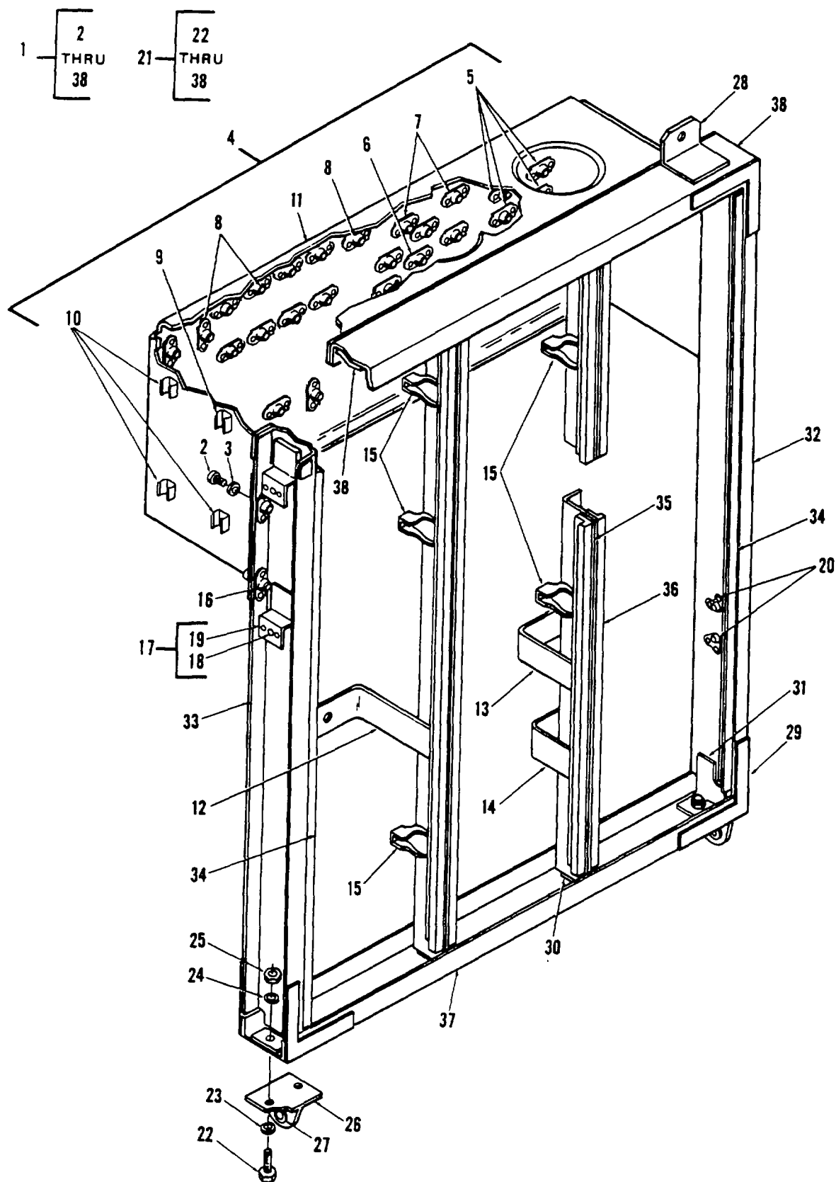
Figure 318. Panel, Overhead
