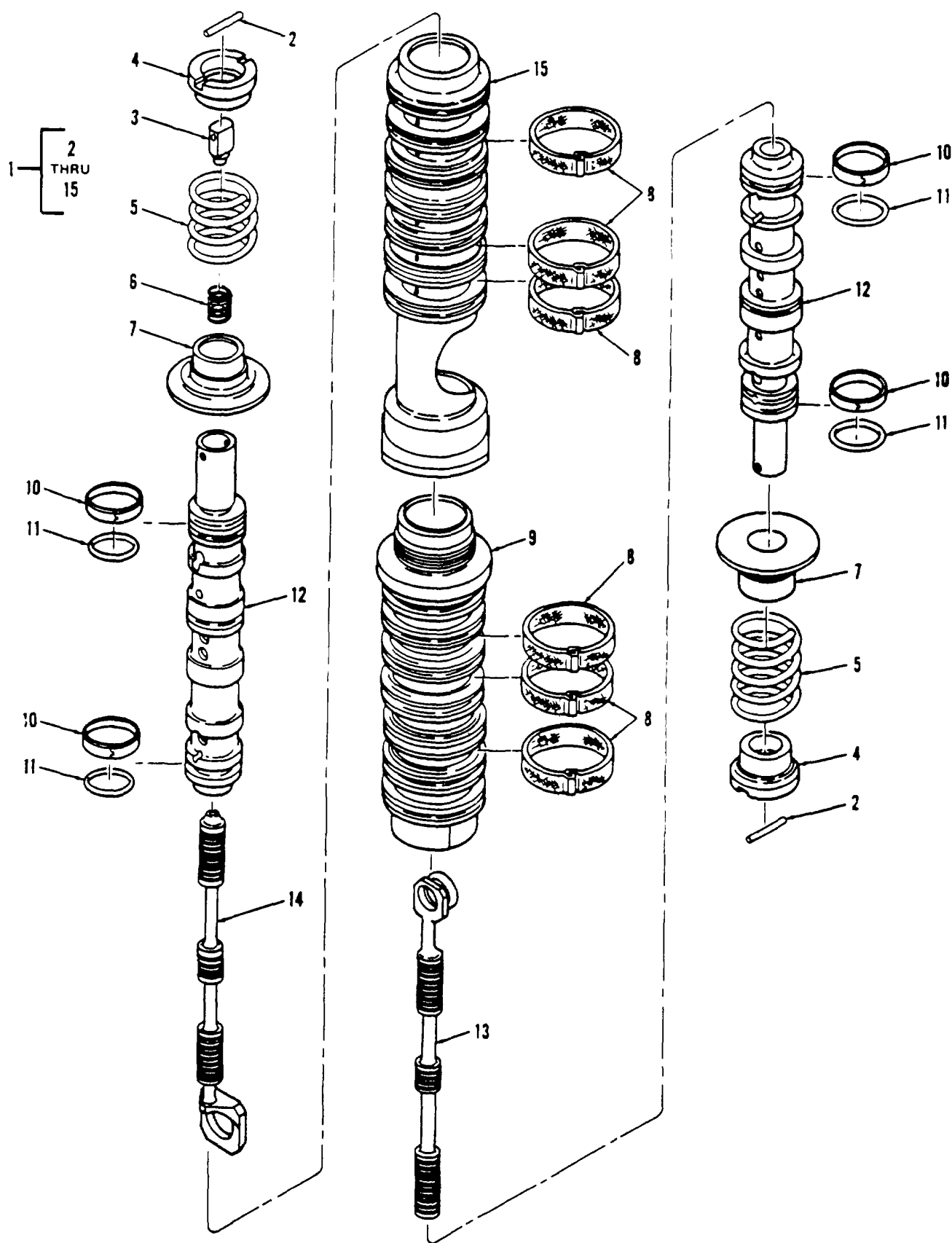
Figure 246. Servo
