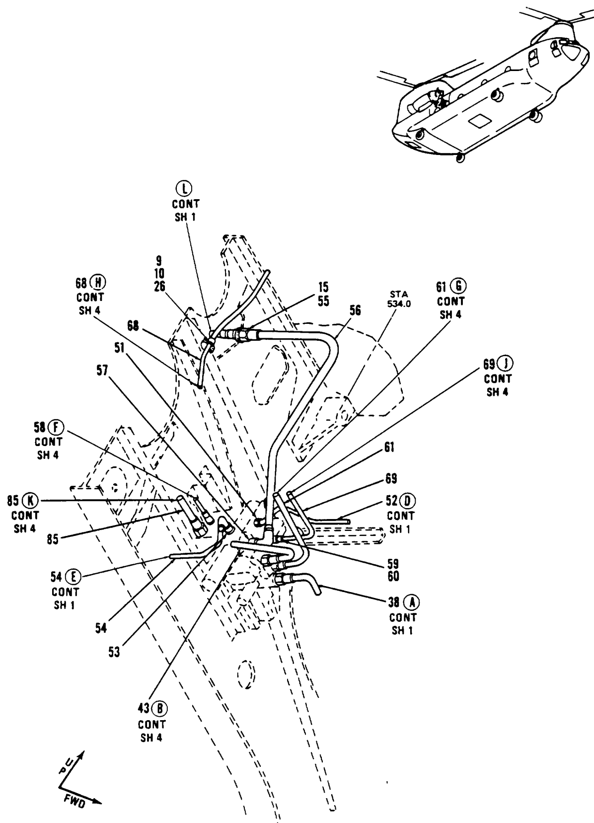
Figure 269. Tubing Instl, Hydraulic, Aft Crown Panel, LH Sta 440 to 594 (Sheet 3 of 4)
