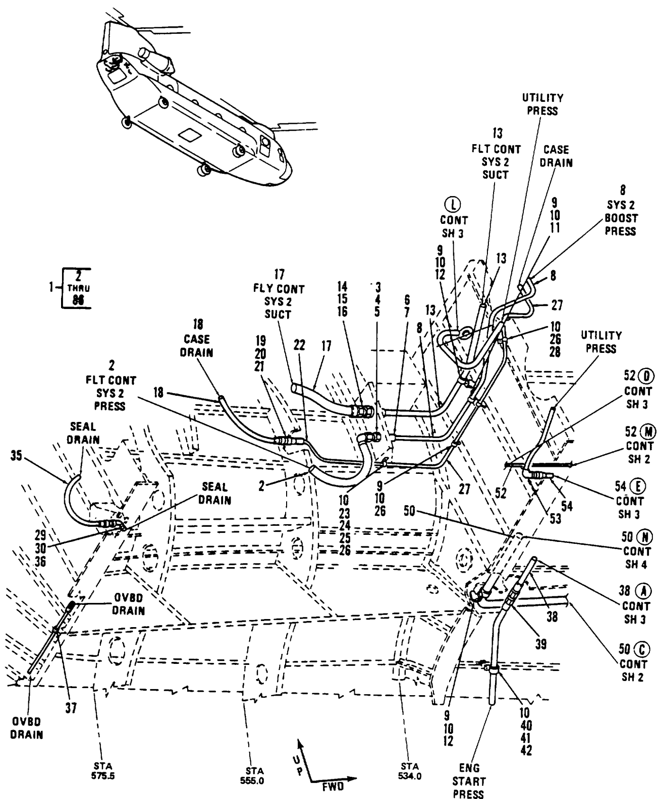
Figure 269. Tubing Instl, Hydraulic, Aft Crown Panel, LH Sta 440 to 594 (Sheet 2 of 4)
