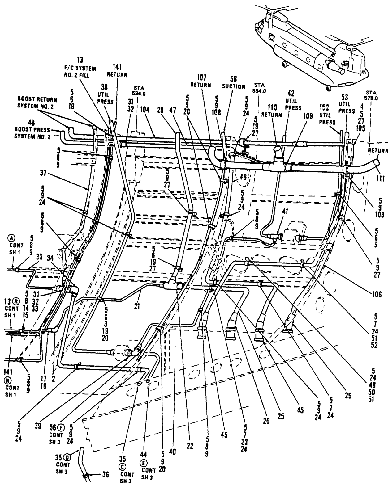
Figure 268. Tubing Instl, Hydraulic, Aft Fuselage, Lower, RH Sta 440 to 594 (Sheet 4 of 5)
