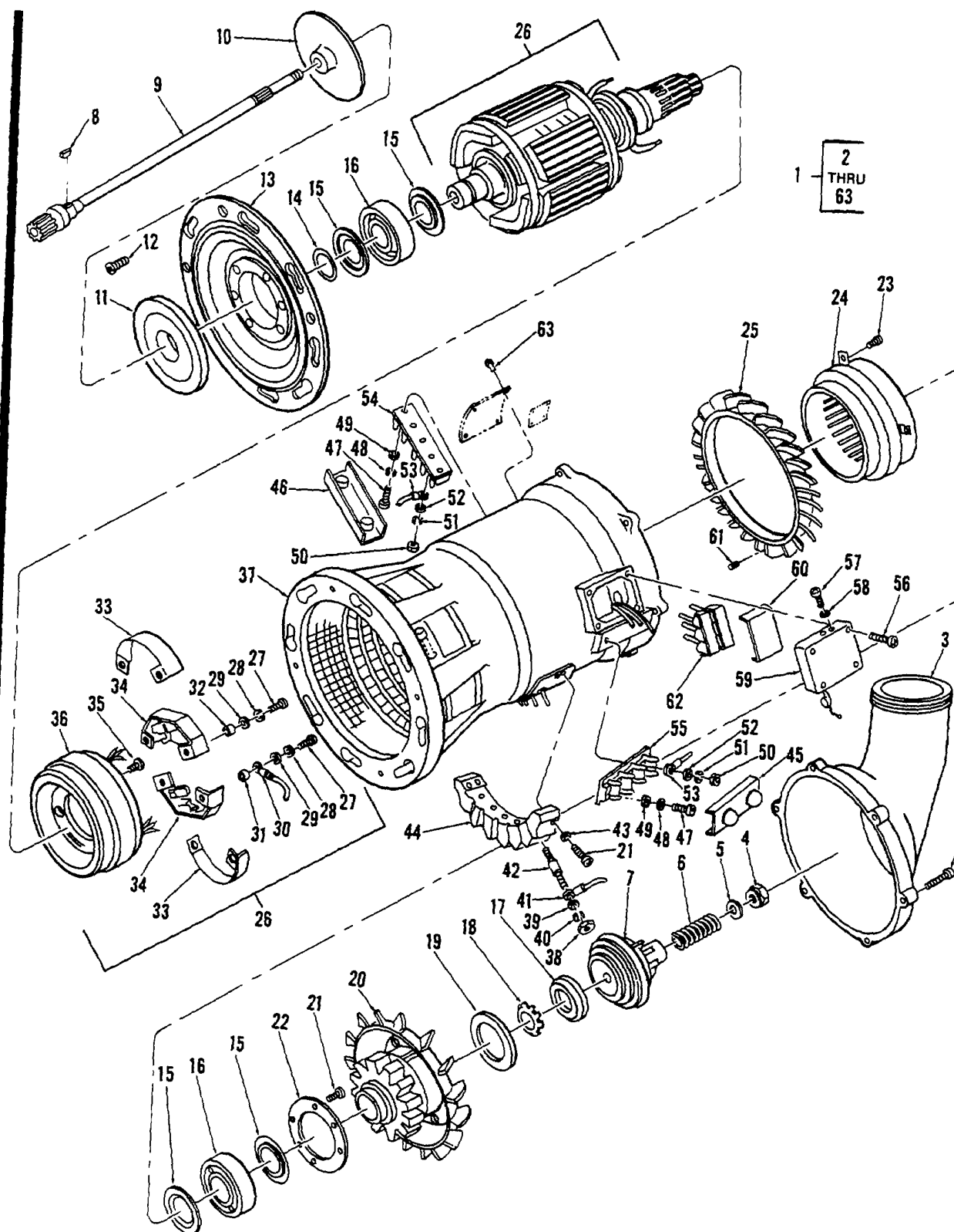
Figure 299. Generator, Alternating Current
