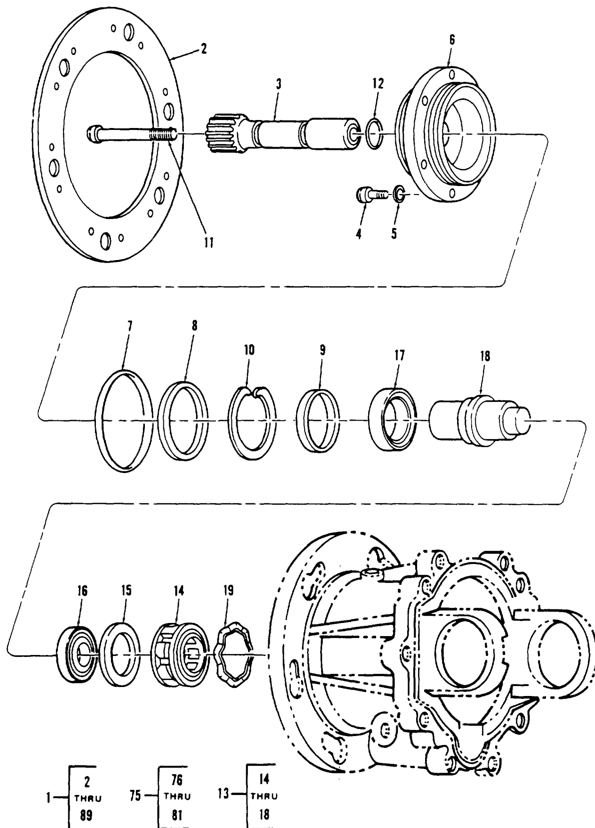
Figure 253. Starter, Engine, Hydraulic 420078 (Sheet 1 of 3)
