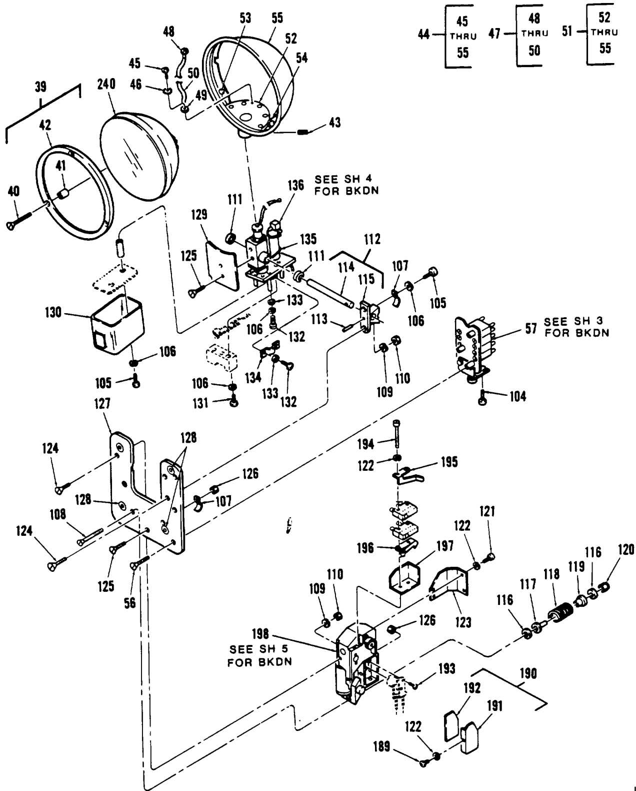
Figure 311. Light Instl, Landing and Search (Sheet 2 of 5)
