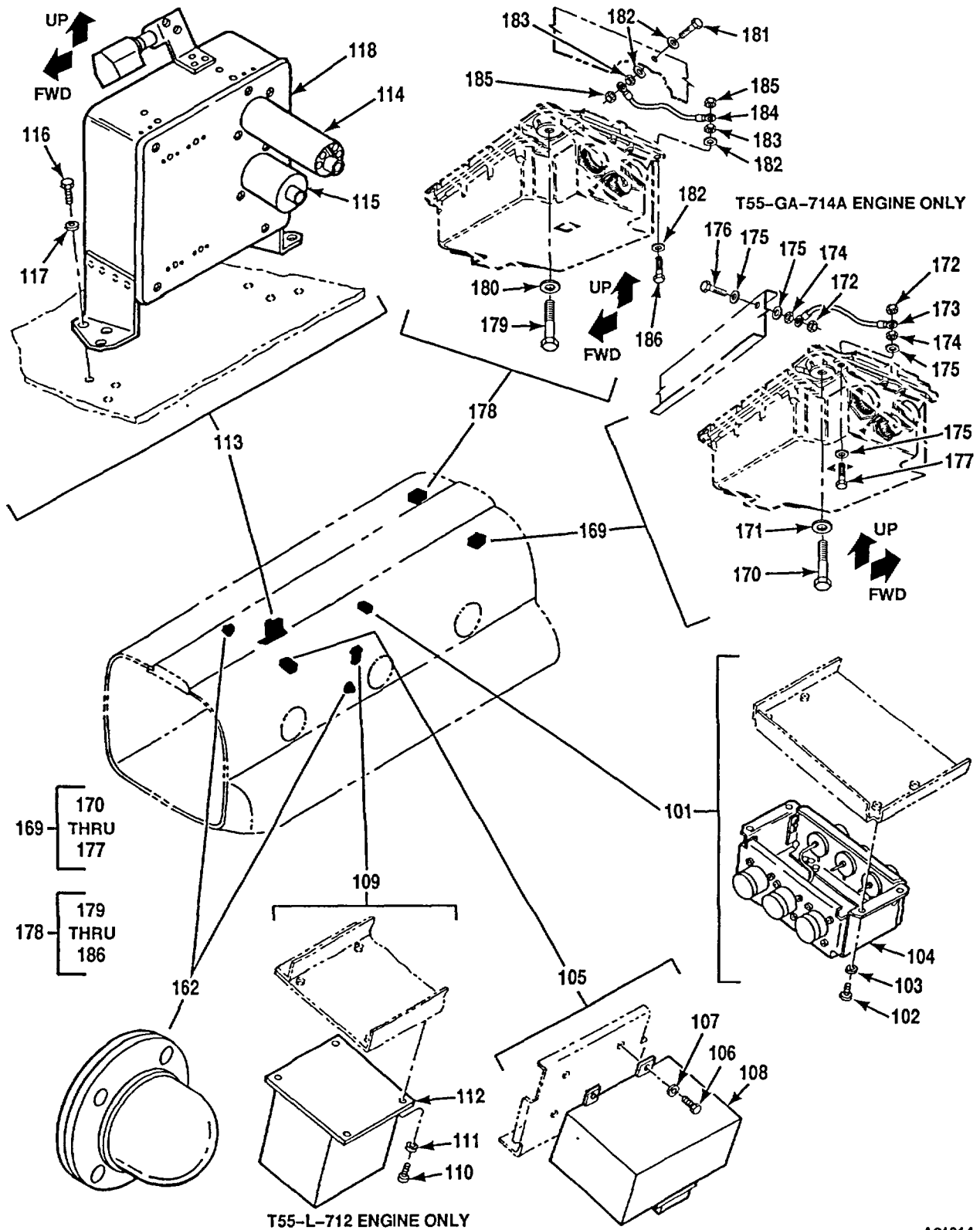
Figure 323. Equipment Instl, Cabin (Sheet 3 of 4)
