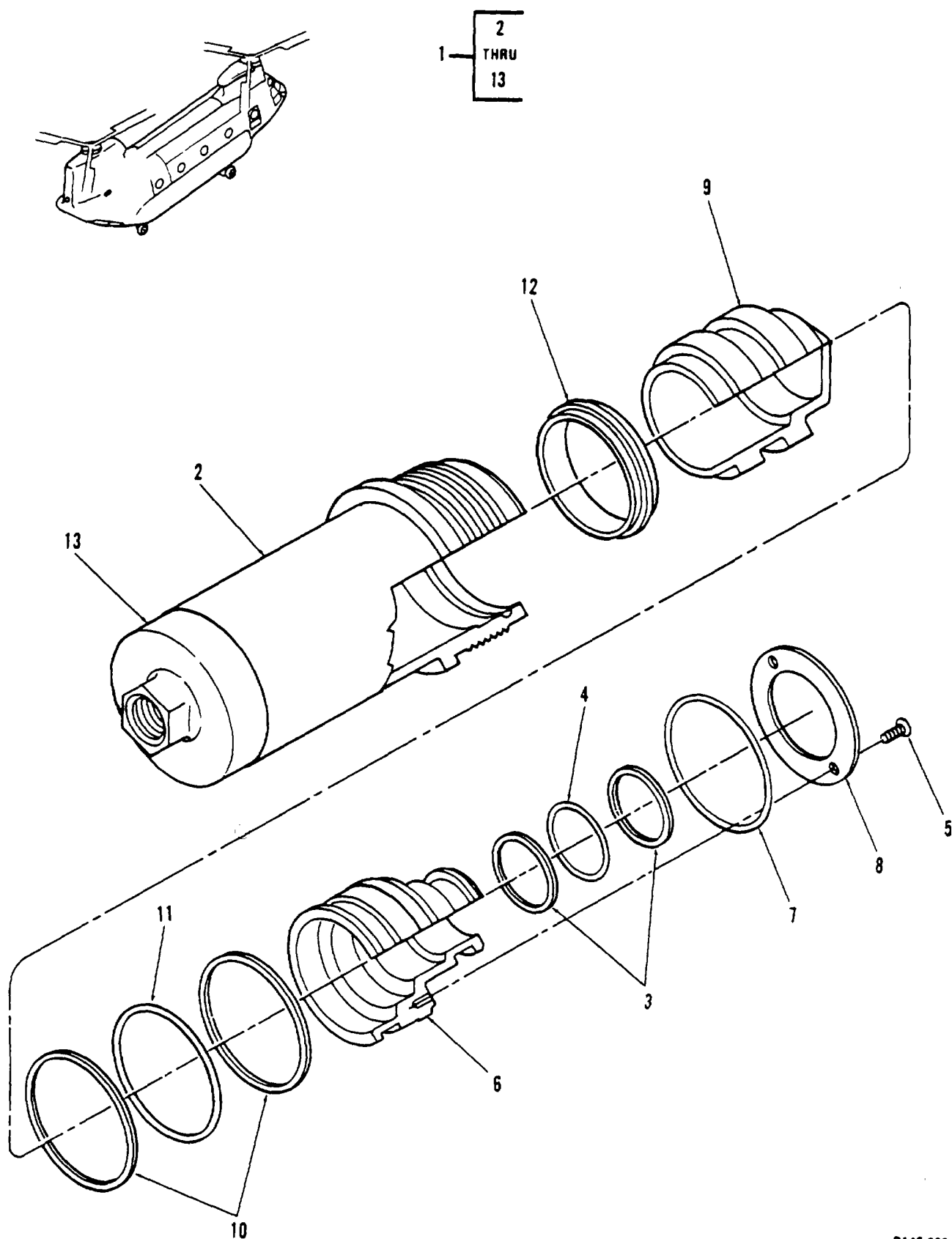
Figure 234. Accumulator, Hydraulic 60910
