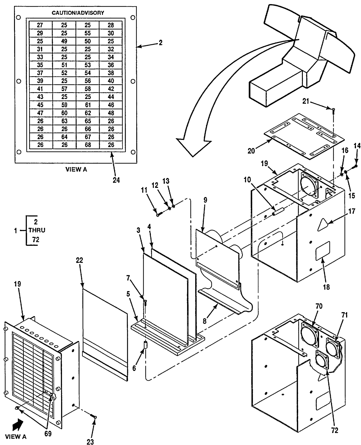
Figure 339A. Panel, Master Caution (T55-GA-714A Engine)
