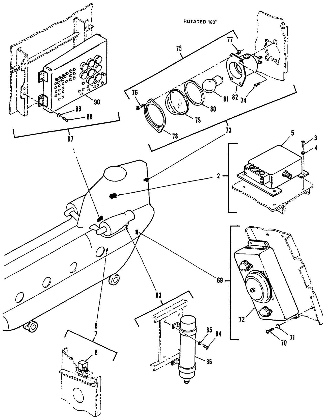
Figure 332. Equipment Instl, Tail, Electrical (Sheet 3 of 4)
