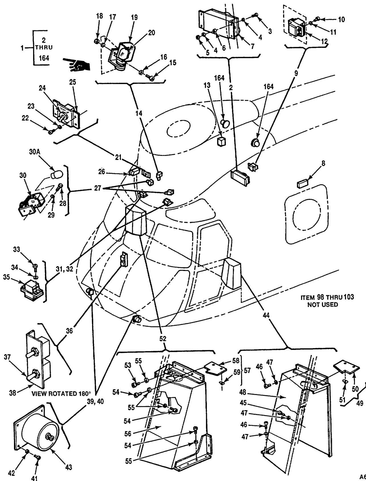
Figure 303. Equipment Instl, Nose, Electrical (Sheet 1 of 2)
