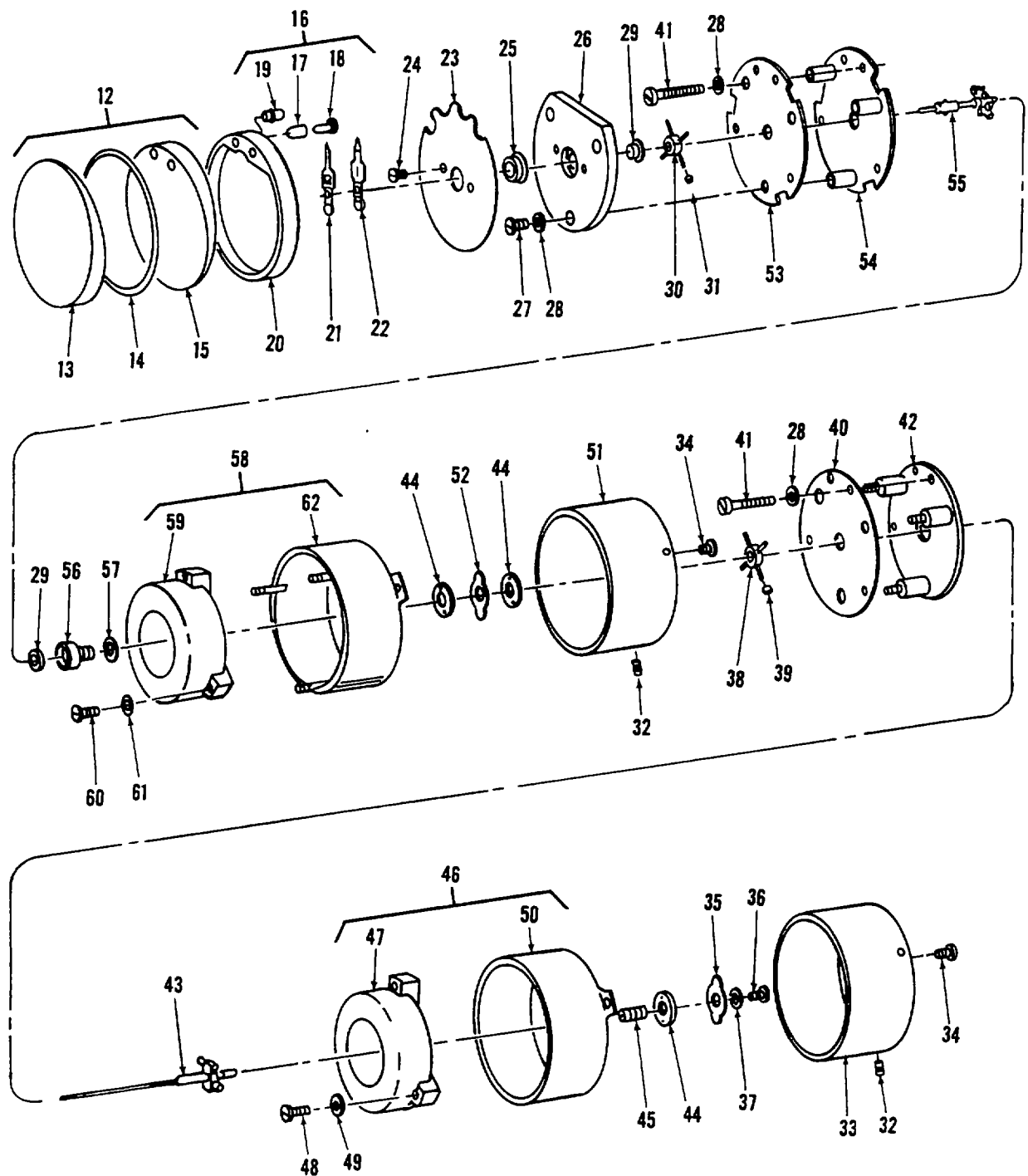
Figure 280. Indicator, Fuel Flow (Sheet 2 of 2)
