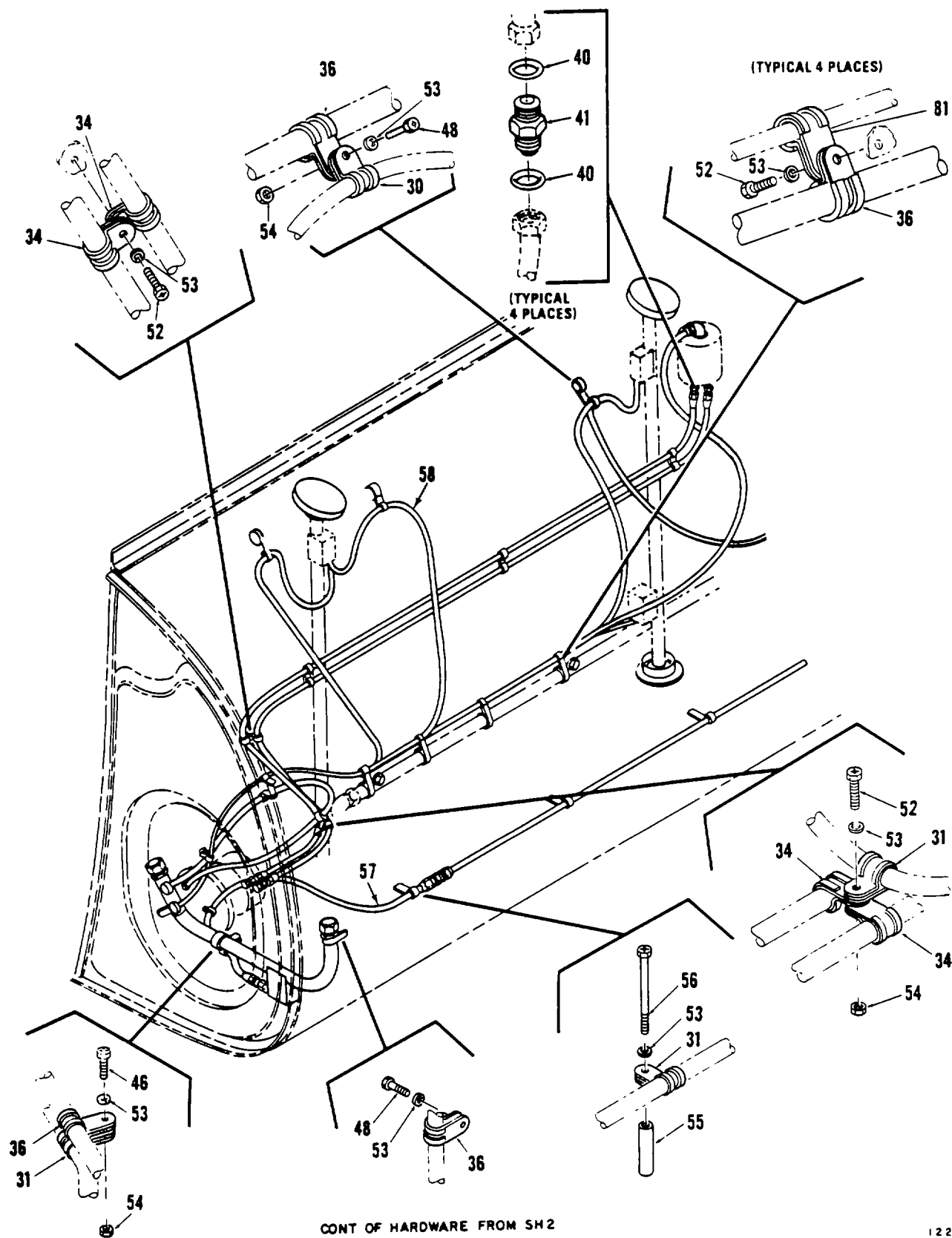
Figure 345. Fuel Cell, Main (Sheet 3 of 8)
