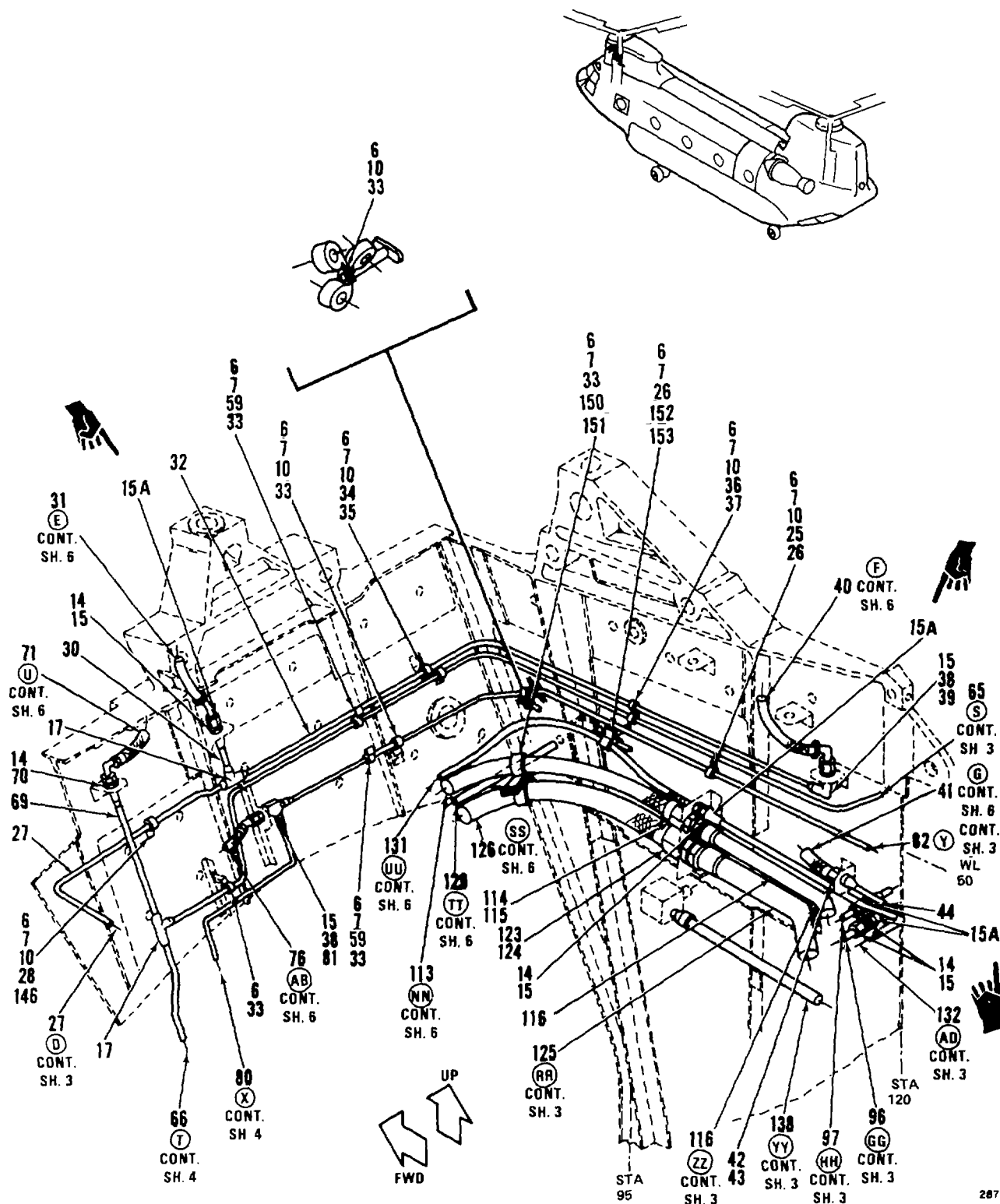
Figure 262. Tubing Instl, Hydraulics, Actuators, Fwd Transmission, Flight Controls Compartment, and Fwd Pylon (Sheet 5 of 6)
