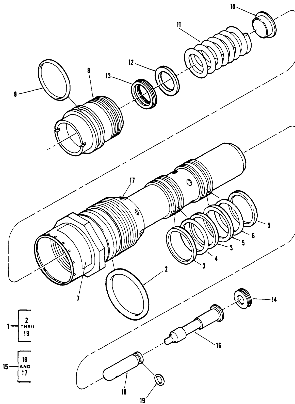
Figure 205. Reducer, Pressure 60610
