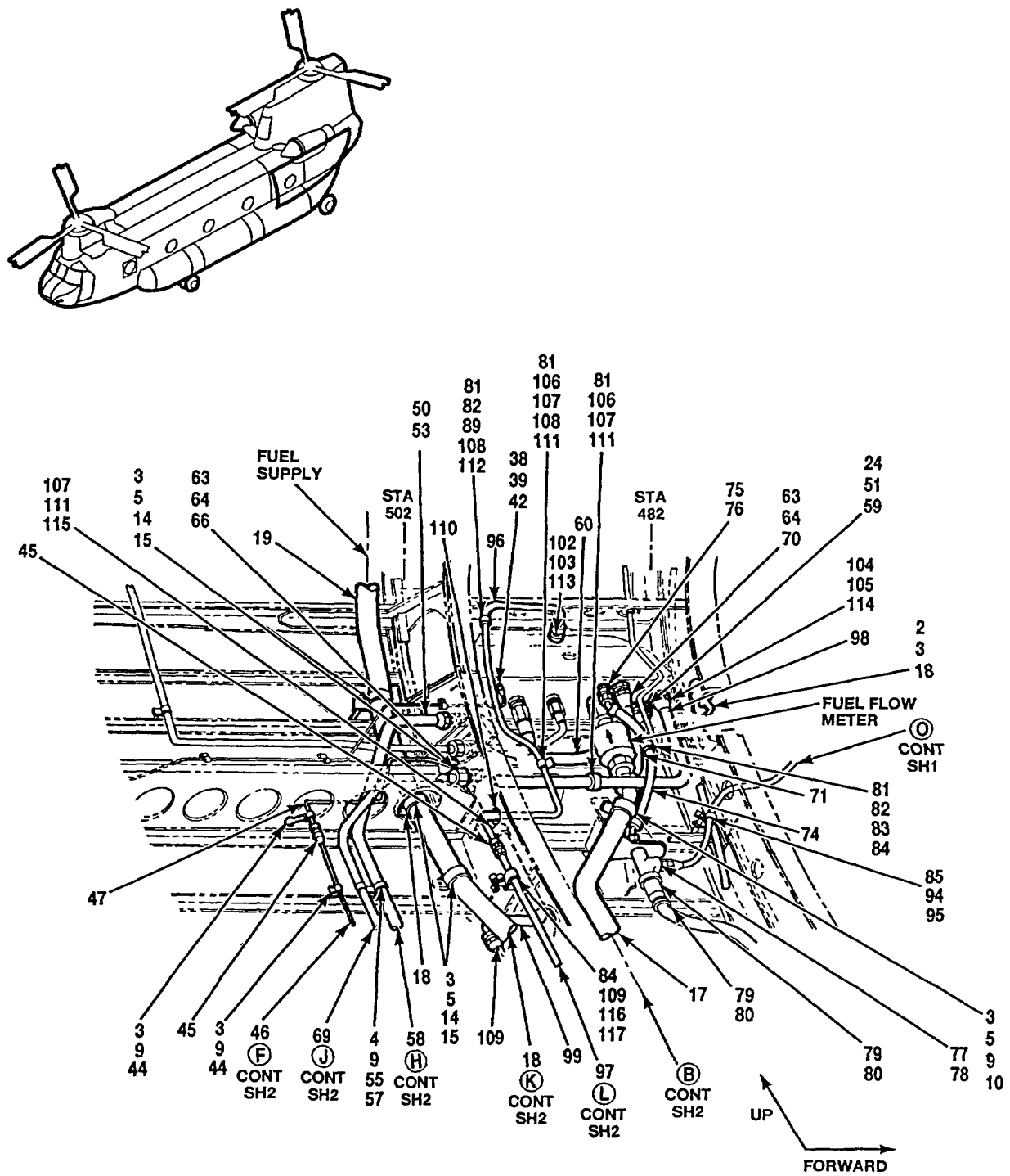
Figure 356. Tubing Instl, Aft Fuselage (Sheet 3 of 4)
