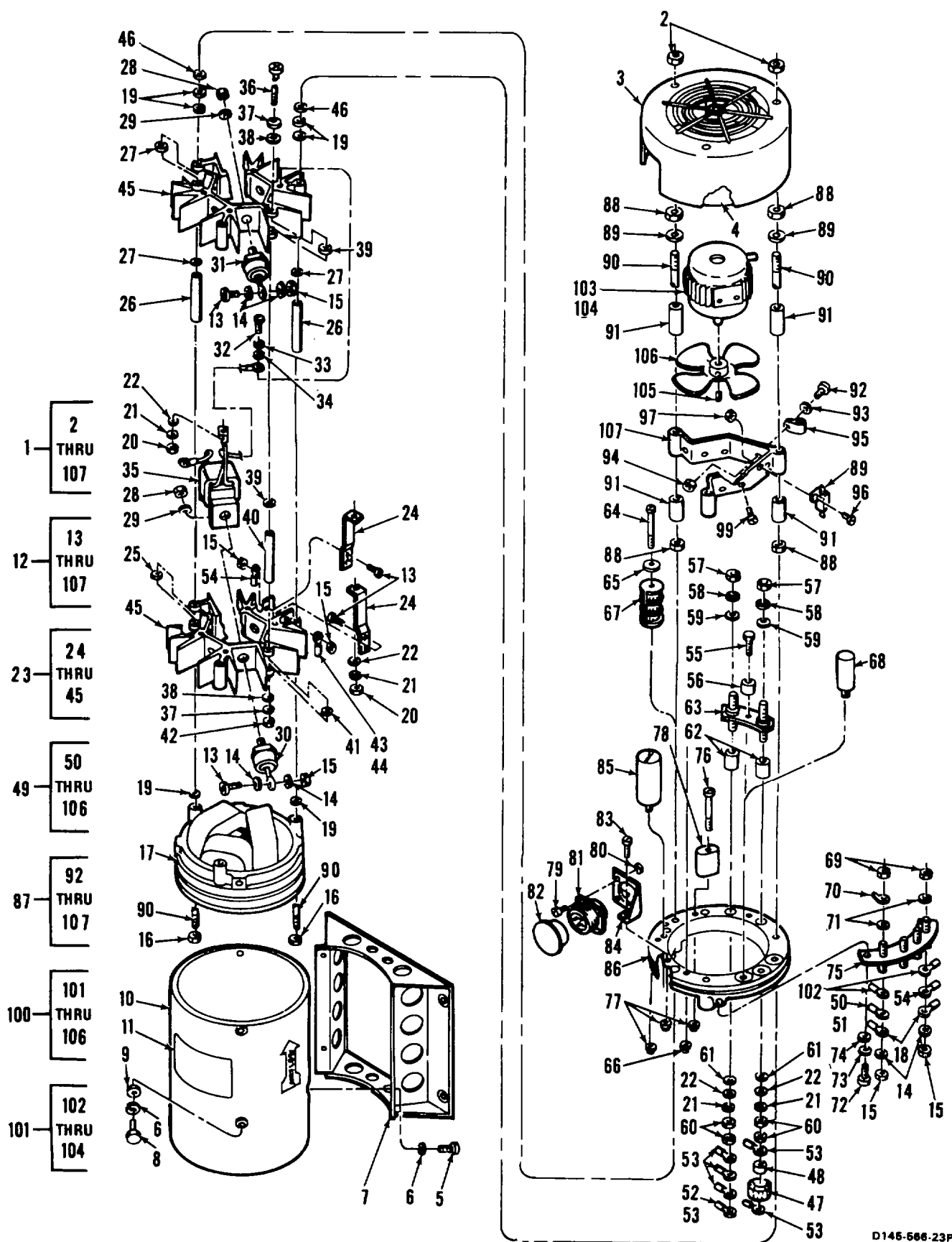
Figure 321. Power Supply, 28VS200Y9
