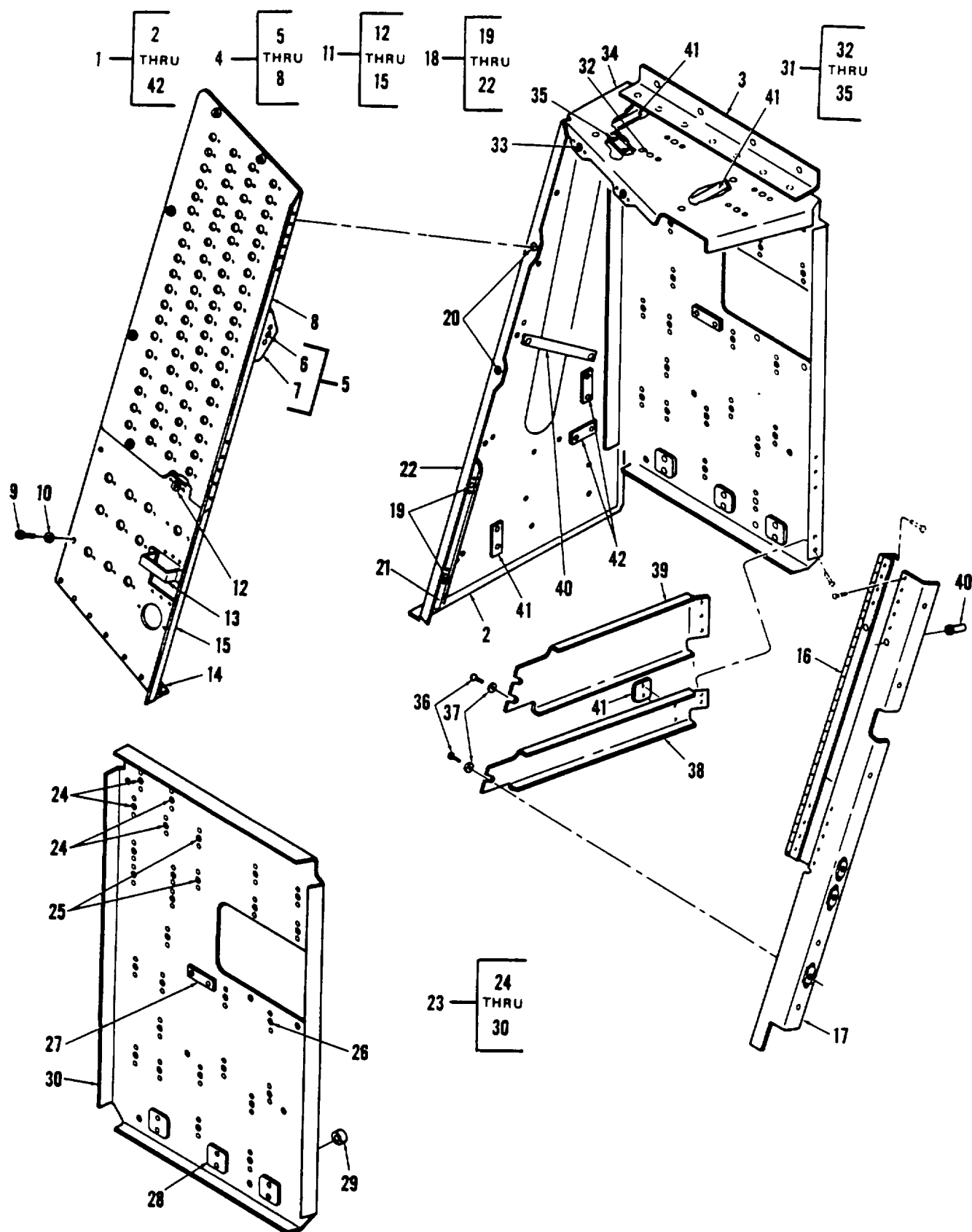
Figure 308. Structure, Power Distribution Panel, LH
