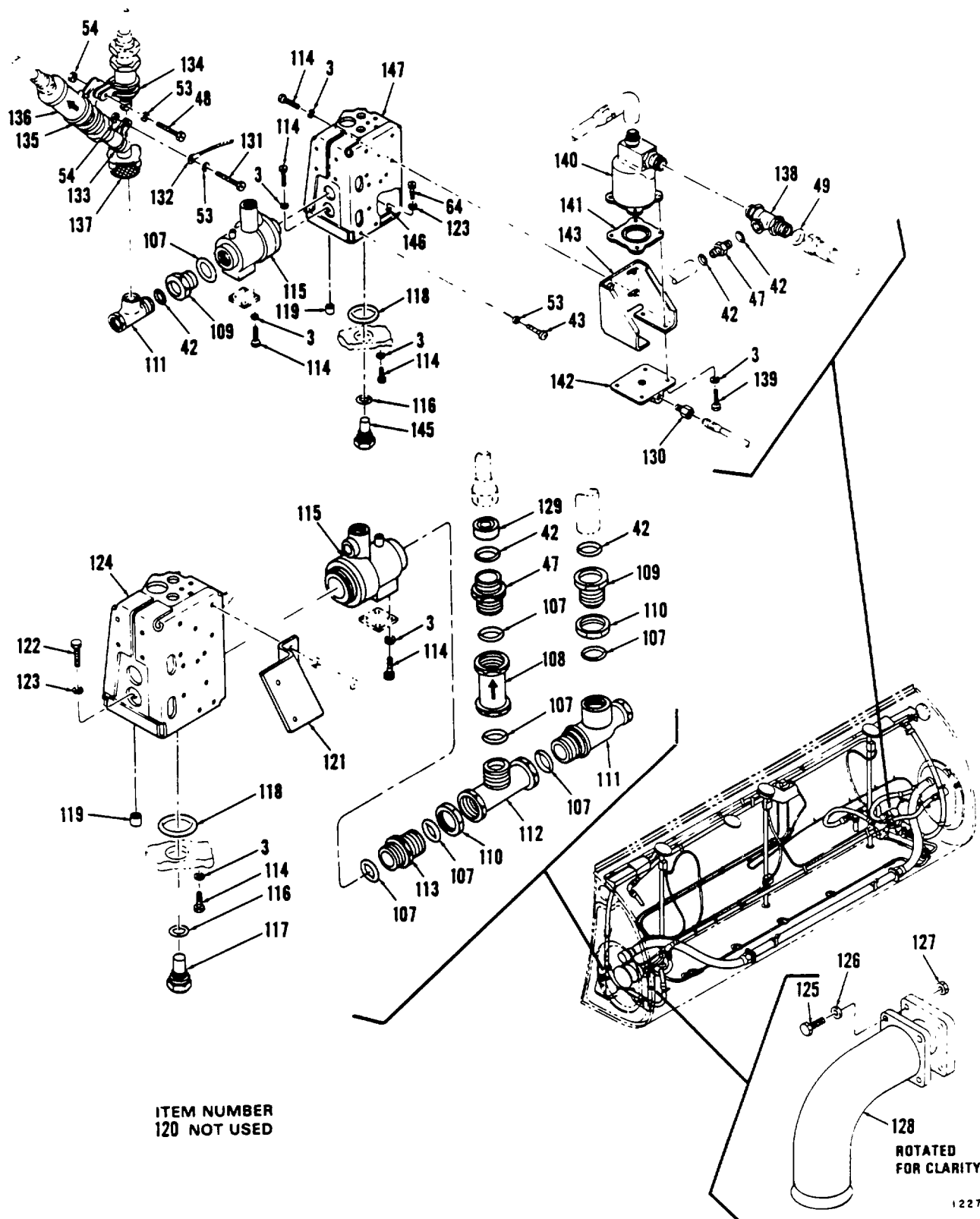
Figure 345. Fuel Cell, Main (Sheet 7 of 8)
