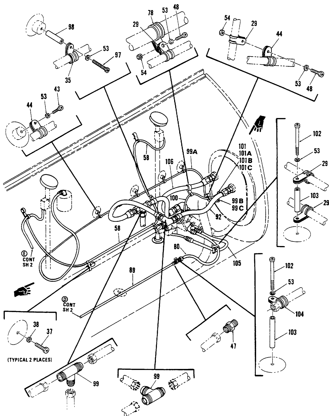
Figure 345. Fuel Cell, Main (Sheet 6 of 8)
