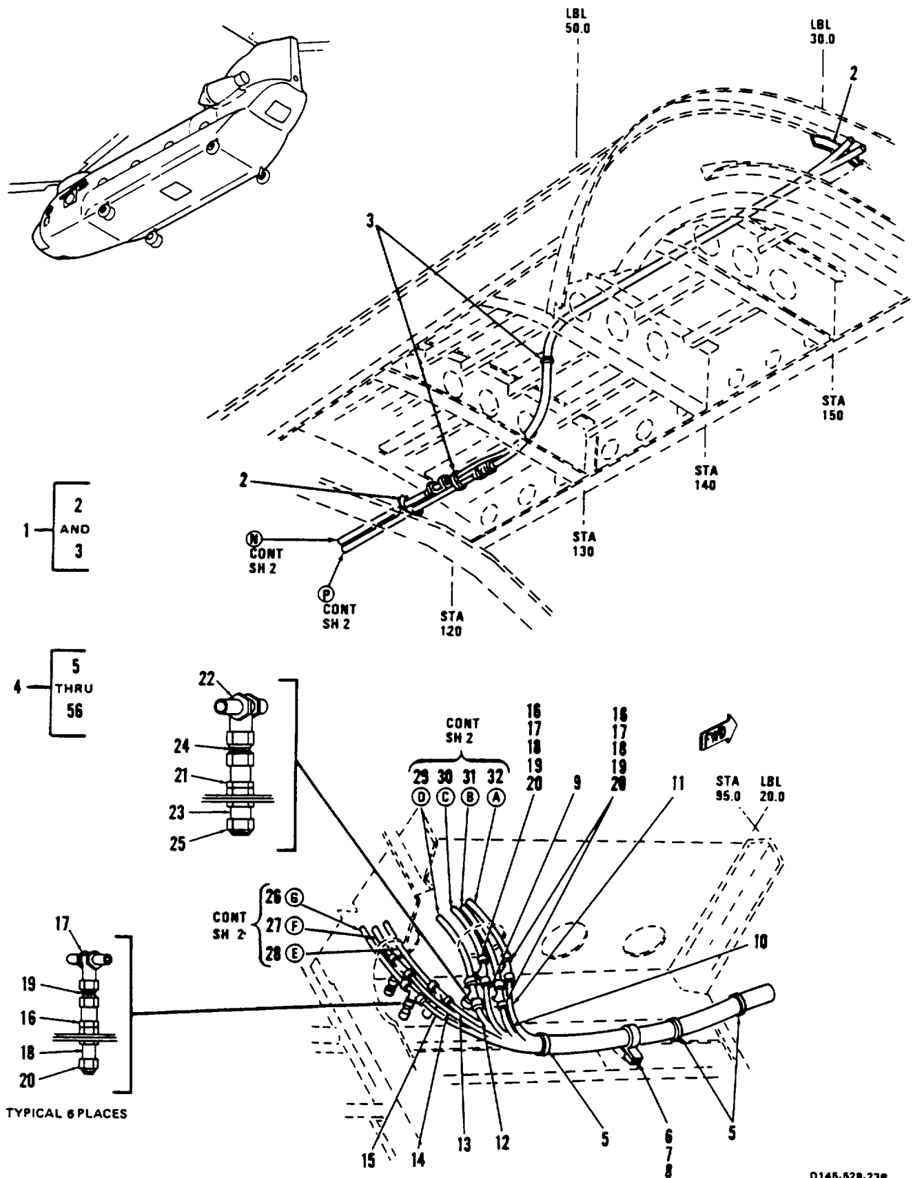
Figure 296. Tubing Instl, Equipment, Crown Panel and Side, LH Sta 120 to 160 (Sheet 1 of 3)
