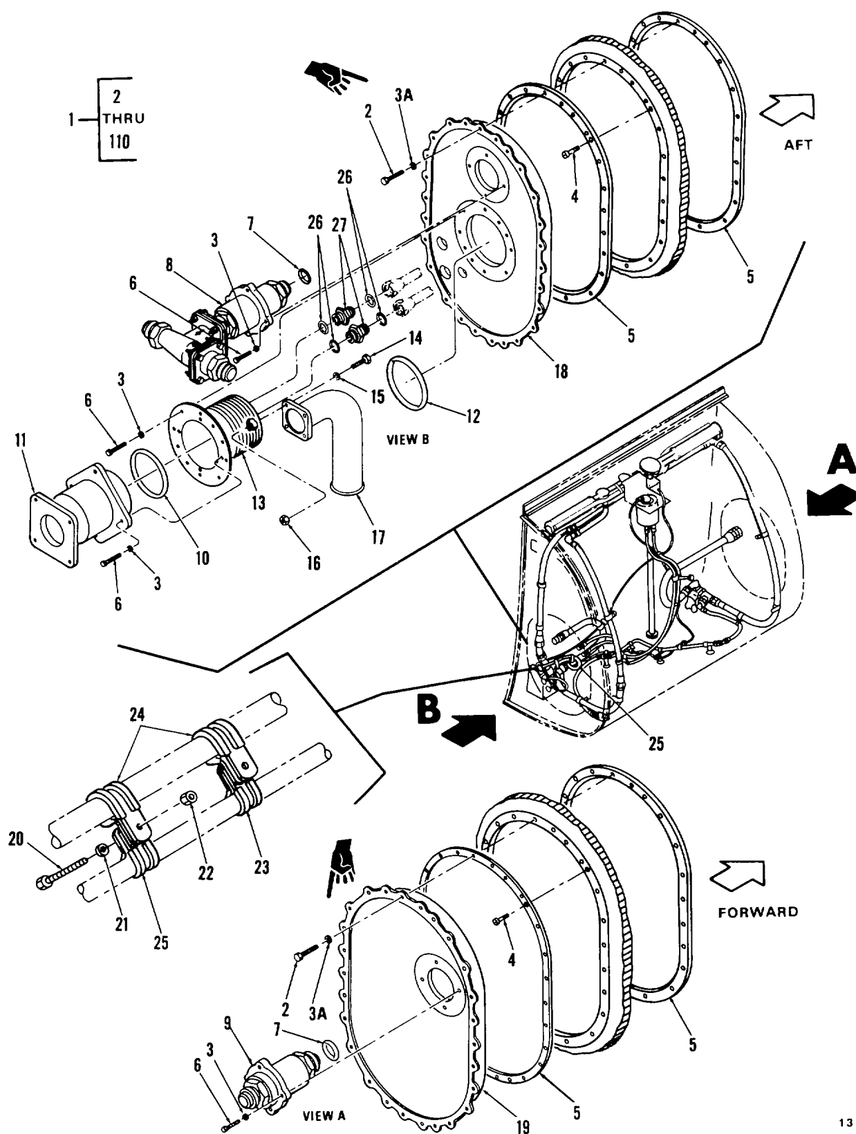
Figure 346. Fuel Cell, Aft Auxiliary (Sheet 1 of 6)
