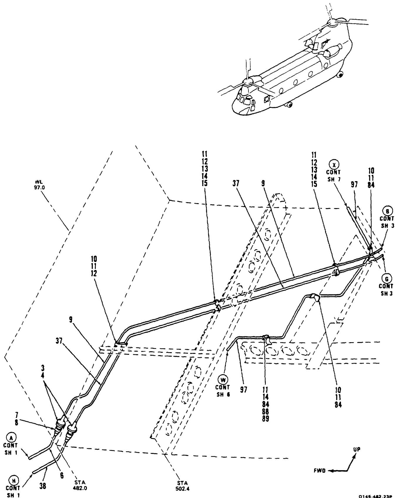
Figure 273. Tubing Instl, Aft Pylon , and Combing Transmission Area (Sheet 2 of 7)
