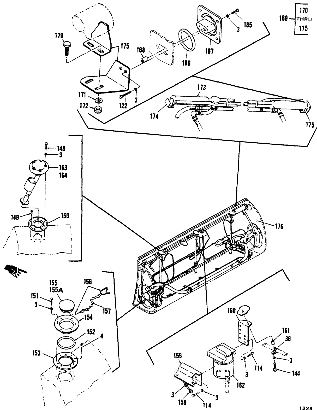
Figure 345. Fuel Cell, Main (Sheet 8 of 8)
