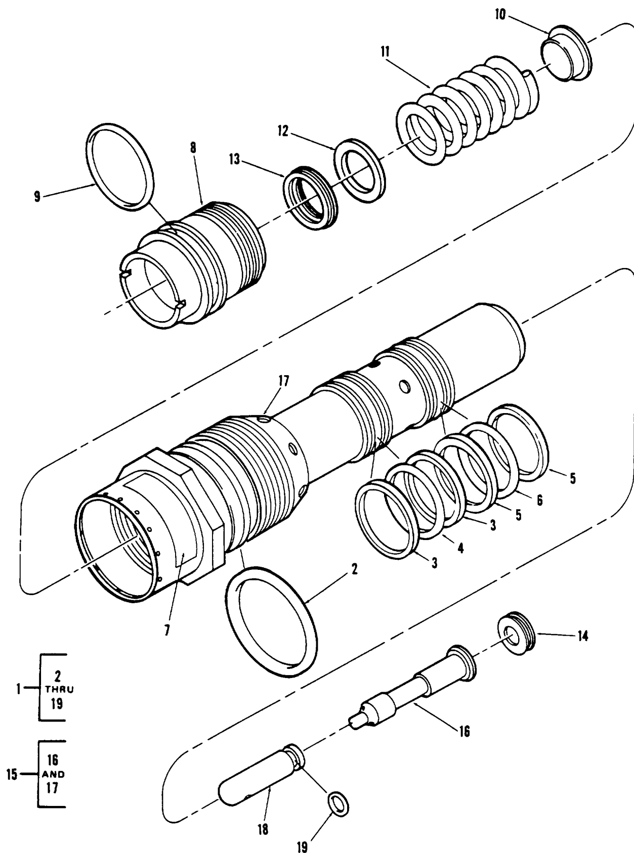
Figure 205. Reducer, Pressure 60610
