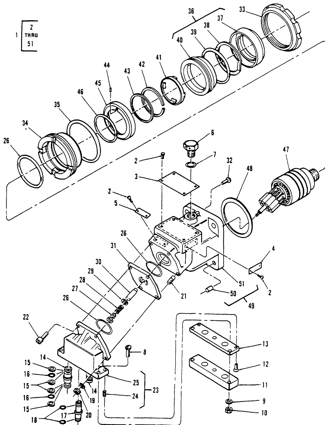
Figure 221. Motor, Hydraulic
