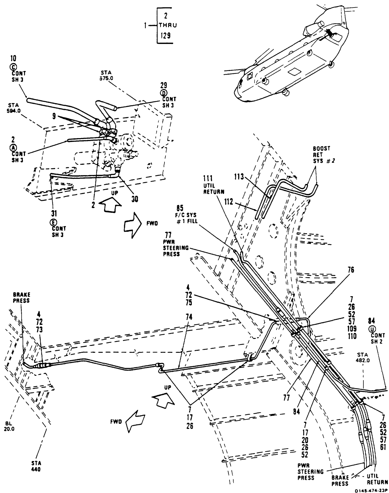
Figure 270. Tubing Instl, Hydraulic, Aft Crown Panel, RH Sta 440 to 594 (Sheet 1 of 4)
