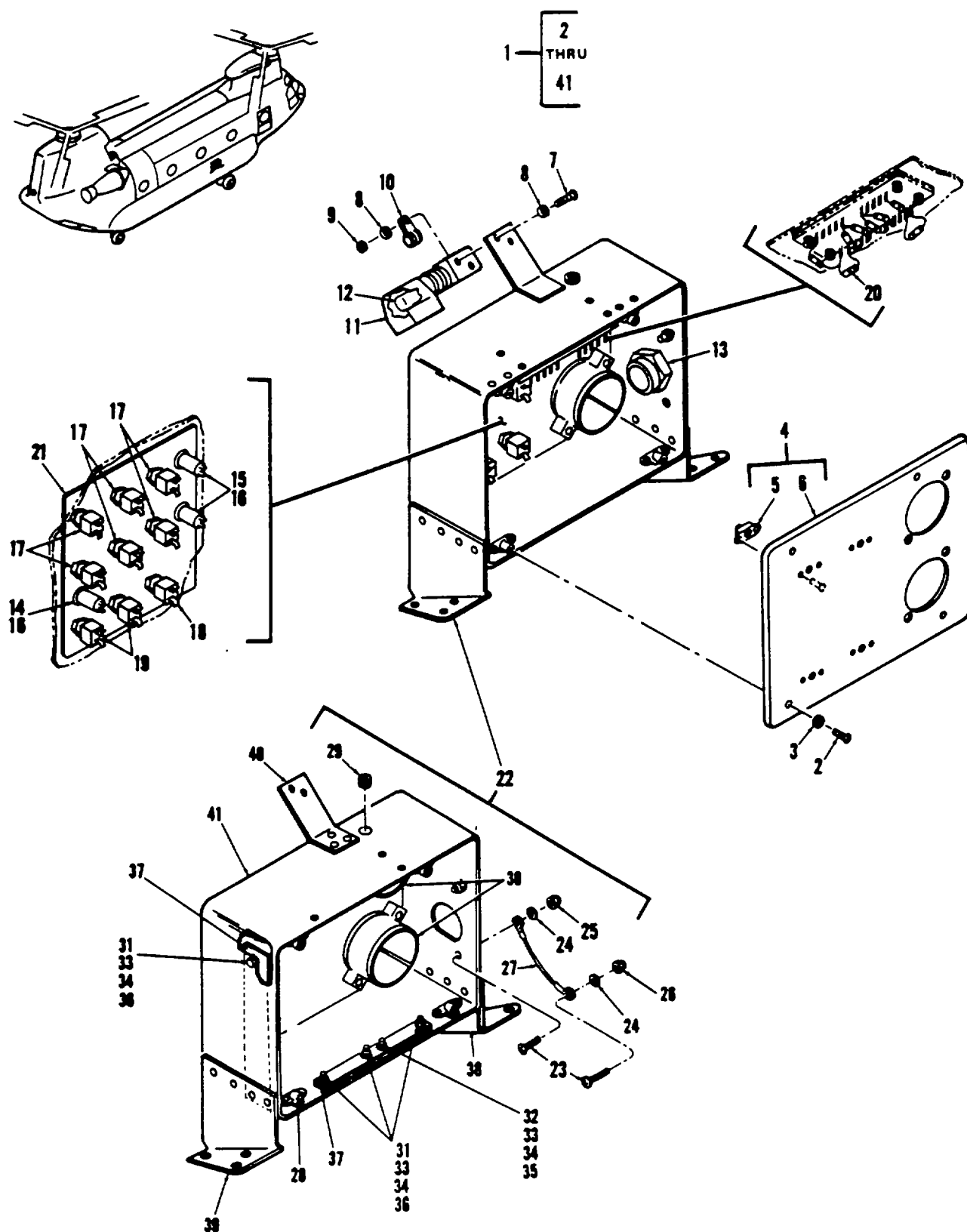
Figure 329. Panel, Precheck
