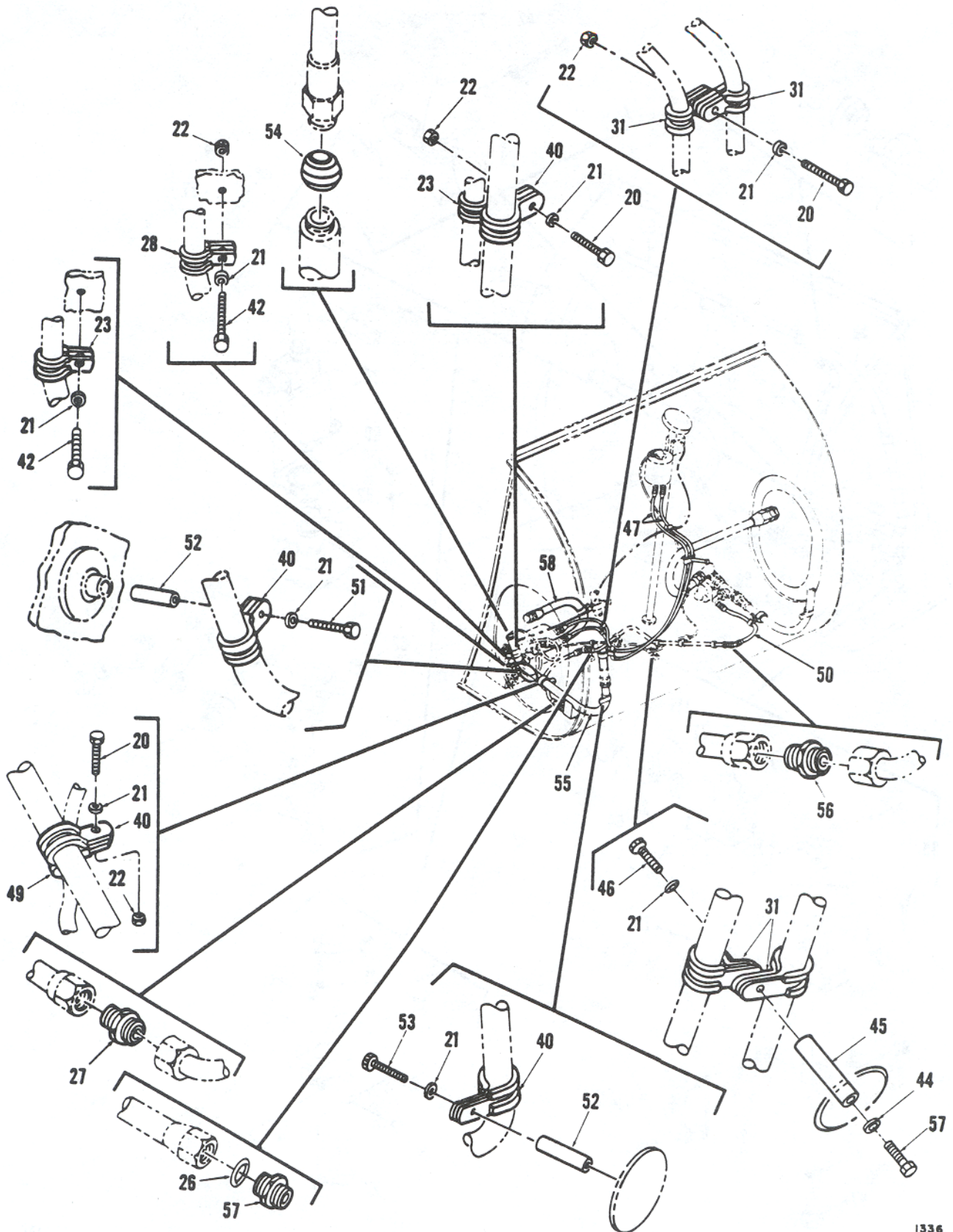
Figure 346. Fuel Cell, Aft Auxiliary (Sheet 3 of 6).
