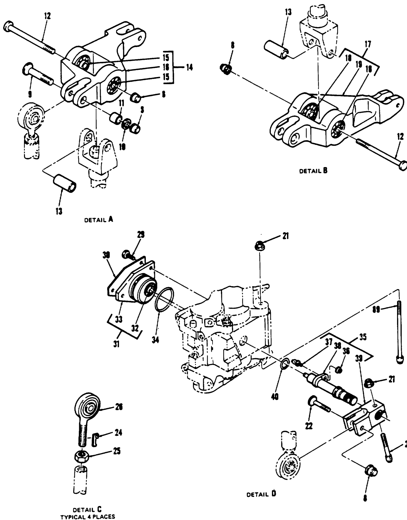
Figure 245. Actuator, Pitch Axis (Sheet 2 of 5)
