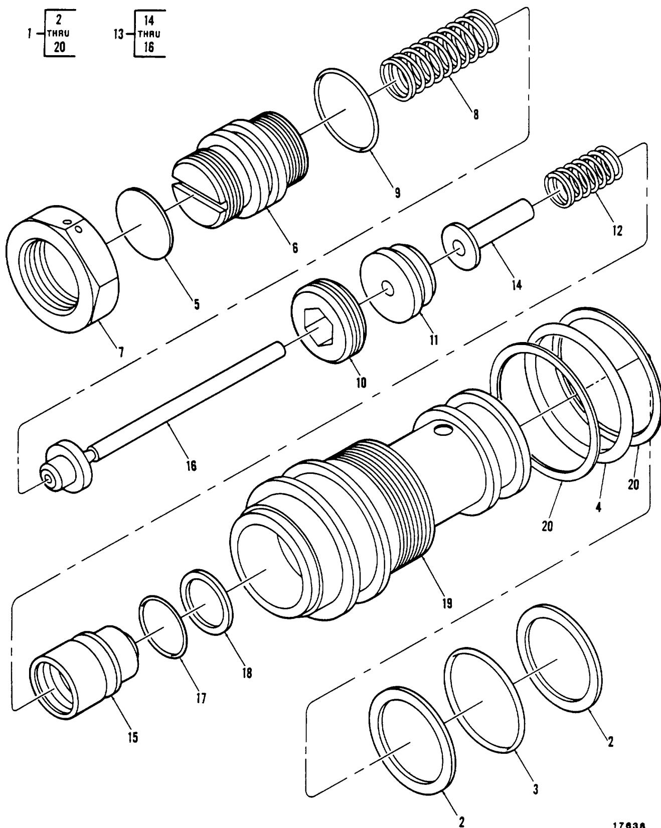
Figure 226. Valve, Relief, Pressure
