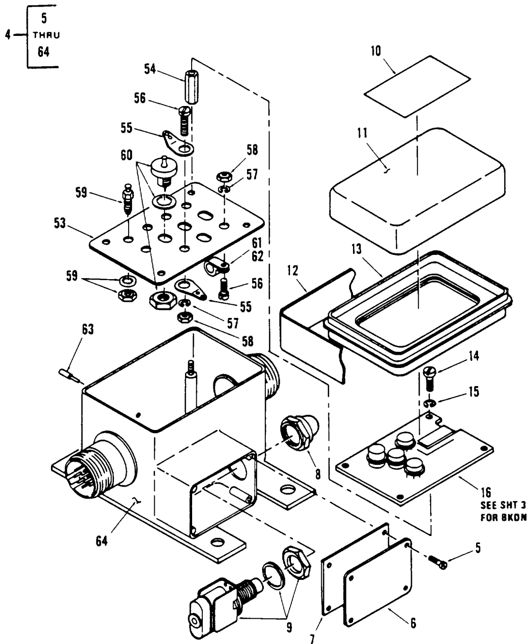
Figure 285. Signal Conditioner Instl, Fwd Pylon CGI (Sheet 2 of 3)
