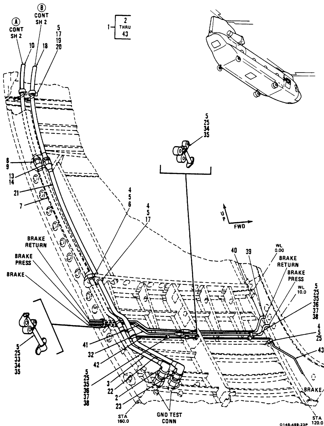
Figure 265. Tubing Instl, Hydraulic, Crown Panel and Side, LH, Sta 120 to 160 (Sheet 2 of 2)
