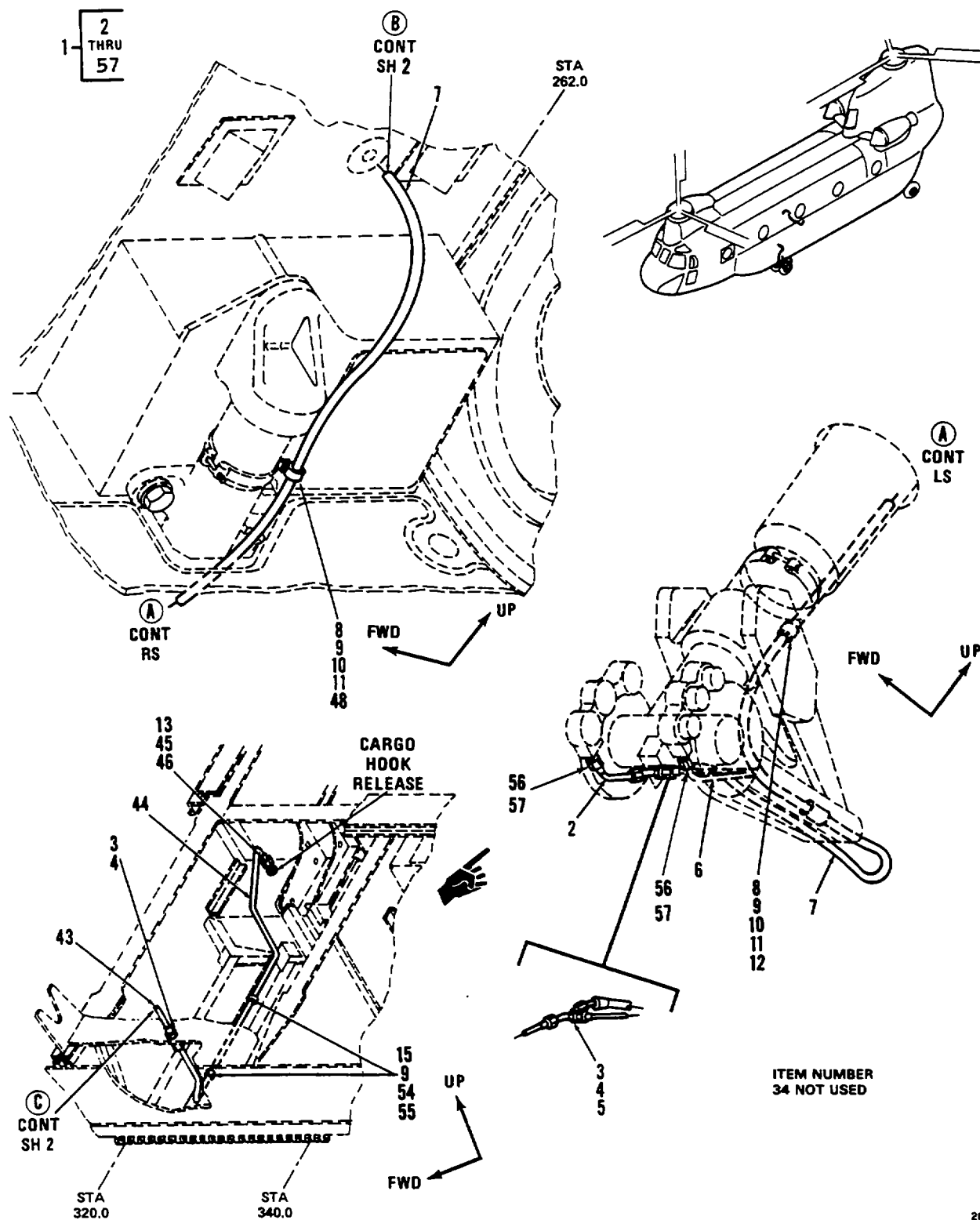
Figure 263. Tubing Instl, Hydraulic, Cabin Ceiling and Side, Lower, LH, Sta 160 to 440 (Sheet 1 of 2)
