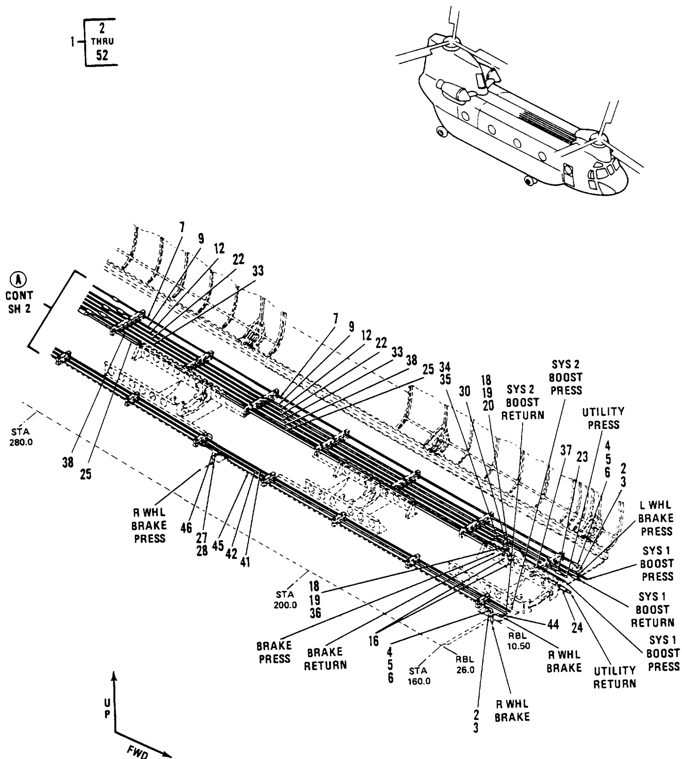
Figure 266. Tubing Instl, Hydraulic, Cabin Crown Panel and Tunnel, Sta 160 to 440 (Sheet 1 of 2)
