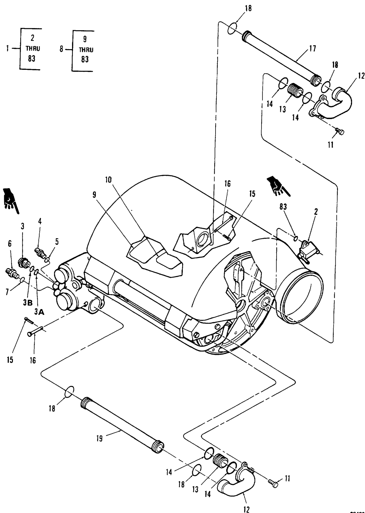
Figure 217. Reservoir / Cooler 1711019-002 (Sheet 1 of 3)
