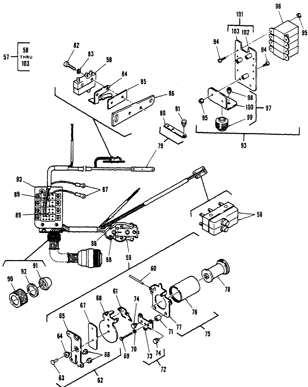
Figure 311. Light Instl, Landing and Search (Sheet 3 of 5)
