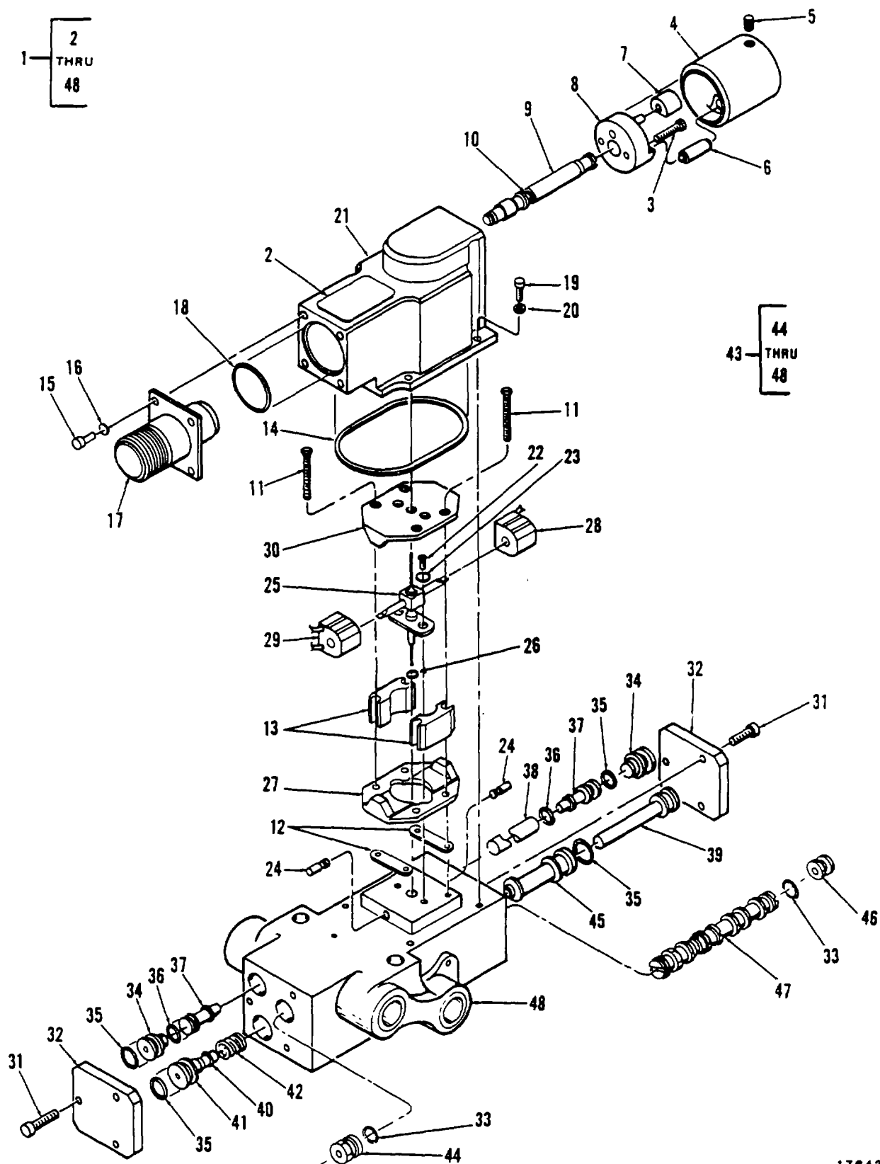
Figure 238. Valve, Hoist Control A23772-001
