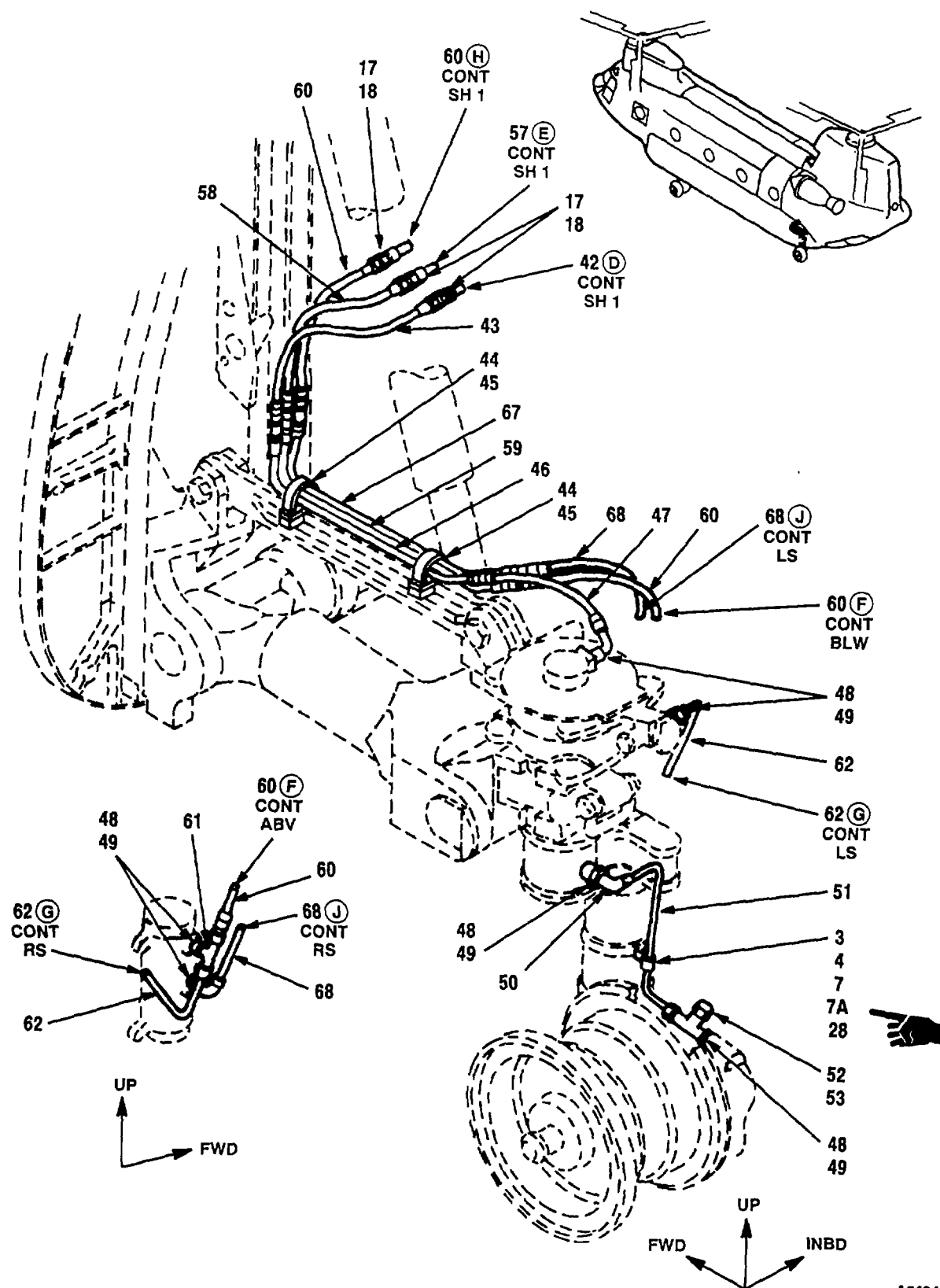
Figure 267. Tubing Instl, Lower Aft Fuselage, Sta 440 to 594 (Sheet 3 of 3)
