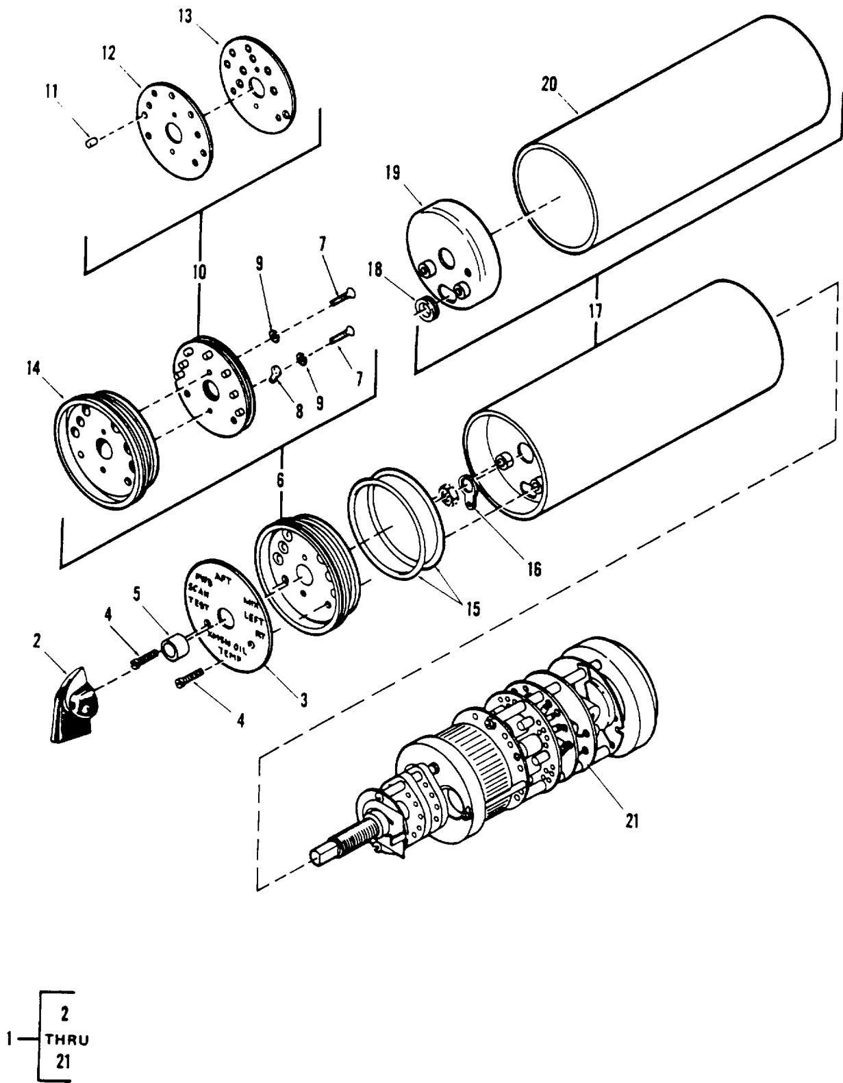
Figure 281. Switch, Rotary, Oil Temperature
