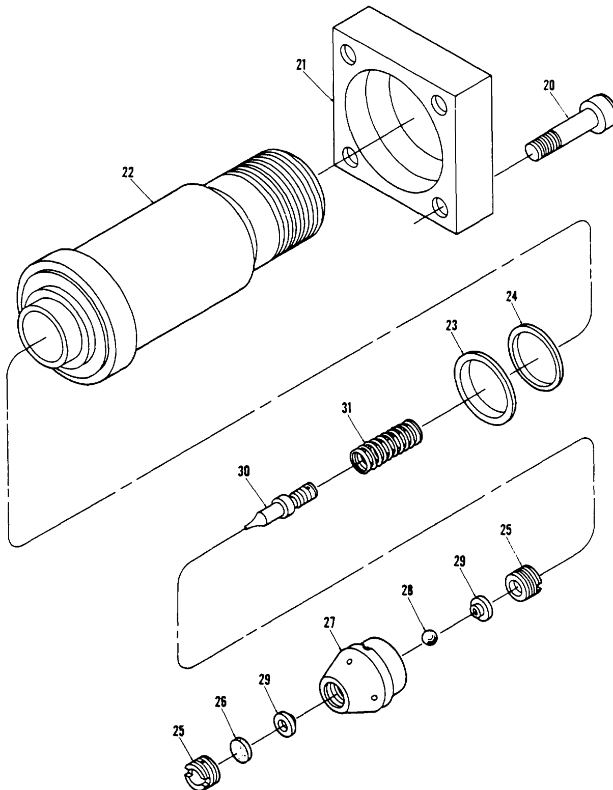
Figure 204. Valve, Solenoid HP1322100-6 (Sheet 2 of 4)
