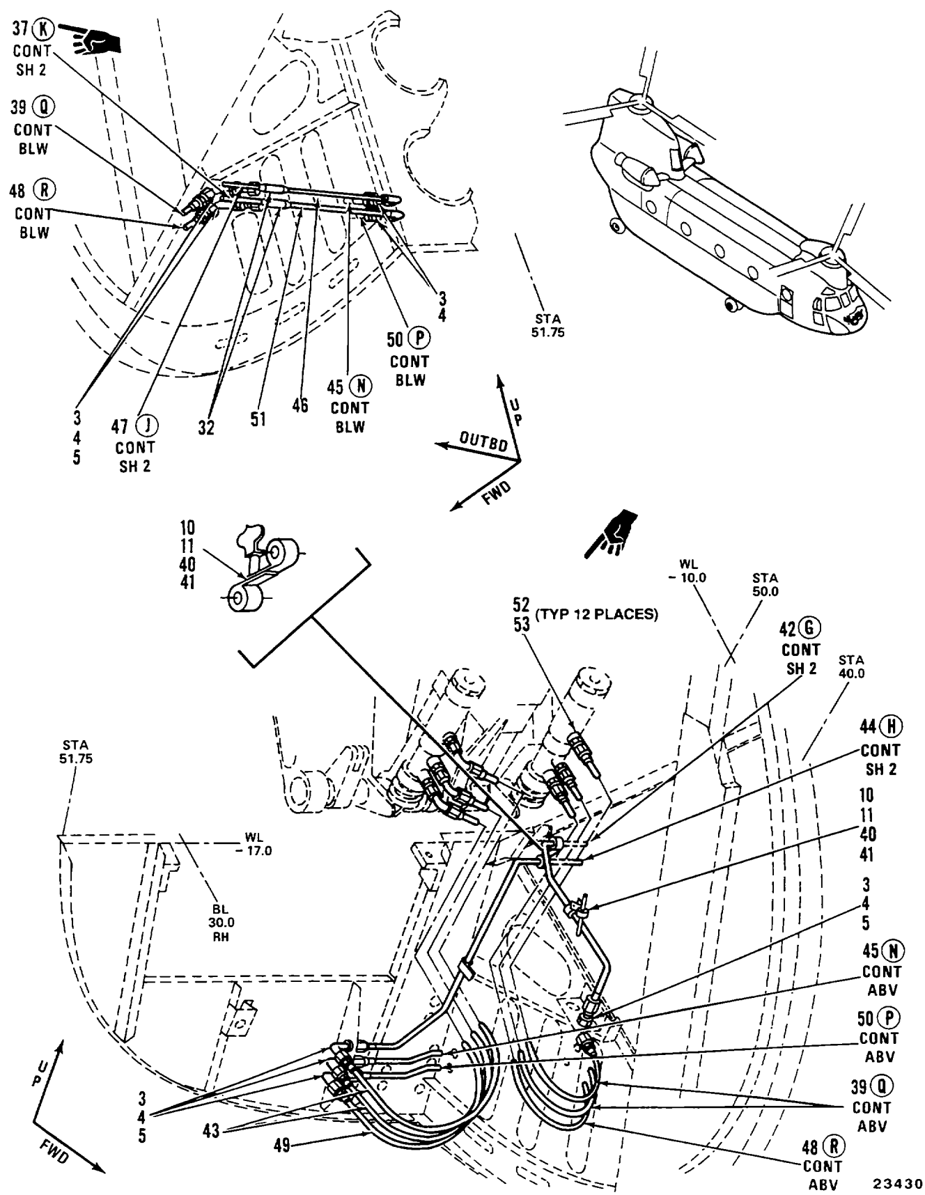
Figure 258. Tubing Instl, Hydraulic, Nose Compartment Sta 0 to 52 (Sheet 3 of 3)
