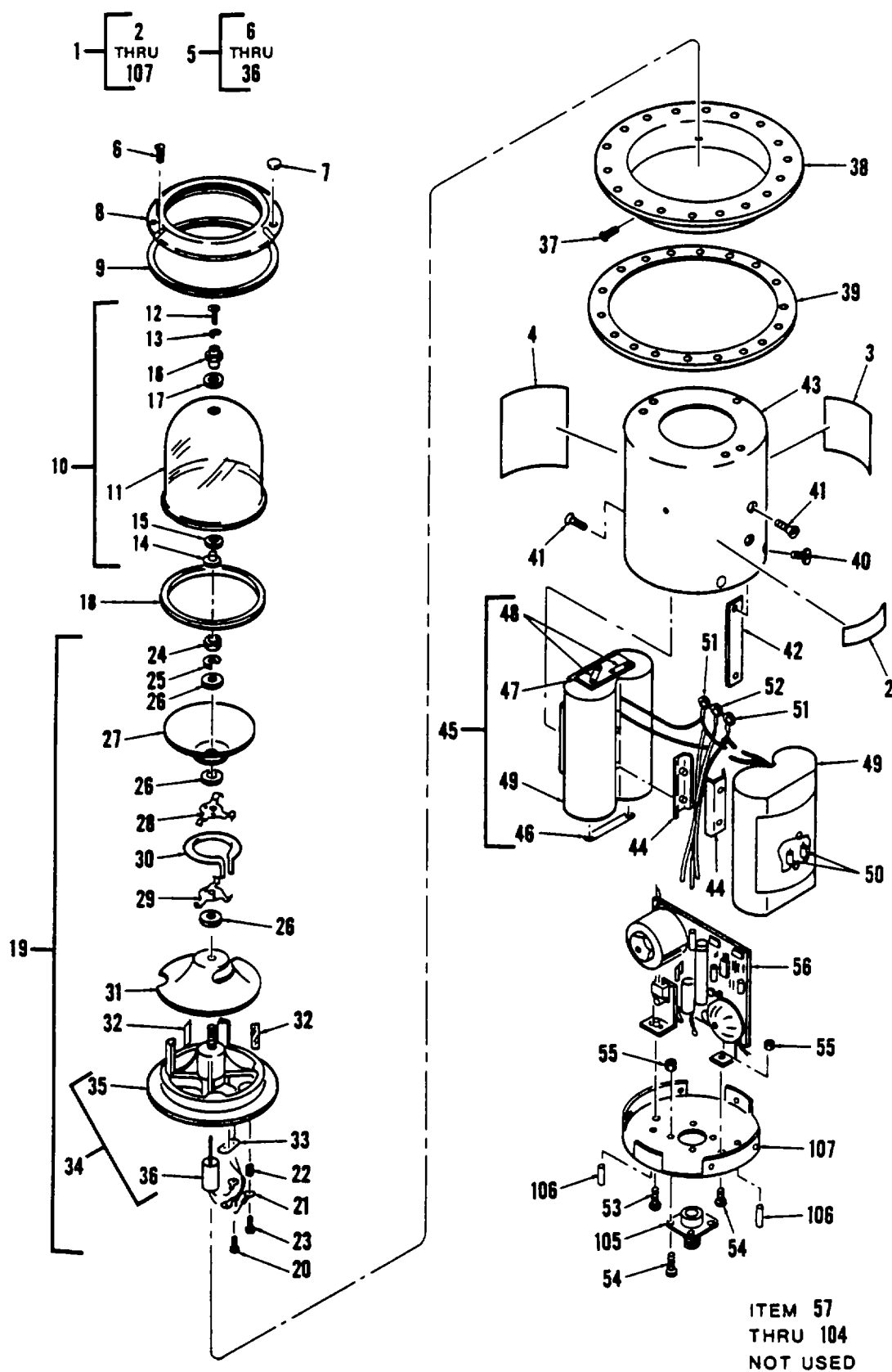
Figure 330. Light, Anticollision
