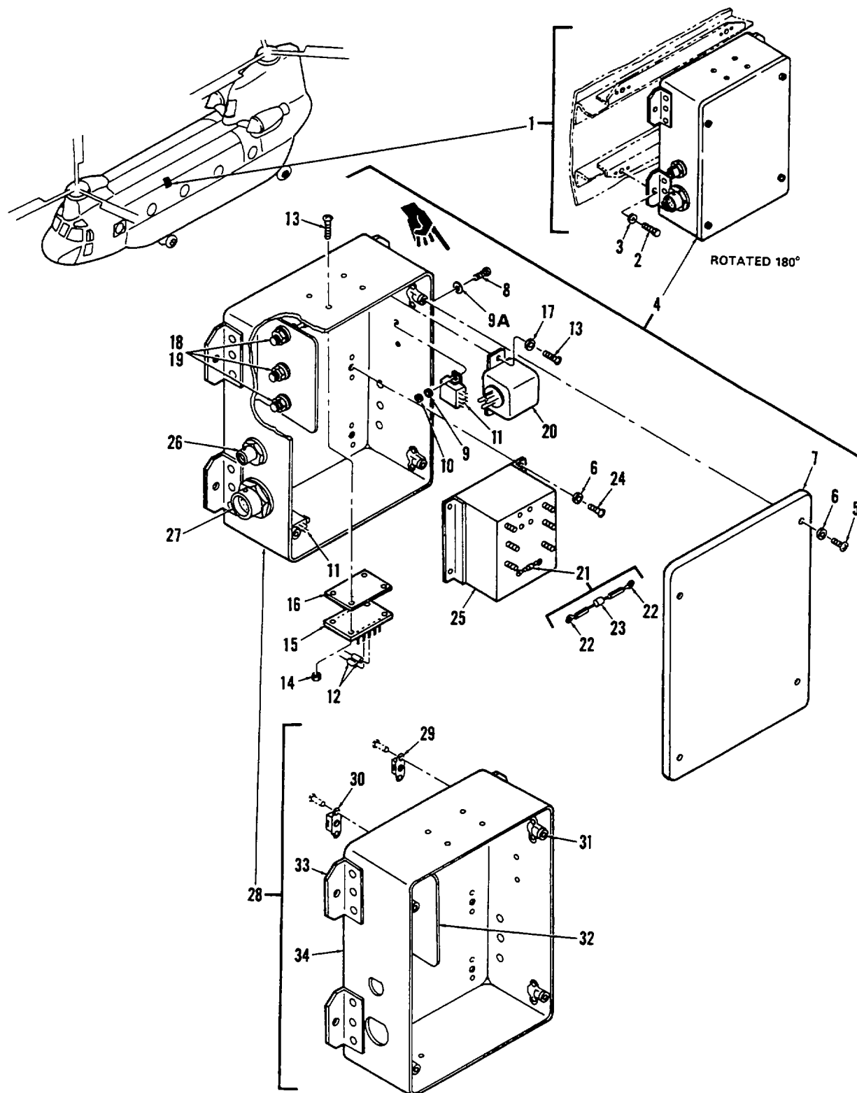
Figure 324. Box Instl, Relay, Emergency Hook Release
