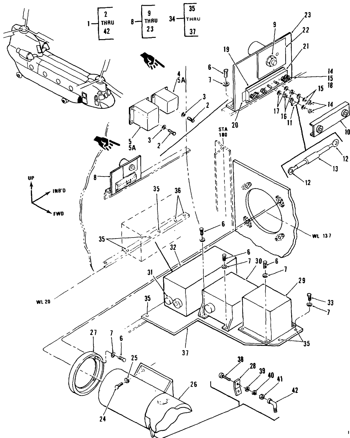
Figure 319. Equipment Installation, R.H. Pod, Electrical
