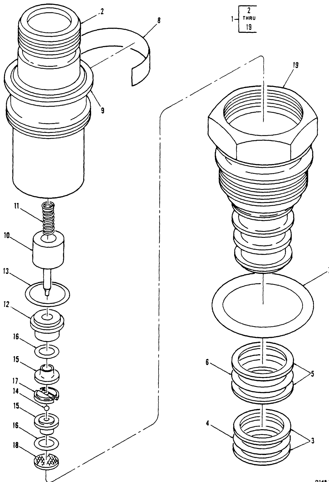
Figure 225. Valve, Solenoid, Cartridge 60740-10
