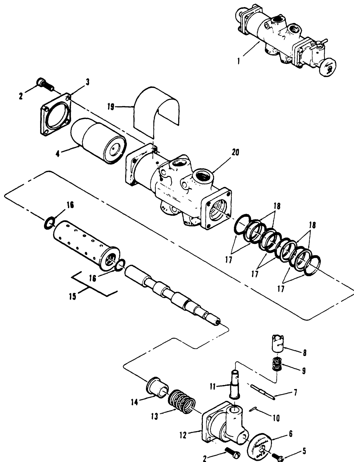
Figure 213. Valve, Sequence, Ramp Door
