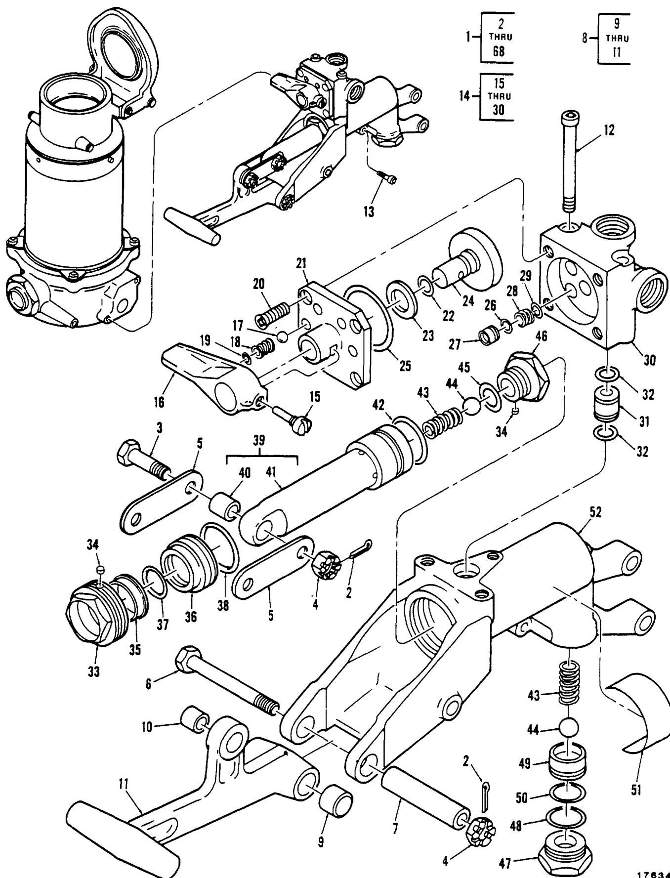
Figure 211. Fill Module, Hyd Pump (Sheet 1 of 2)
