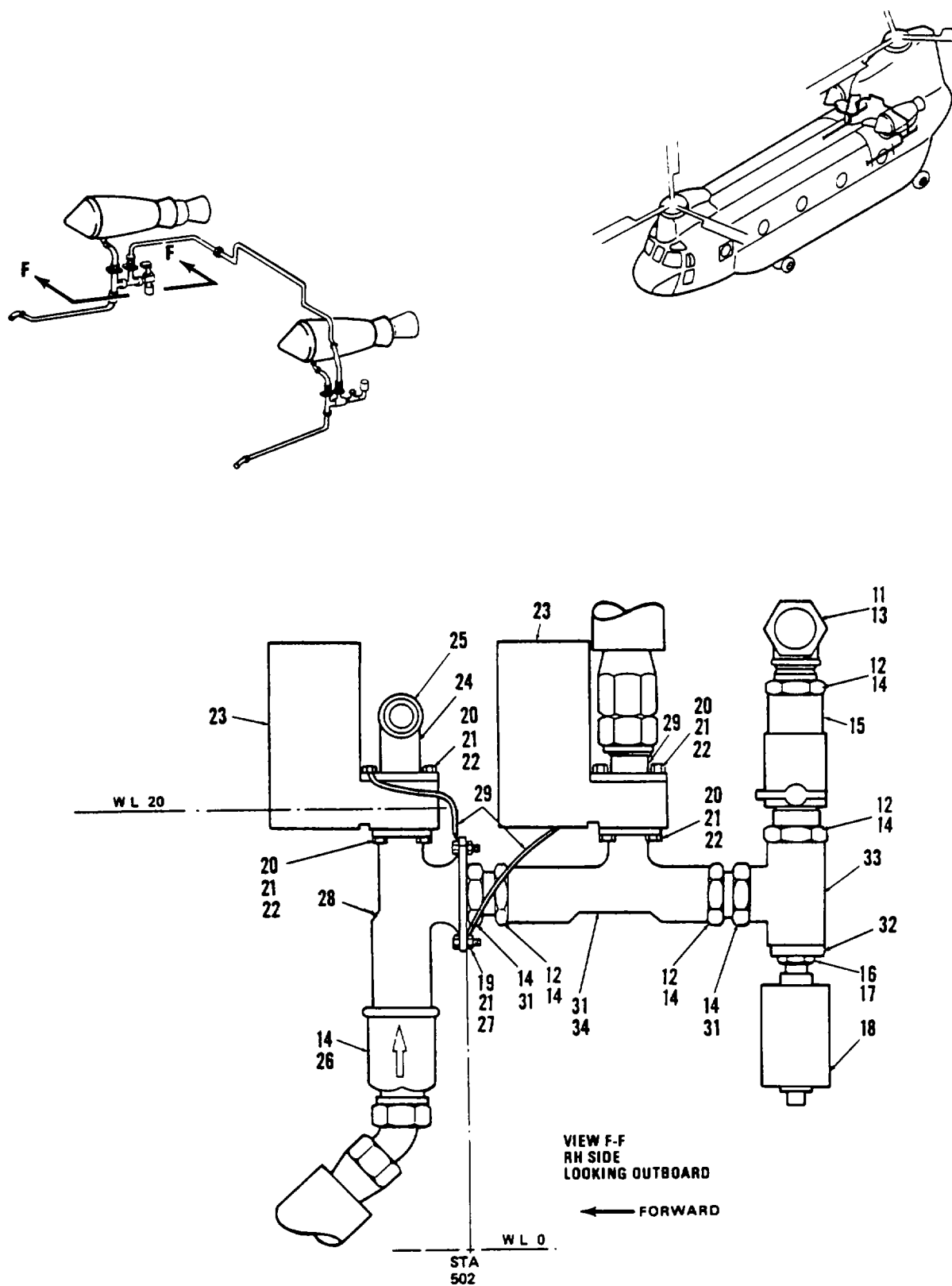
Figure 351. Plumbing Instl, Fuel, Fuselage (Sheet 2 of 5)
