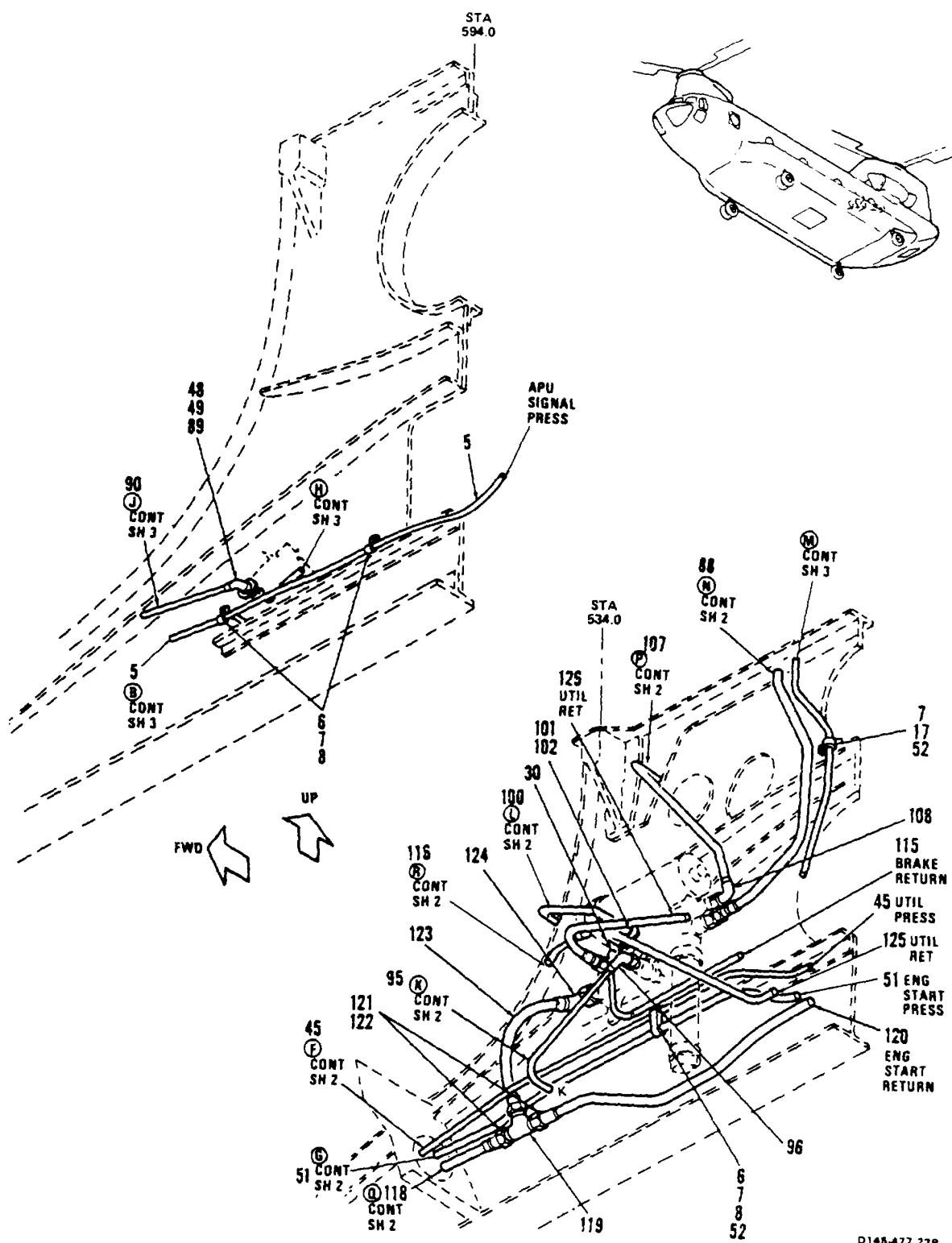
Figure 270. Tubing Instl, Hydraulic, Aft Crown Panel, RH Sta 440 to 594 (Sheet 4 of 4)
