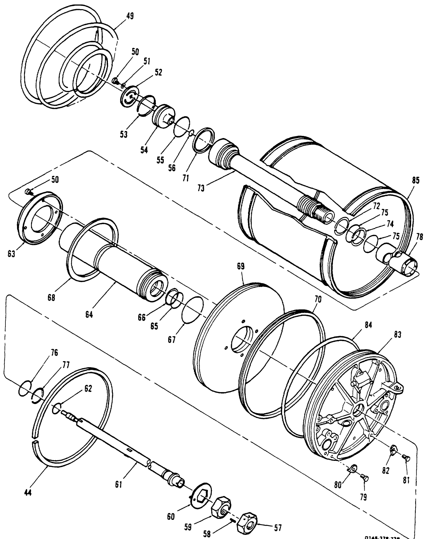
Figure 216. Reservoir/Cooler 1711018-002 (Sheet 3 of 3)
