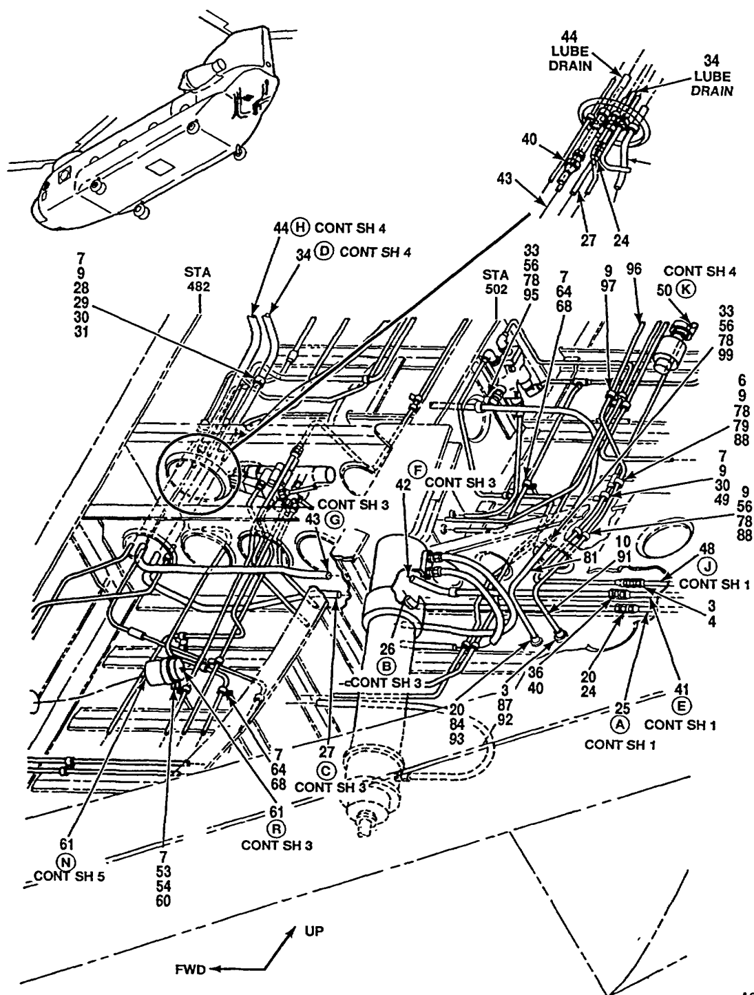
Figure 357. Tubing Instl, Aft Fuselage (Sheet 2 of 5)
