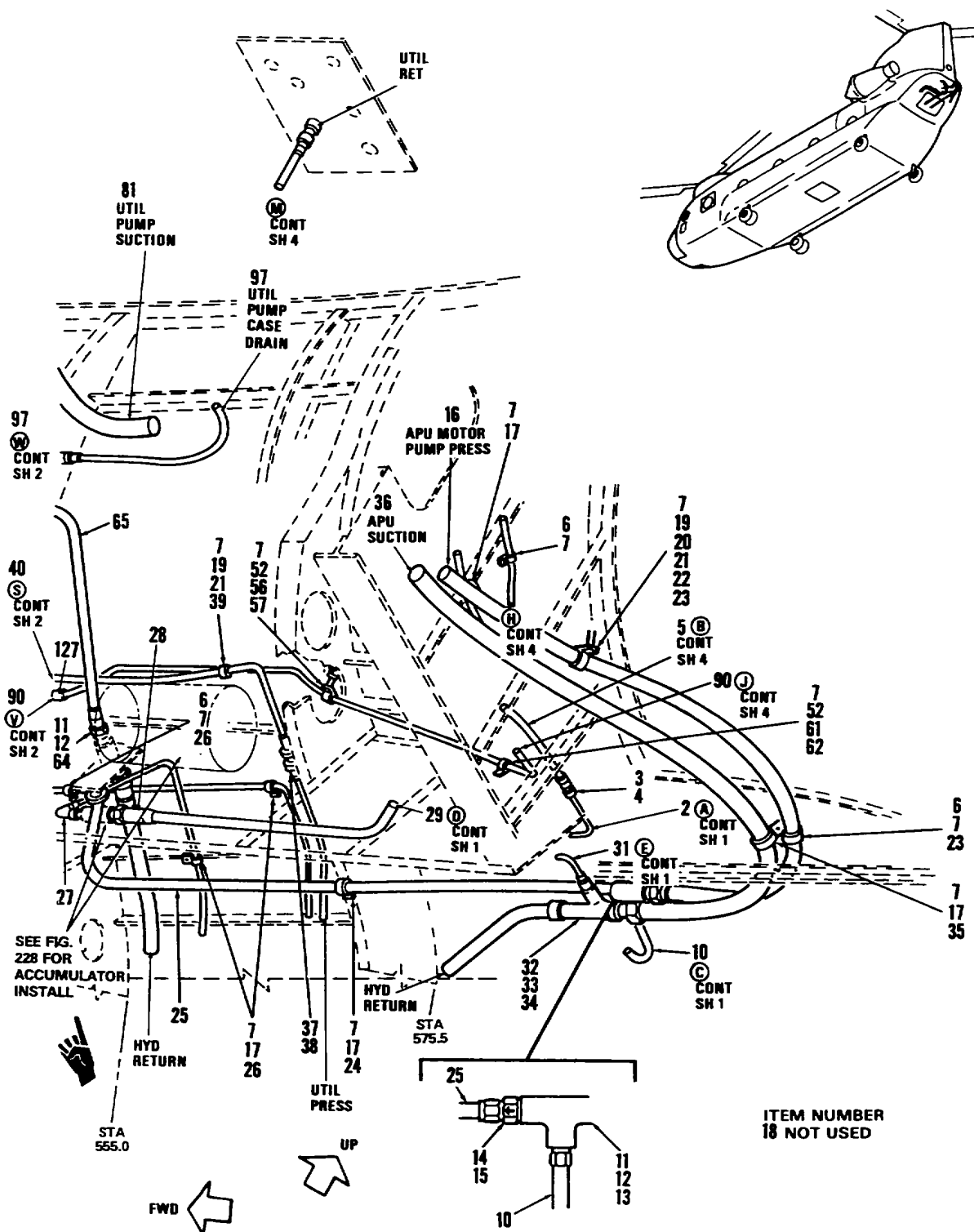
Figure 270. Tubing Instl, Hydraulic, Aft Crown Panel, RH Sta 440 to 594 (Sheet 3 of 4)
