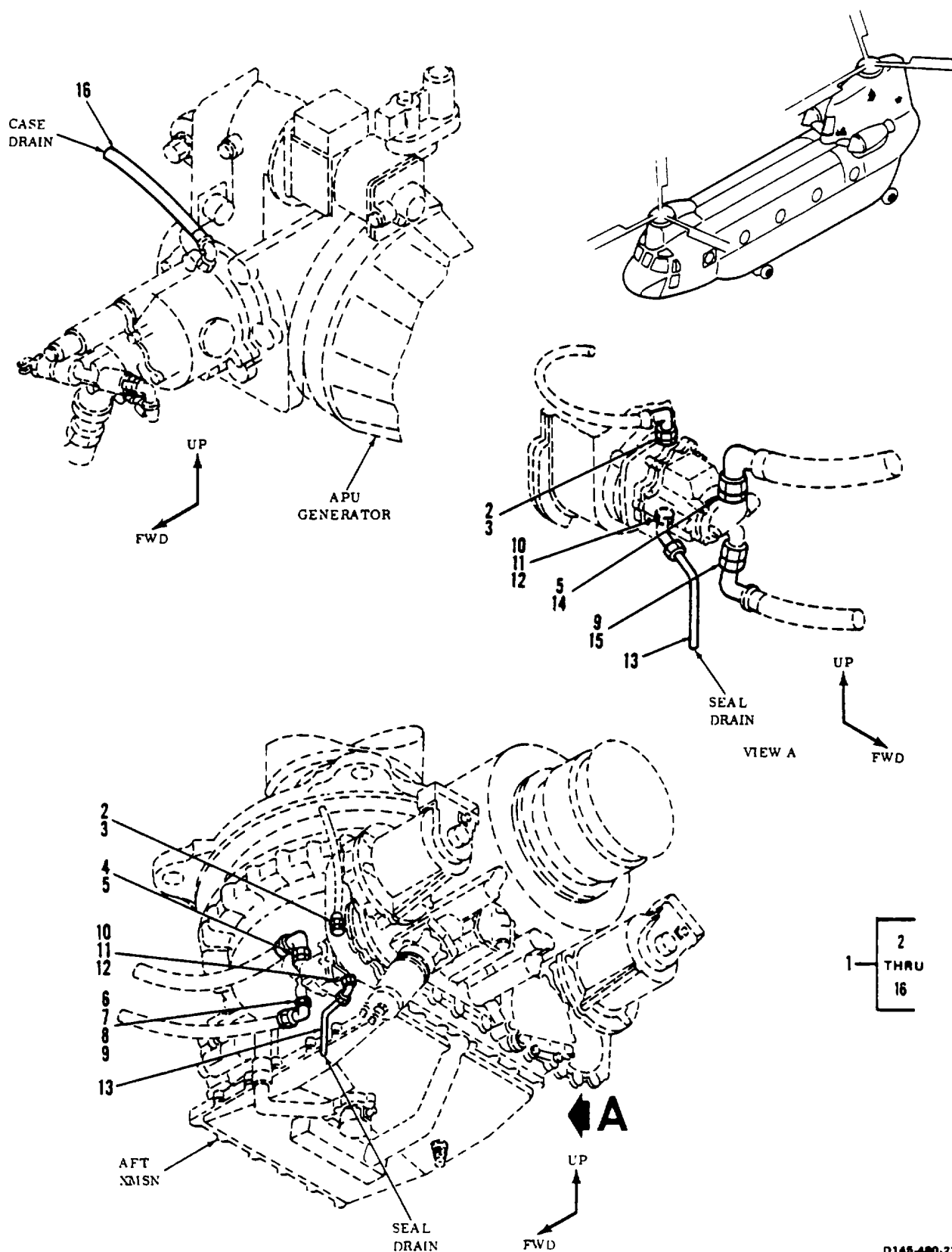
Figure 272. Tubing Instl, Hydraulic, Aft Transmission and APU
