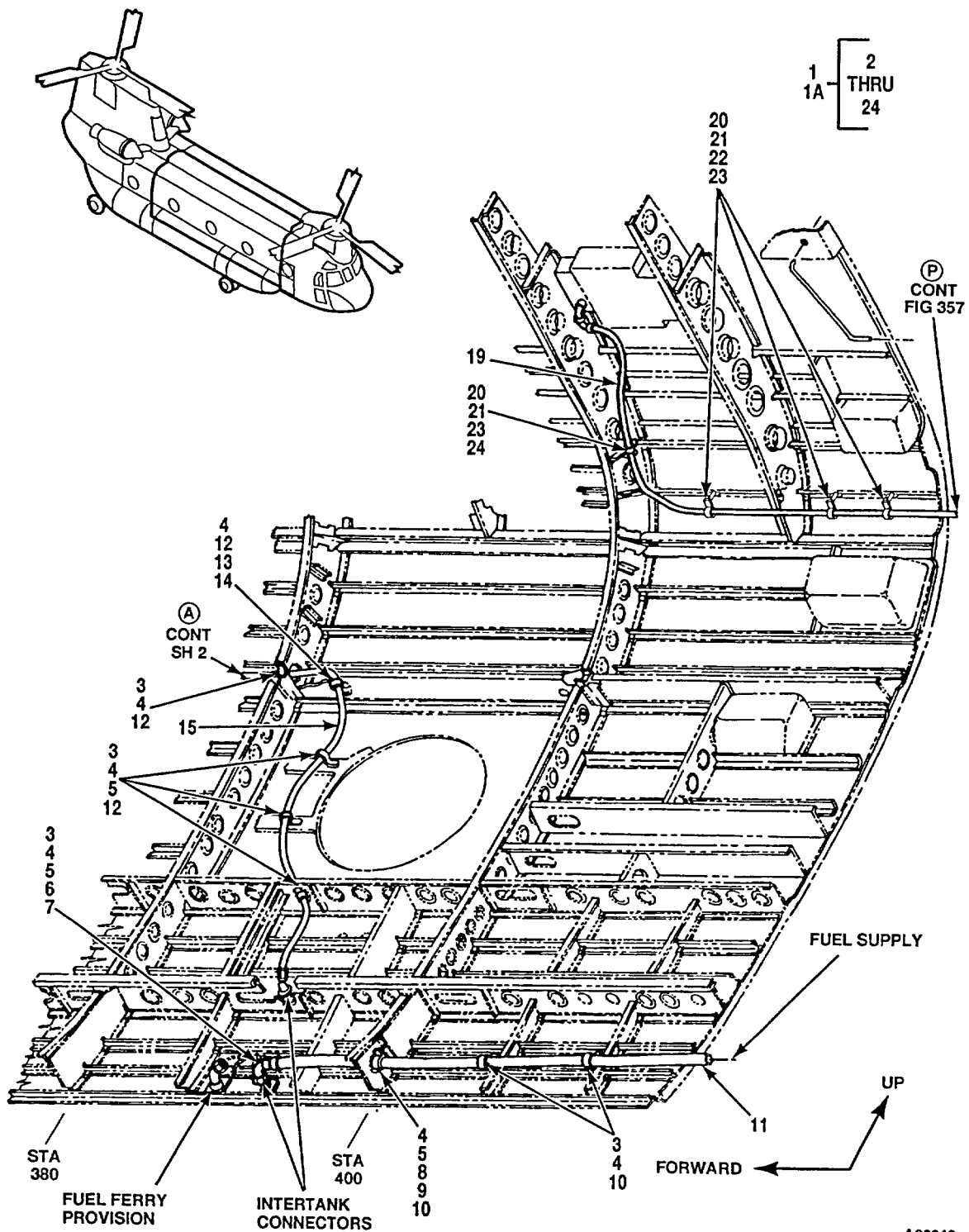
Figure 355. Tubing Instl, Crown, Sta 160 (Sheet 1 of 3)
