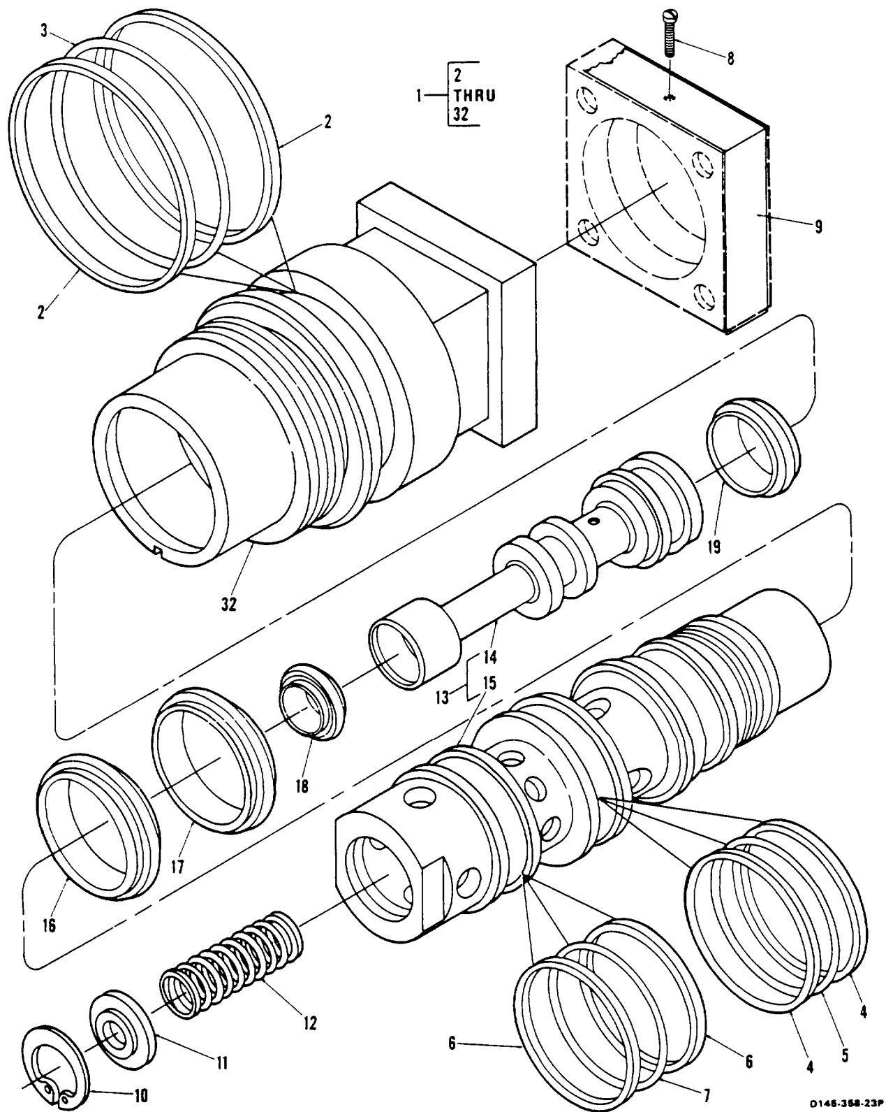
Figure 204. Valve, Solenoid HP1322100-6 (Sheet 1 of 4)
