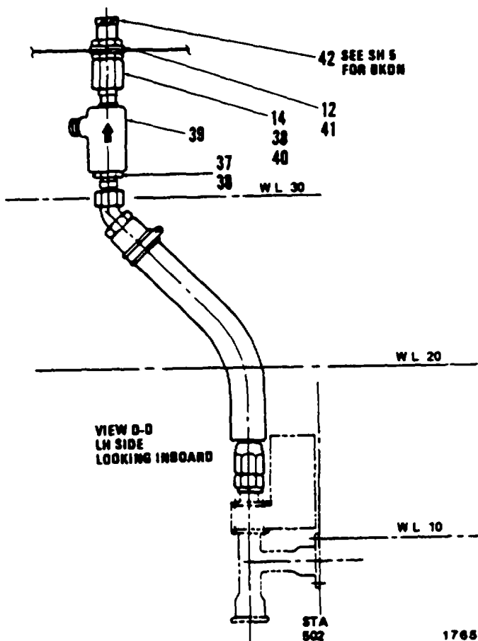
Figure 351. Plumbing Instl, Fuel, Fuselage (Sheet 4 of 5)
