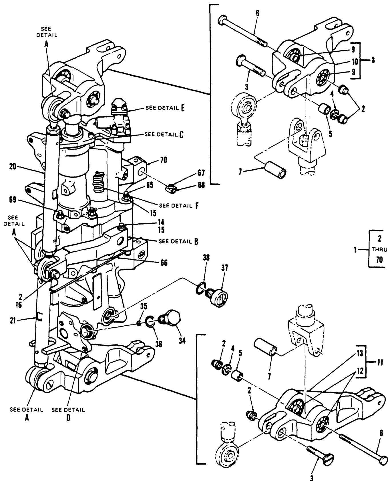
Figure 252. Actuator, Thrust (Sheet 1 of 5)
