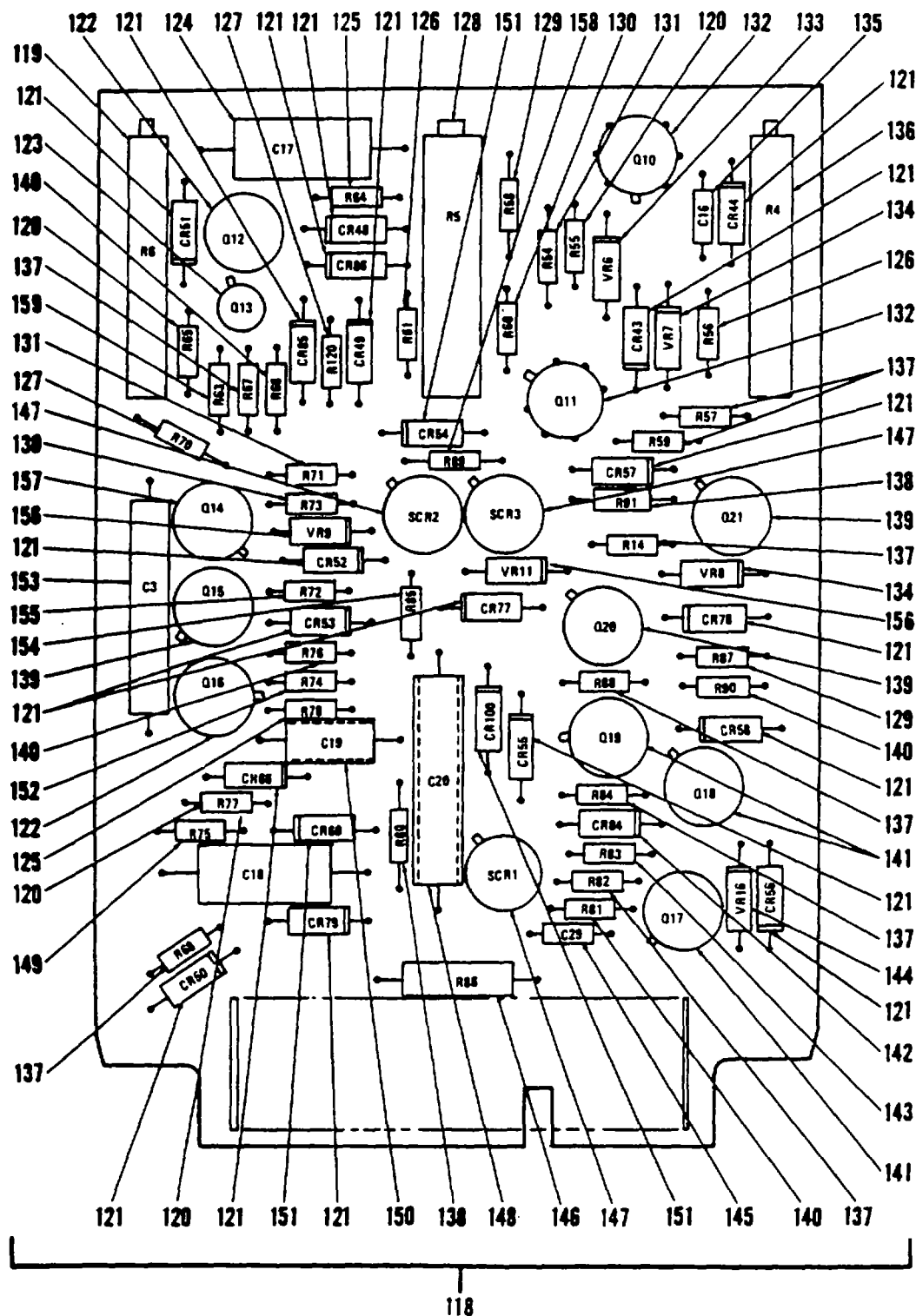
Figure 322. Panel, Generator Control (Sheet 3 of 5)
