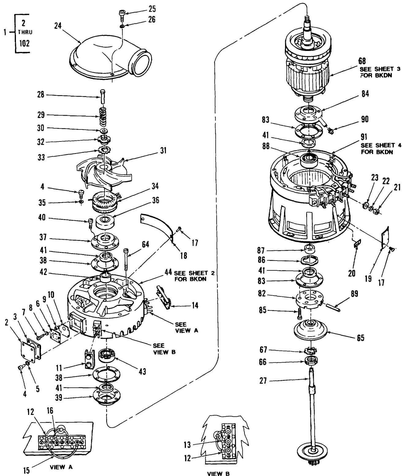
Figure 299A. A.C. Generator Assembly (Sheet 1 of 4)
