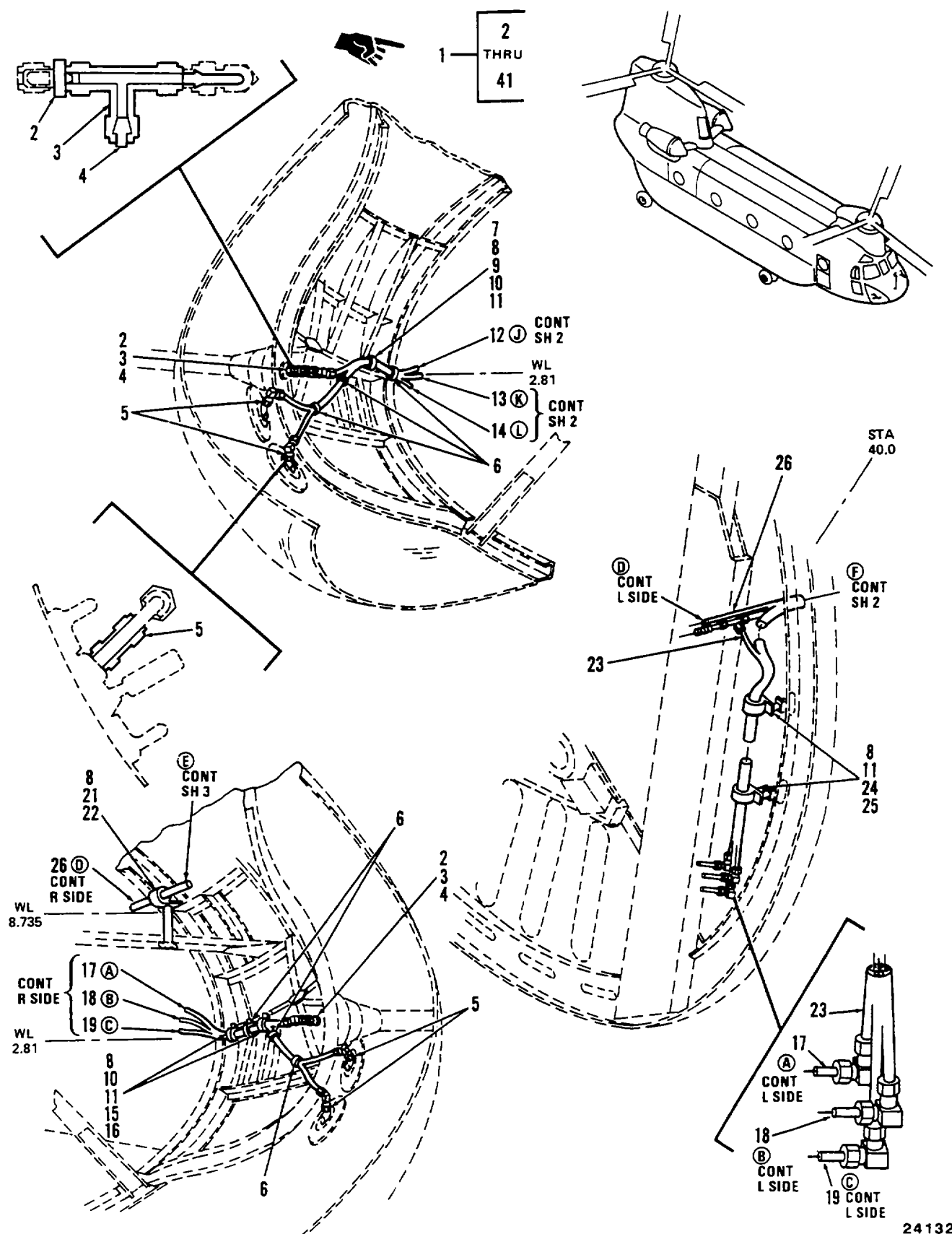
Figure 294. Tubing Instl equipment, Nose Compartment (Sheet 1 of 4)
