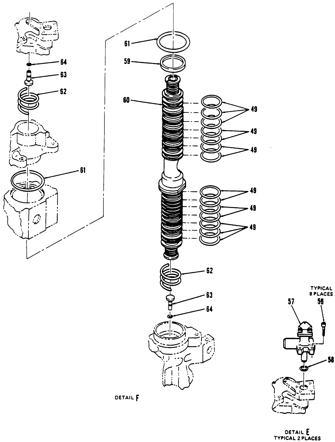
F Figure 252. Actuator, Thrust (Sheet 5 of 5)
