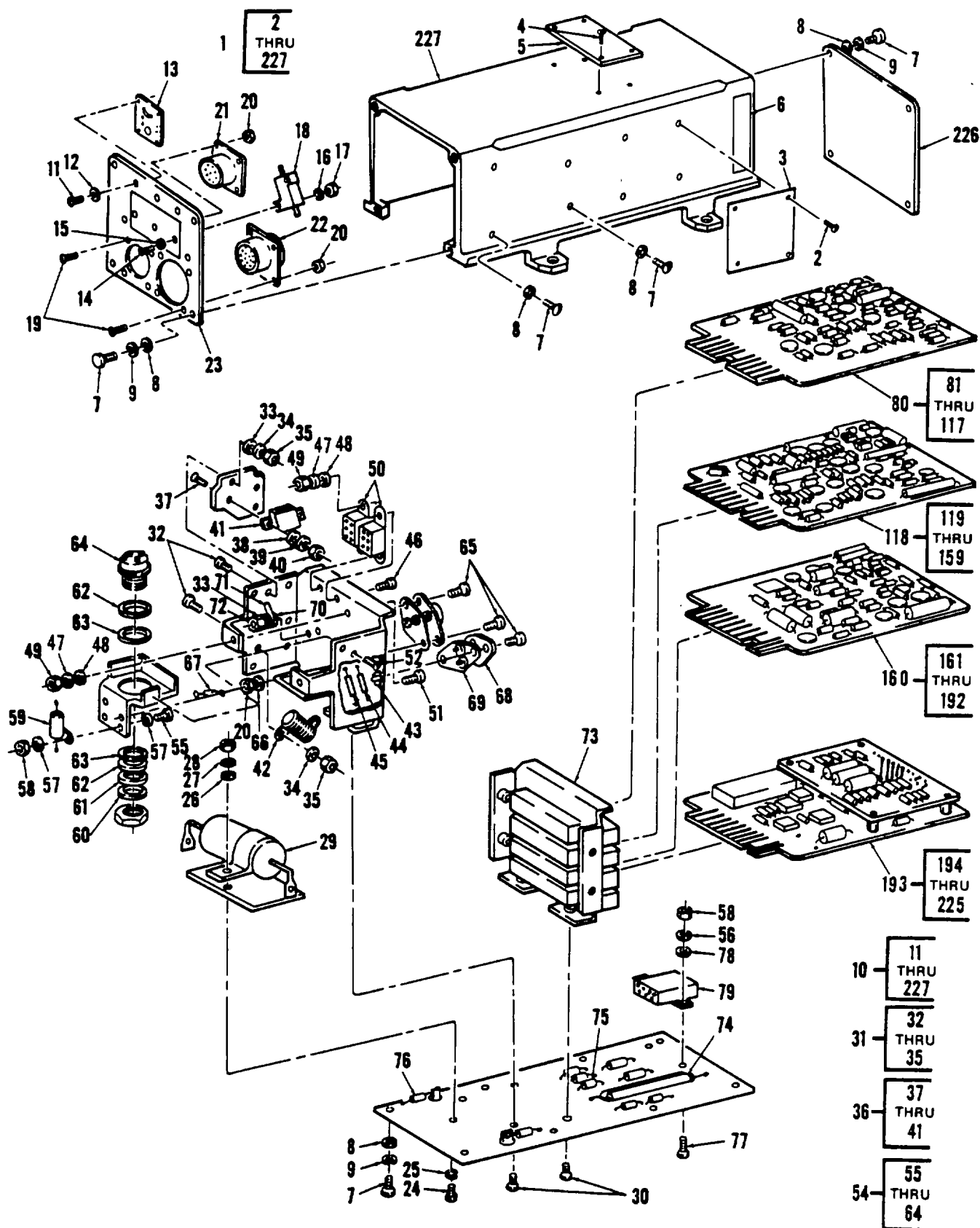
Figure 322. Panel, Generator Control (Sheet 1 of 5)
