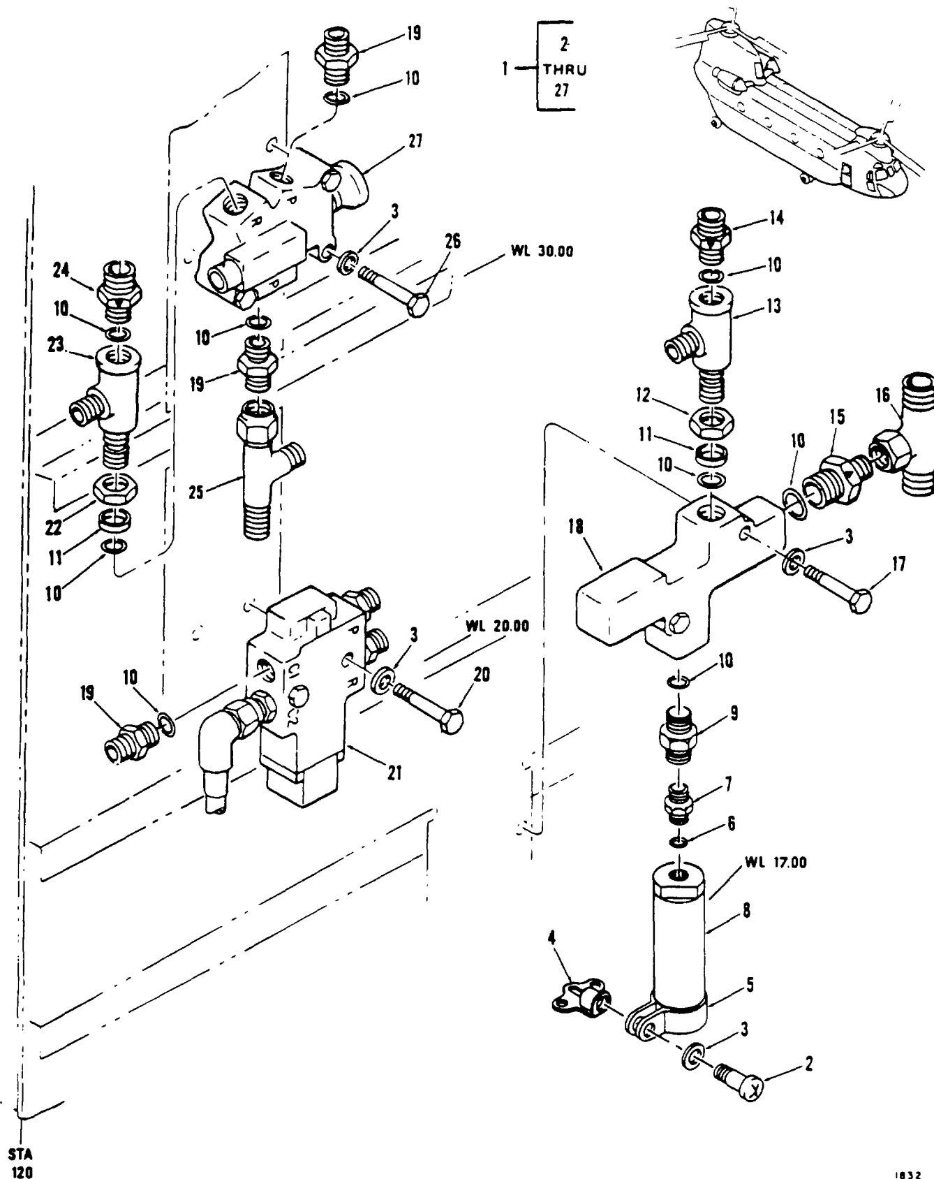
Figure 236. Winch Instl, Rescue
