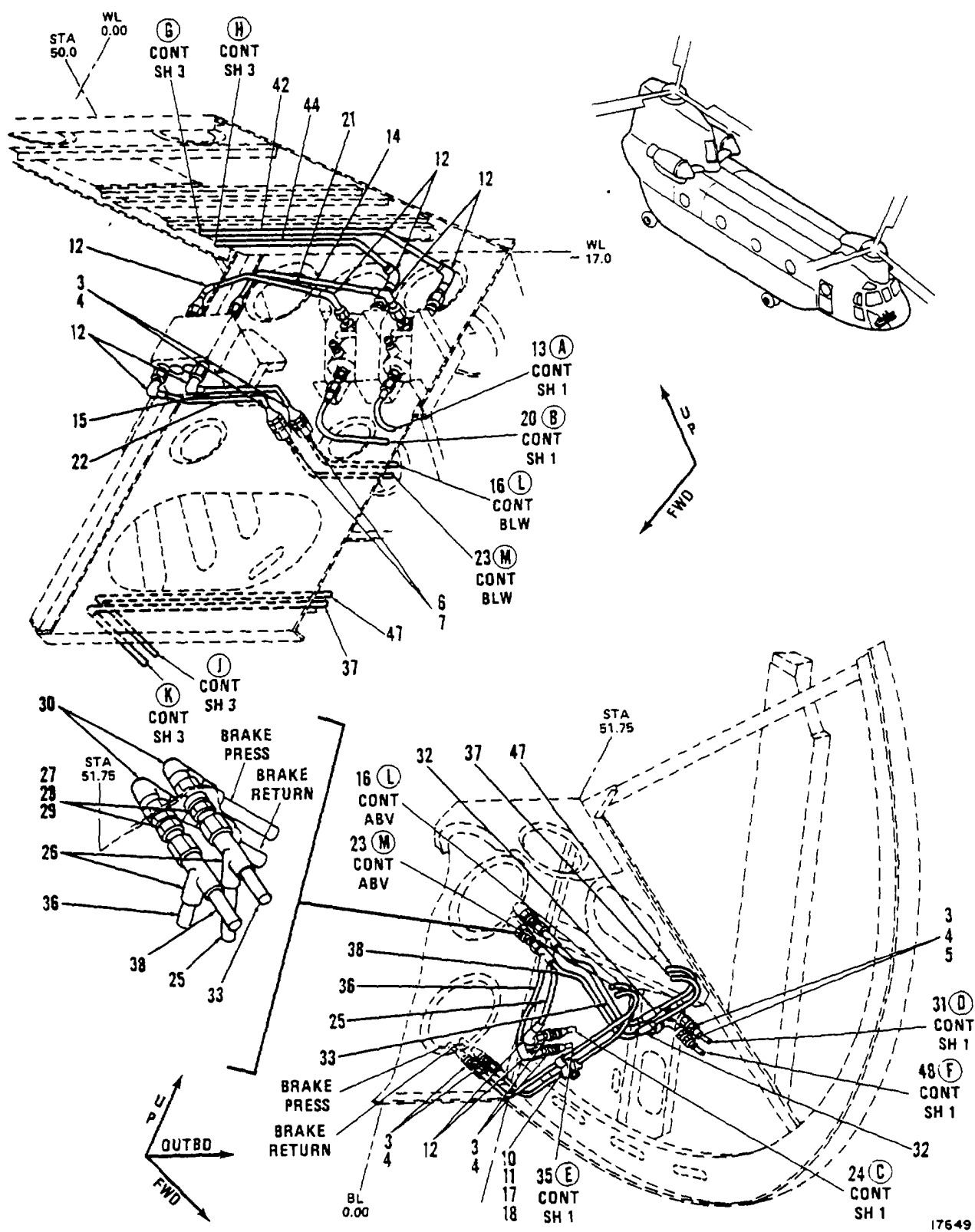
Figure 258. Tubing Instl, Hydraulic, Nose Compartment Sta 0 to 52 (Sheet 2 of 3)
