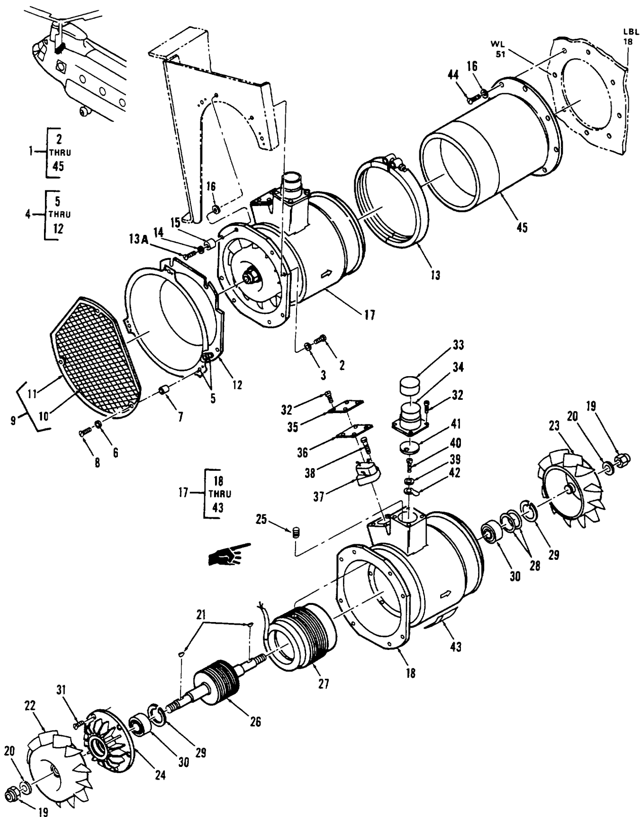
Figure 336. Cooling Instl, Avionics Equipment
