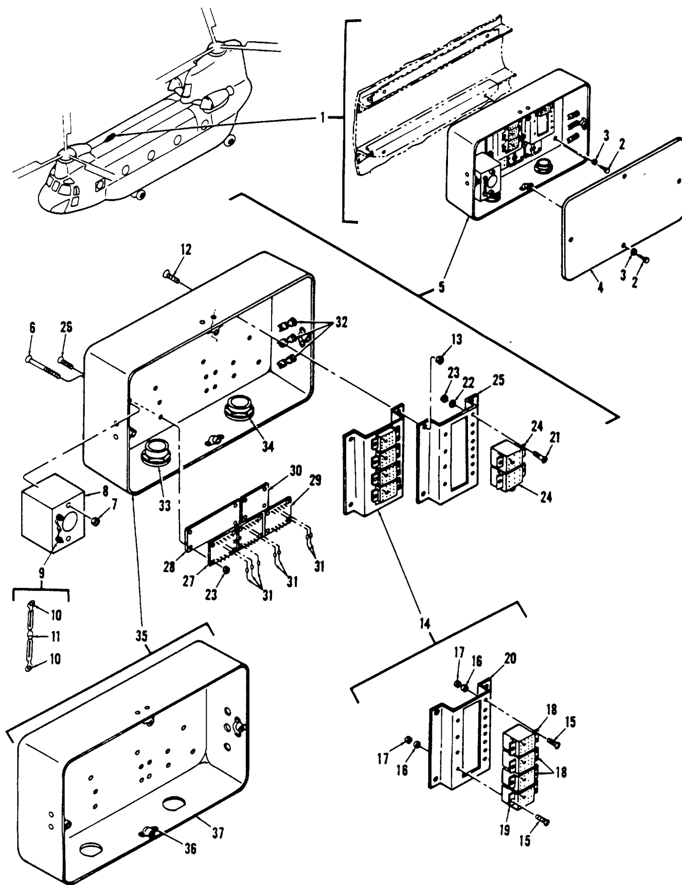
Figure 325. Box Instl, Relay, Hook Release
