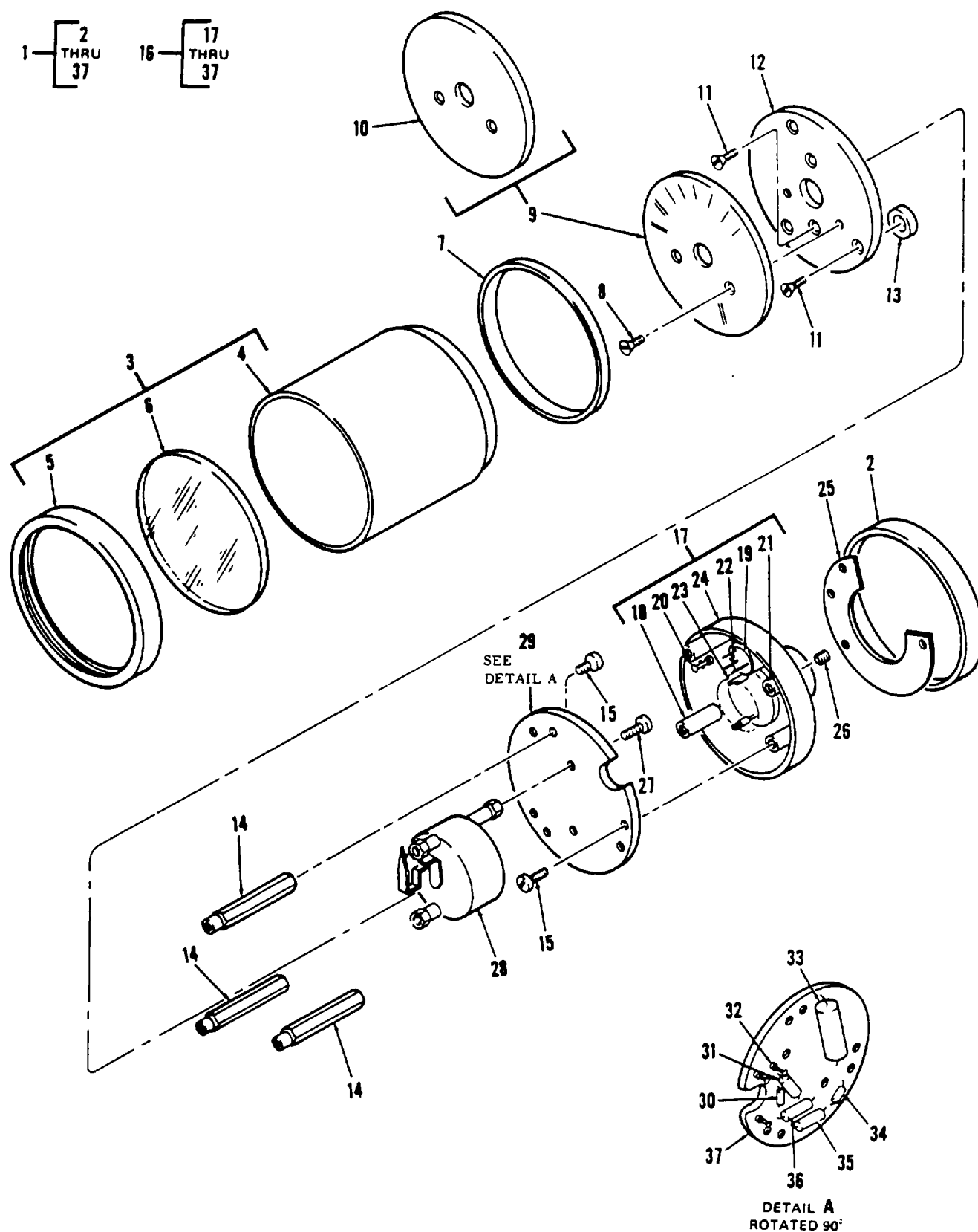
Figure 287. Indicator, Liquid Quantity, Flight Control Hydraulic Reservoir
