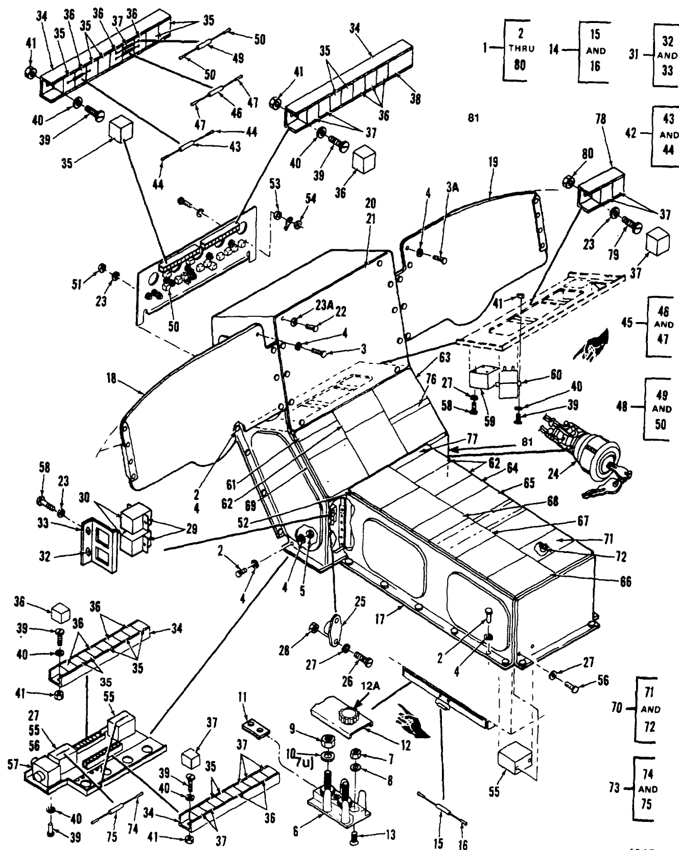
Figure 298. Console Instl, Electrical
