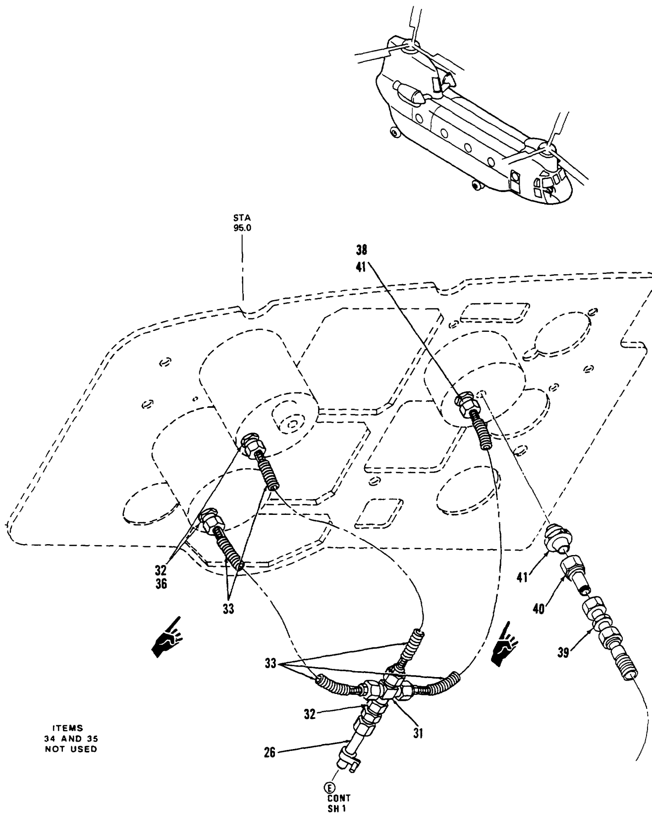
Figure 294. Tubing Instl equipment, Nose Compartment (Sheet 3 of 4)
