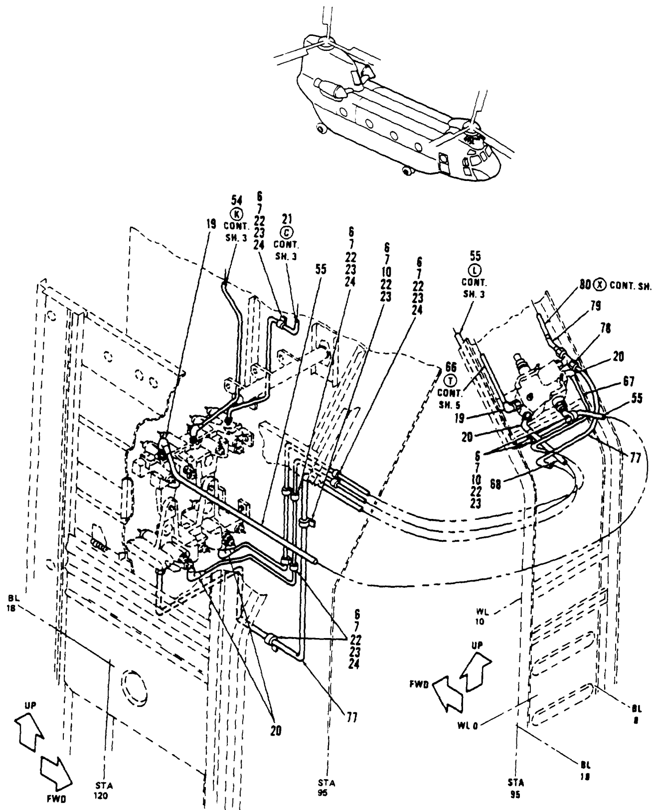
Figure 262. Tubing Instl, Hydraulics, Actuators, Fwd Transmission, Flight Controls Compartment, and Fwd Pylon (Sheet 4 of 6)
