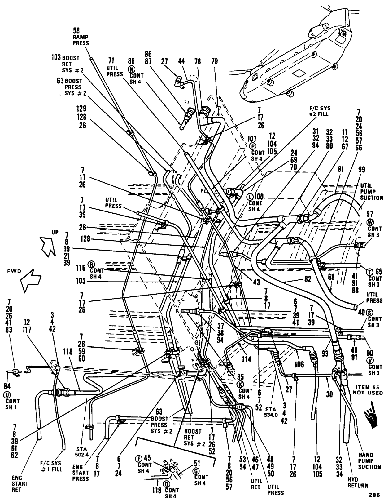
Figure 270. Tubing Instl, Hydraulic, Aft Crown Panel, RH Sta 440 to 594 (Sheet 2 of 4)
