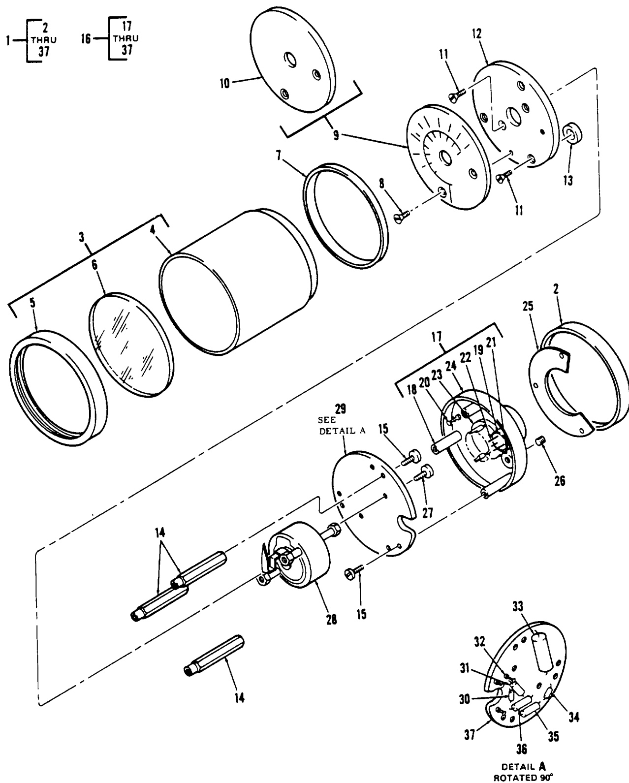
Figure 286. Indicator, Liquid Quantity, Utility Hydraulic Reservoir
