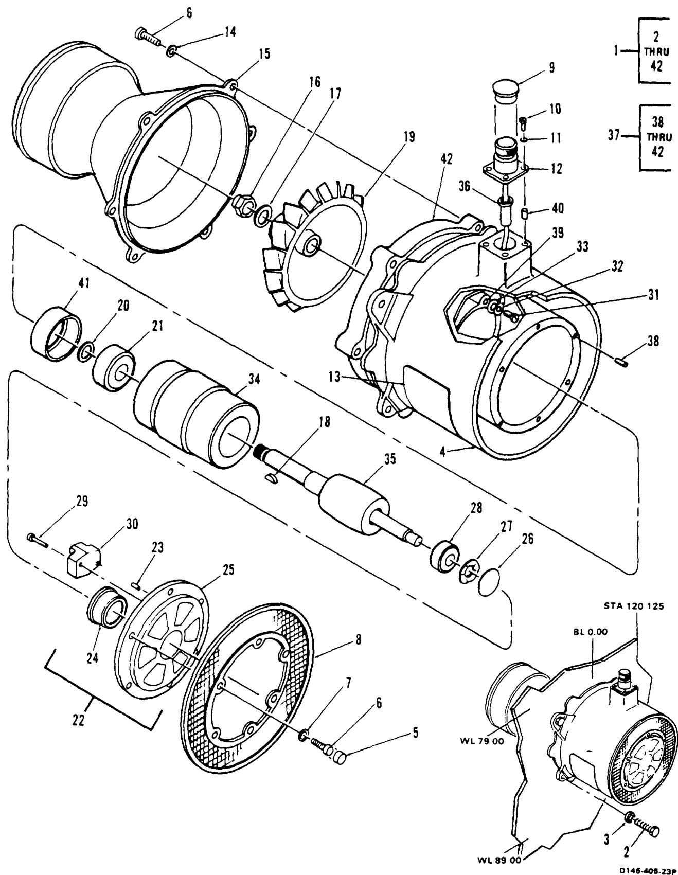
Figure 240. Equipment Instl, Cooling Fan, Fwd Pylon
