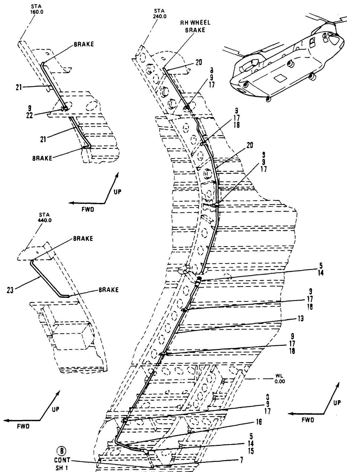
Figure 264. Tubing Instl, Hydraulic, Cabin Ceiling and Side, Lower, LH, Sta 160 to 440 (Sheet 2 of 2)
