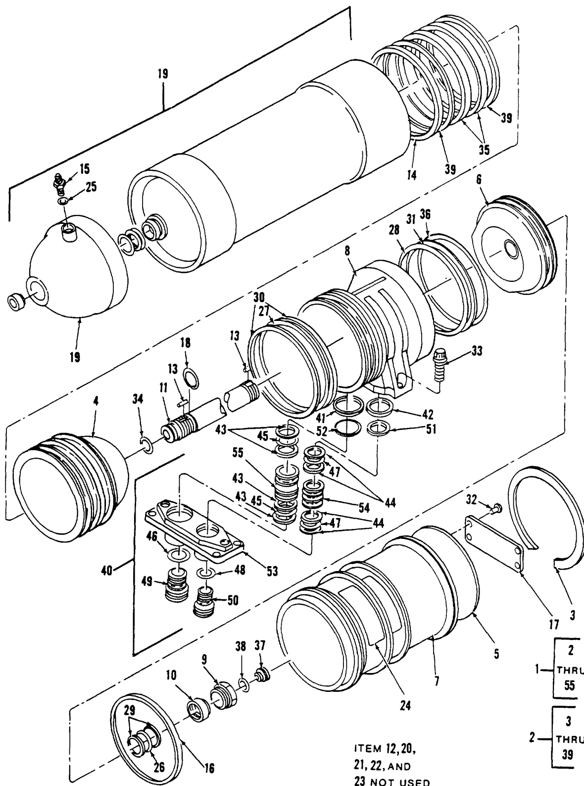
Figure 229. Accumulator Assy 28-60003-2
