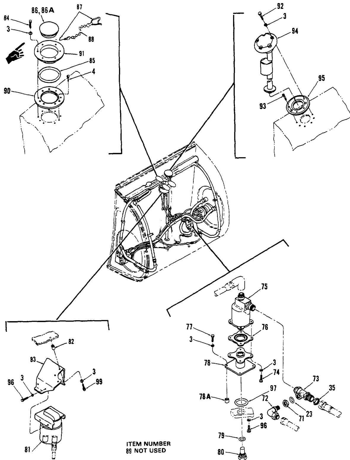
Figure 340. Fuel Cell, Fwd Auxiliary (Sheet 8 of 9)
