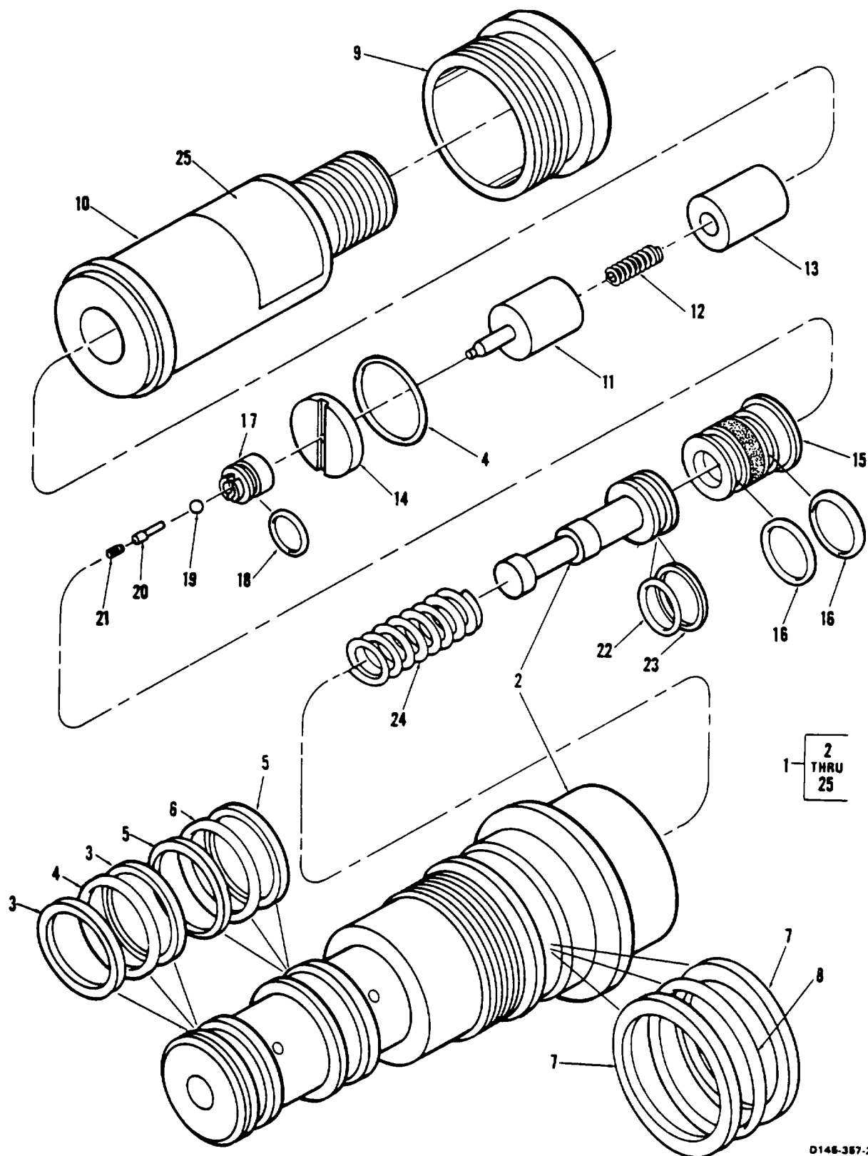
Figure 203. Valve, Solenoid 60600-20
