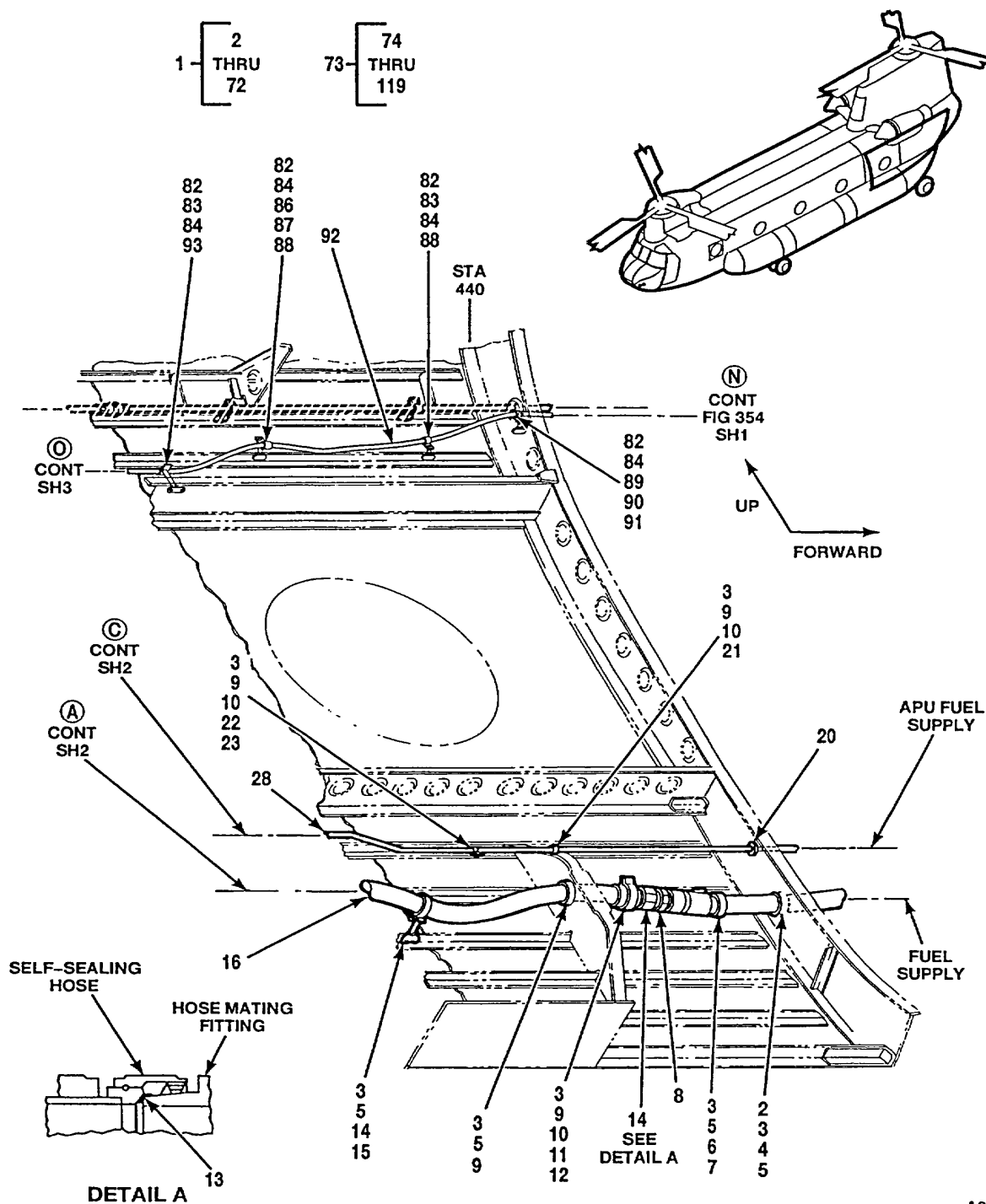
Figure 356. Tubing Instl, Aft Fuselage (Sheet 1 of 4)
