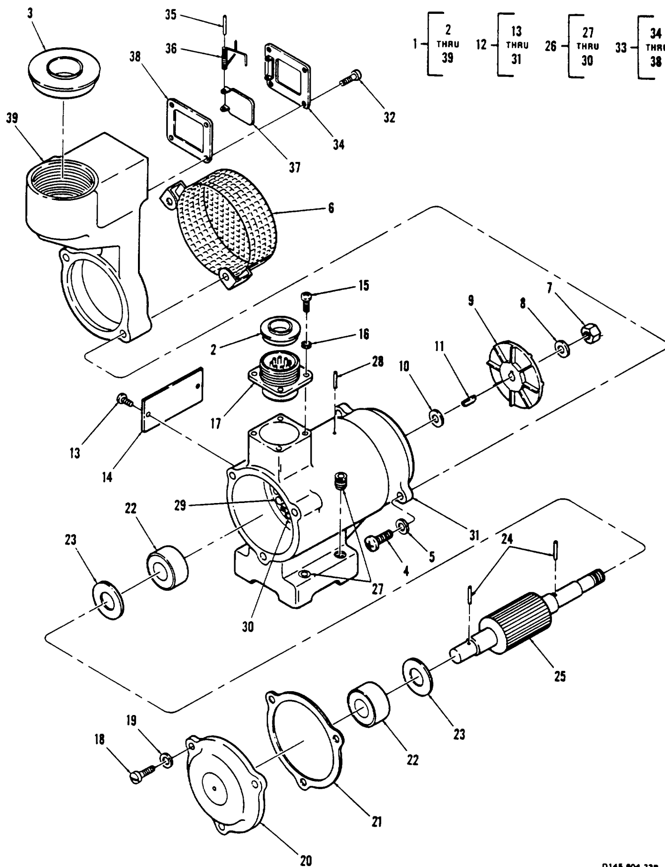
Figure 341. Pump, Centrifugal
