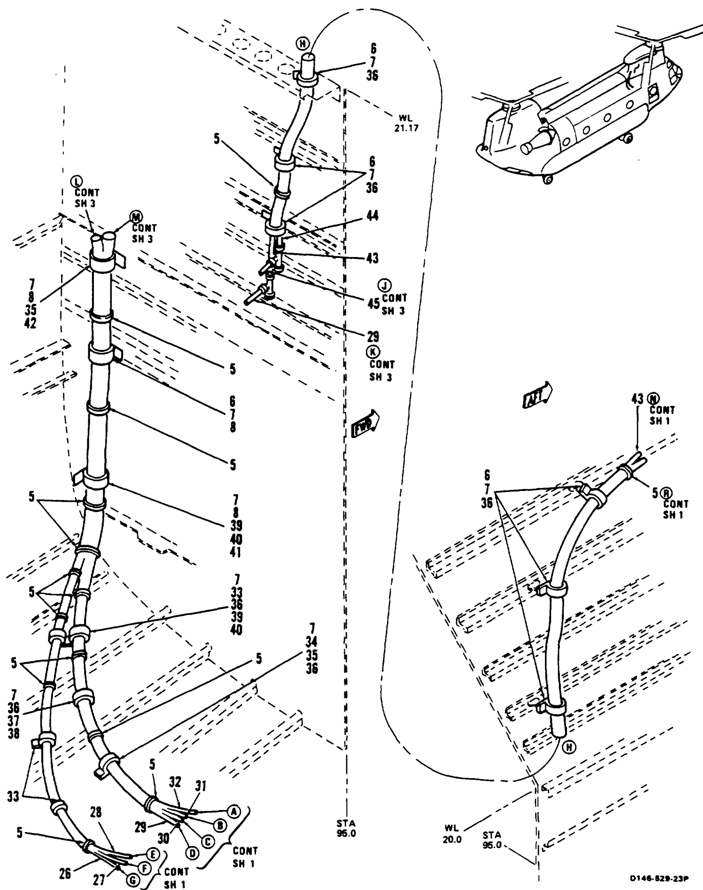
Figure 296. Tubing Instl, Equipment, Crown Panel and Side, LH Sta 120 to 160 (Sheet 2 of 3)
