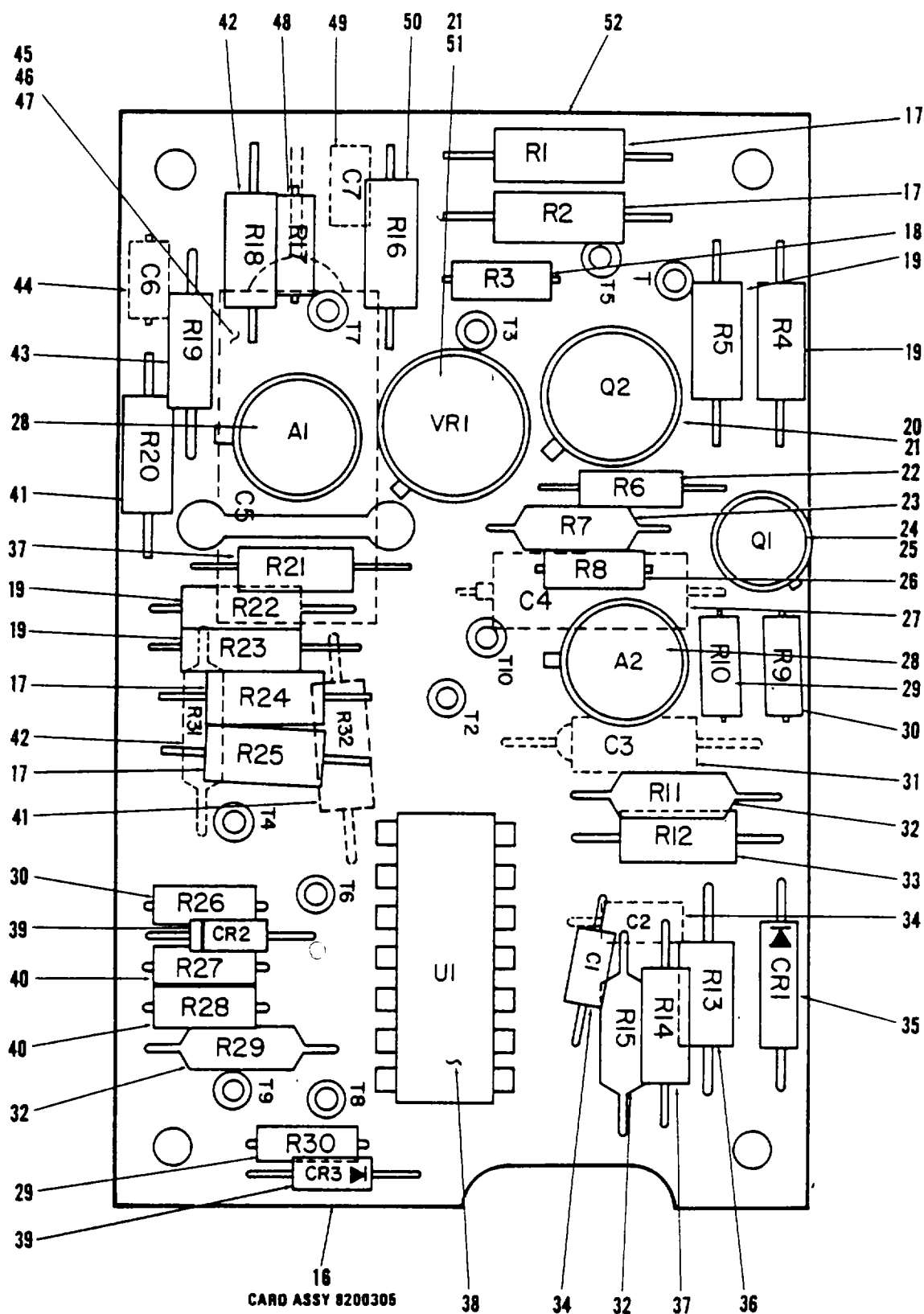
Figure 285. Signal Conditioner Instl, Fwd Pylon CGI (Sheet 3 of 3)
