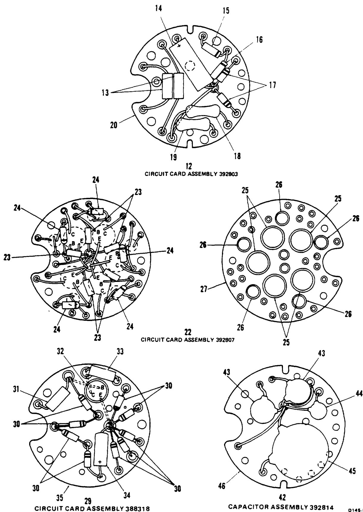
Figure 282. Switch, Selector (Sheet 2 of 2)
