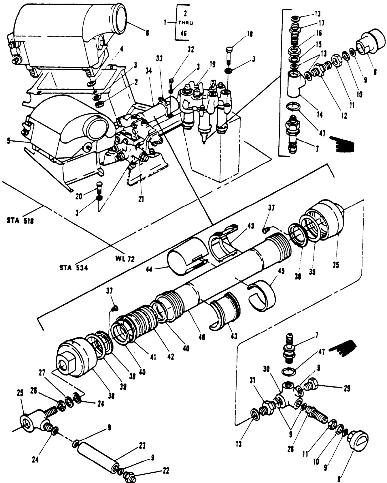
Figure 215. Equipment Instl, Sta 482 To 584, Above WL 72
