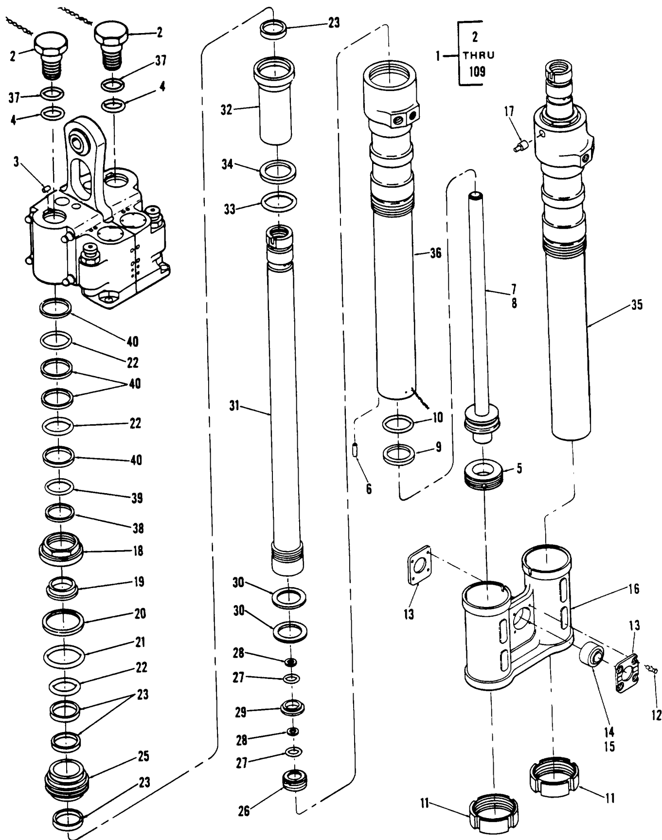
Figure 243. Servocylinder, Swiveling (Sheet 1 of 4)
