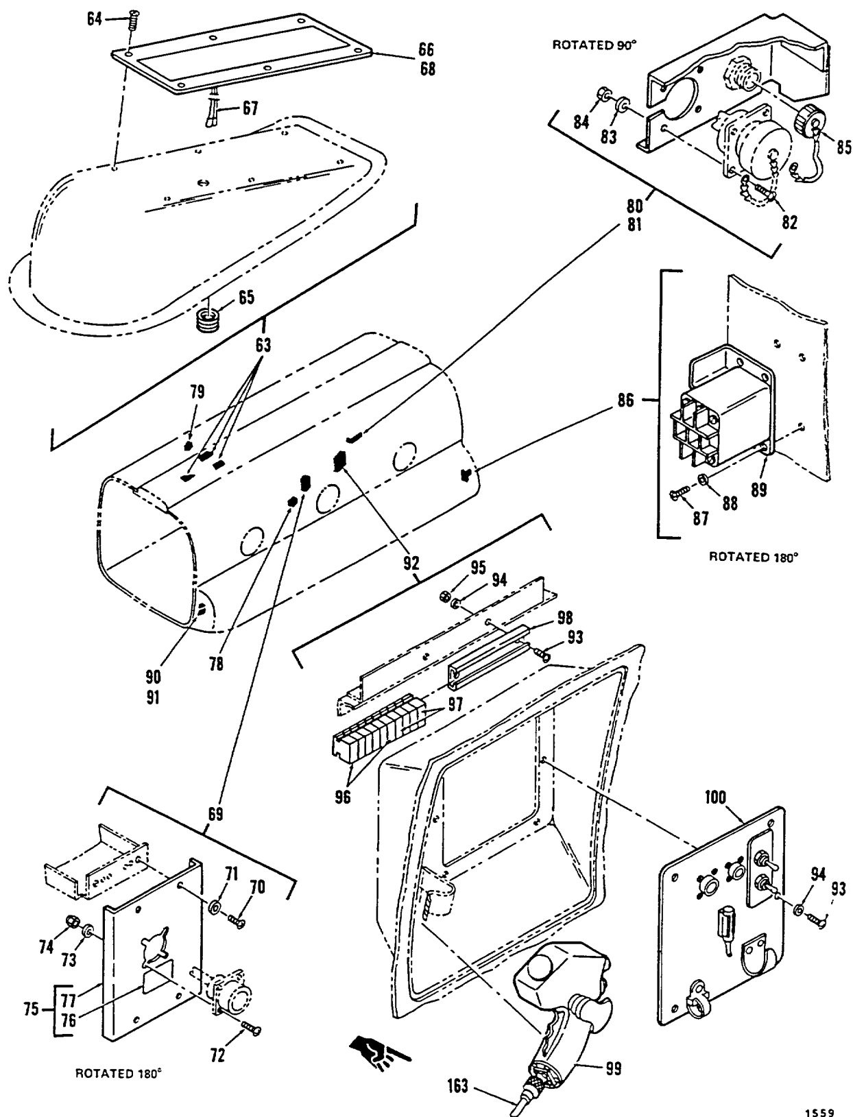
Figure 323. Equipment Instl, Cabin (Sheet 2 of 4)
