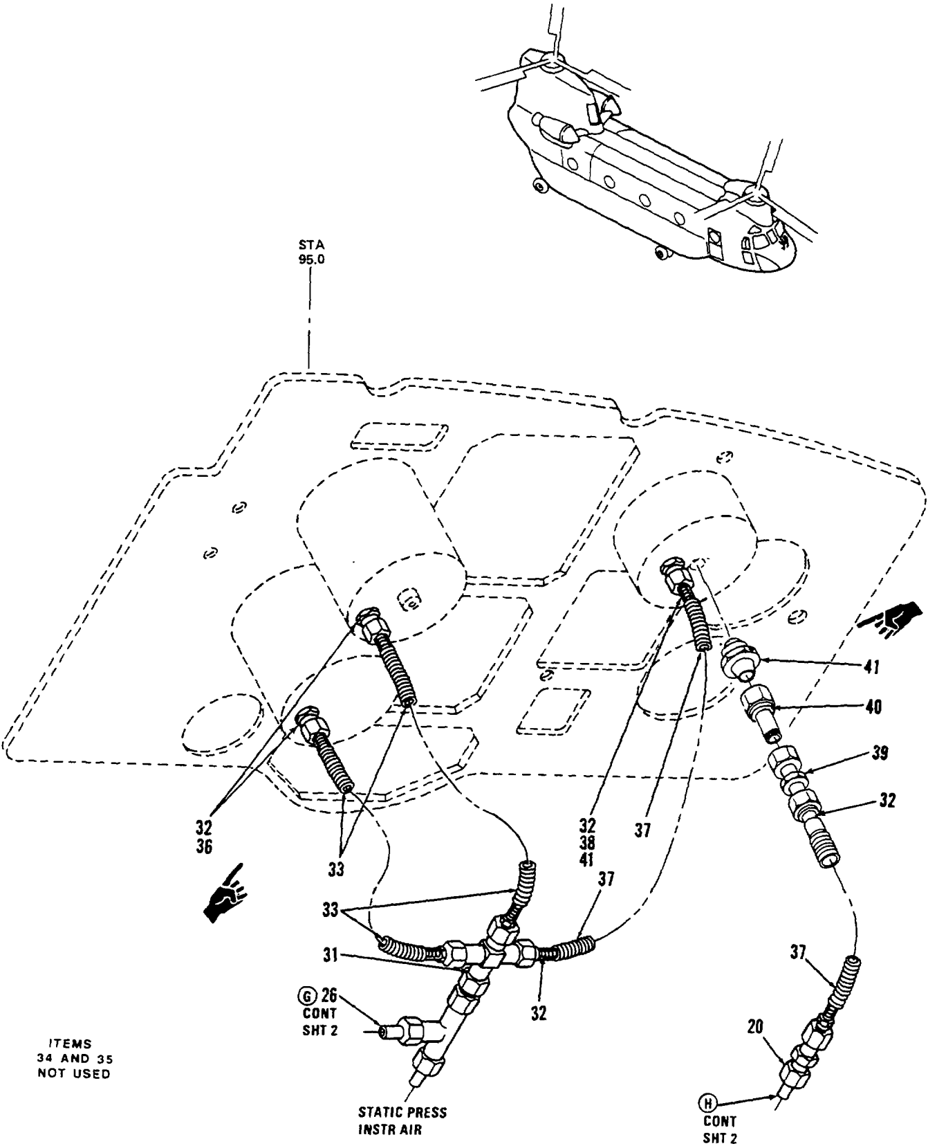
Figure 294. Tubing Instl equipment, Nose Compartment (Sheet 4 of 4)
