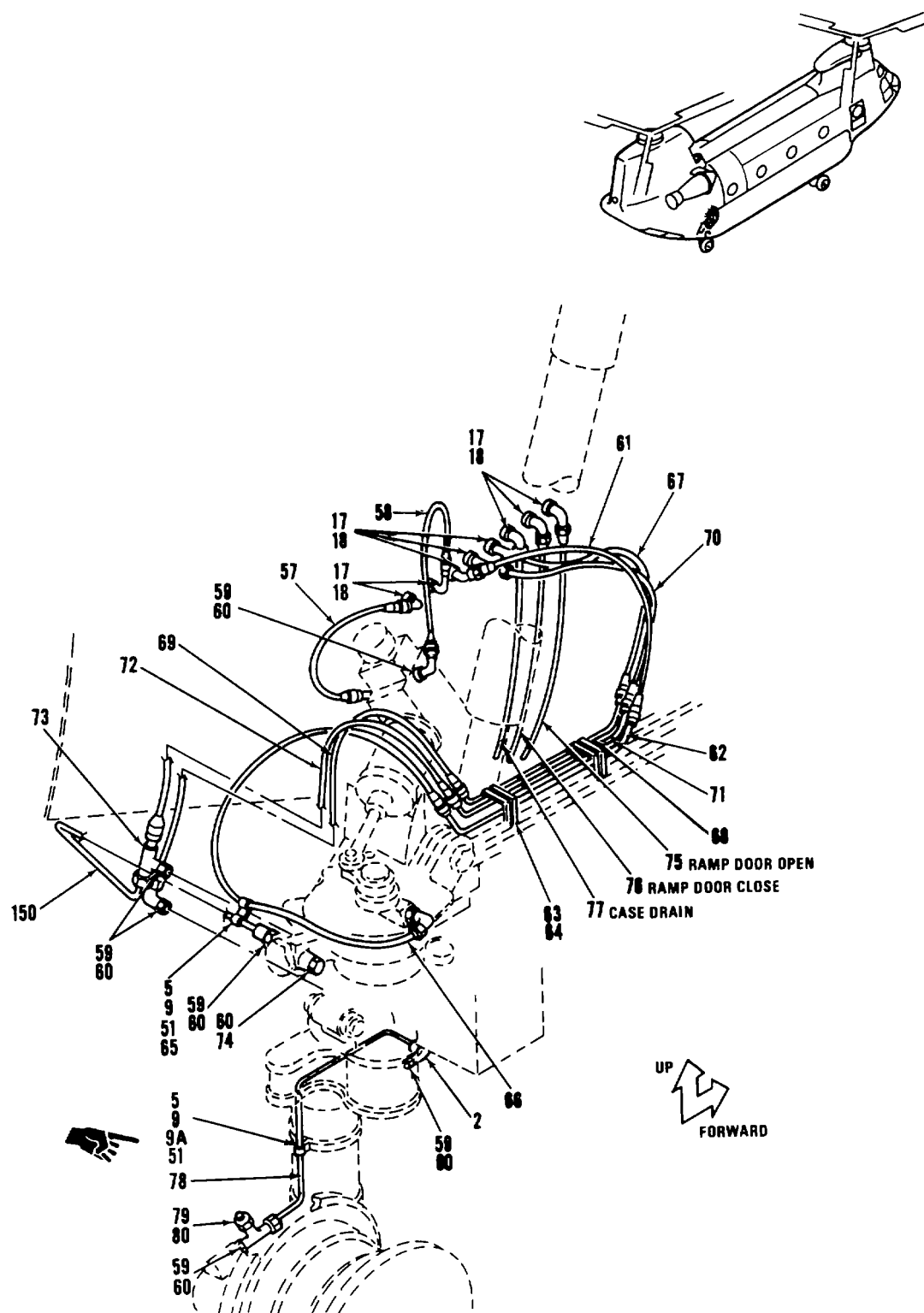
Figure 268. Tubing Instl, Hydraulic, Aft Fuselage, Lower, RH Sta 440 to 594 (Sheet 5 of 5)
