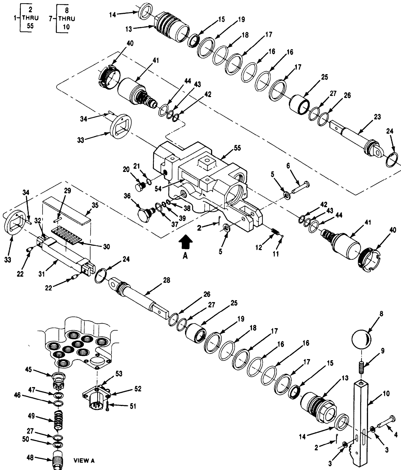
Figure 214A. Valve, Linear Direction Control
