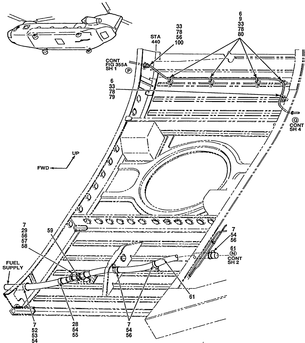
Figure 357. Tubing Instl, Aft Fuselage (Sheet 5 of 5)
