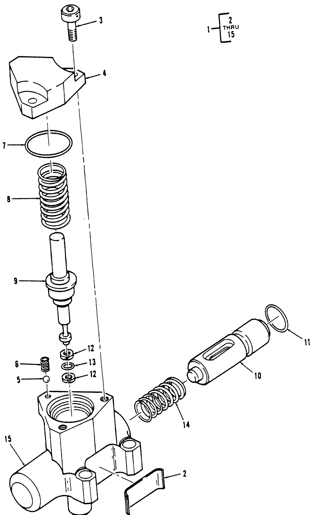
Figure 249. Indicator, Cylinder
