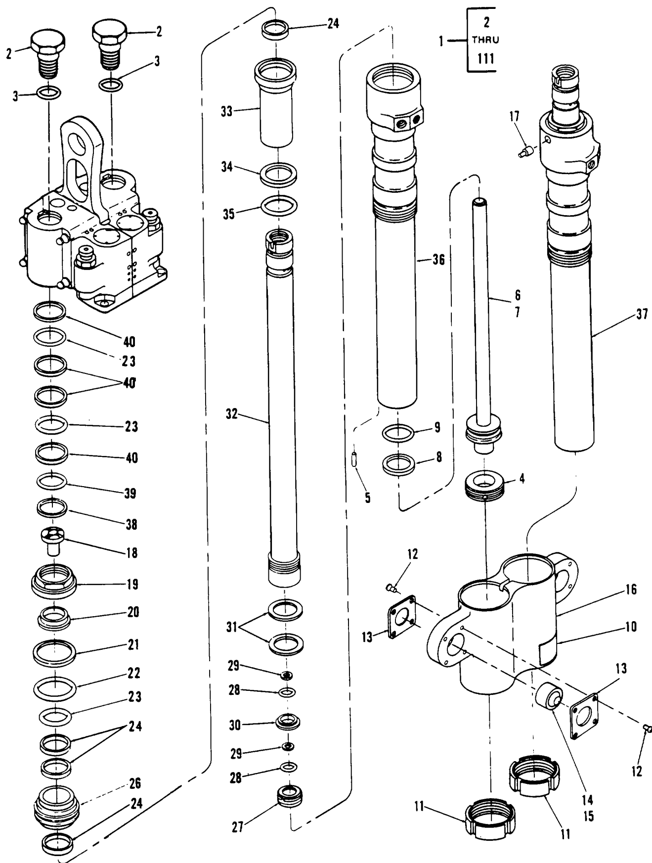
Figure 244. Servocylinder, Pivoting (Sheet 1 of 4)
