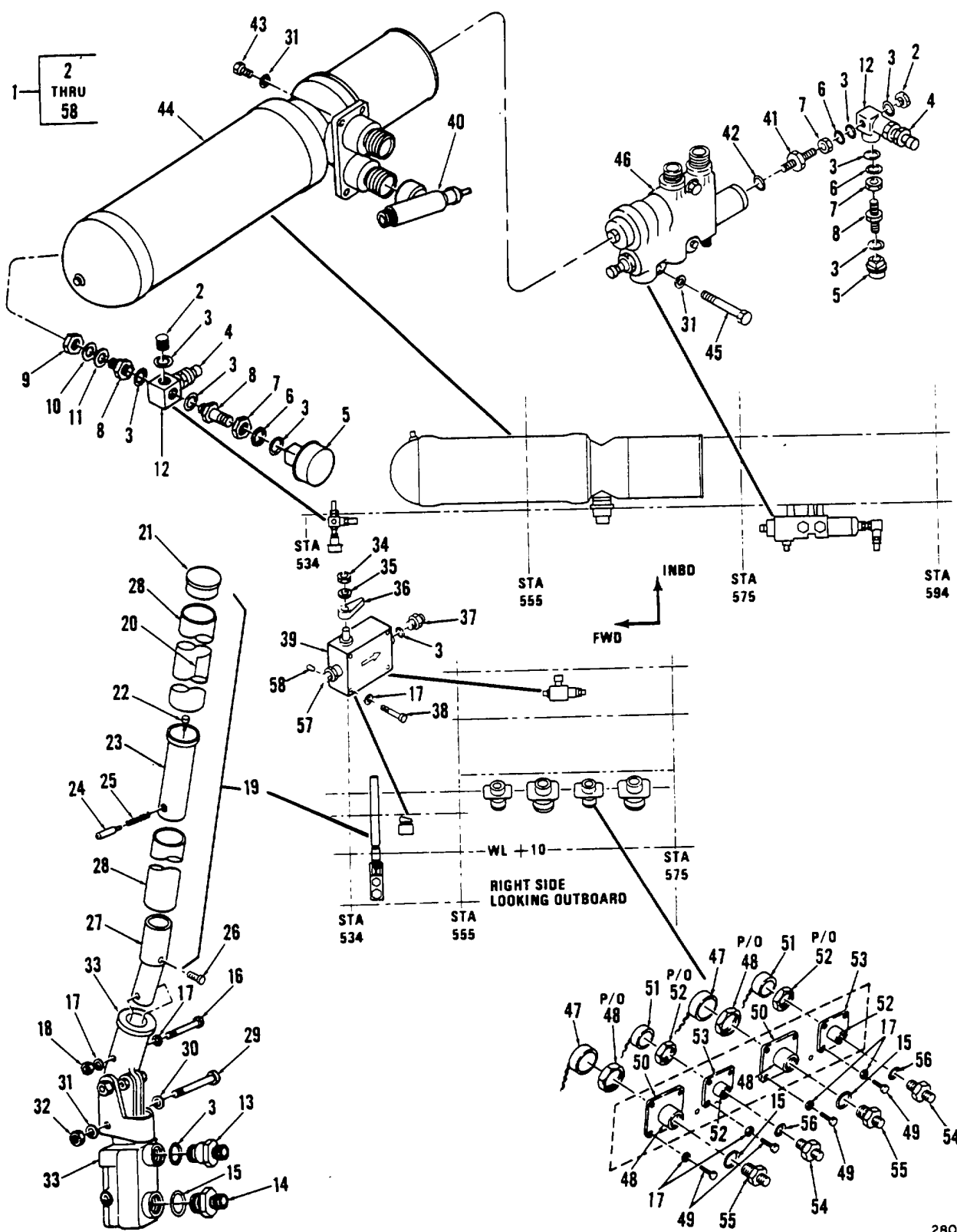
Figure 228. Equipment Instl, Sta 534 to 594 (Sheet 1 of 2)
