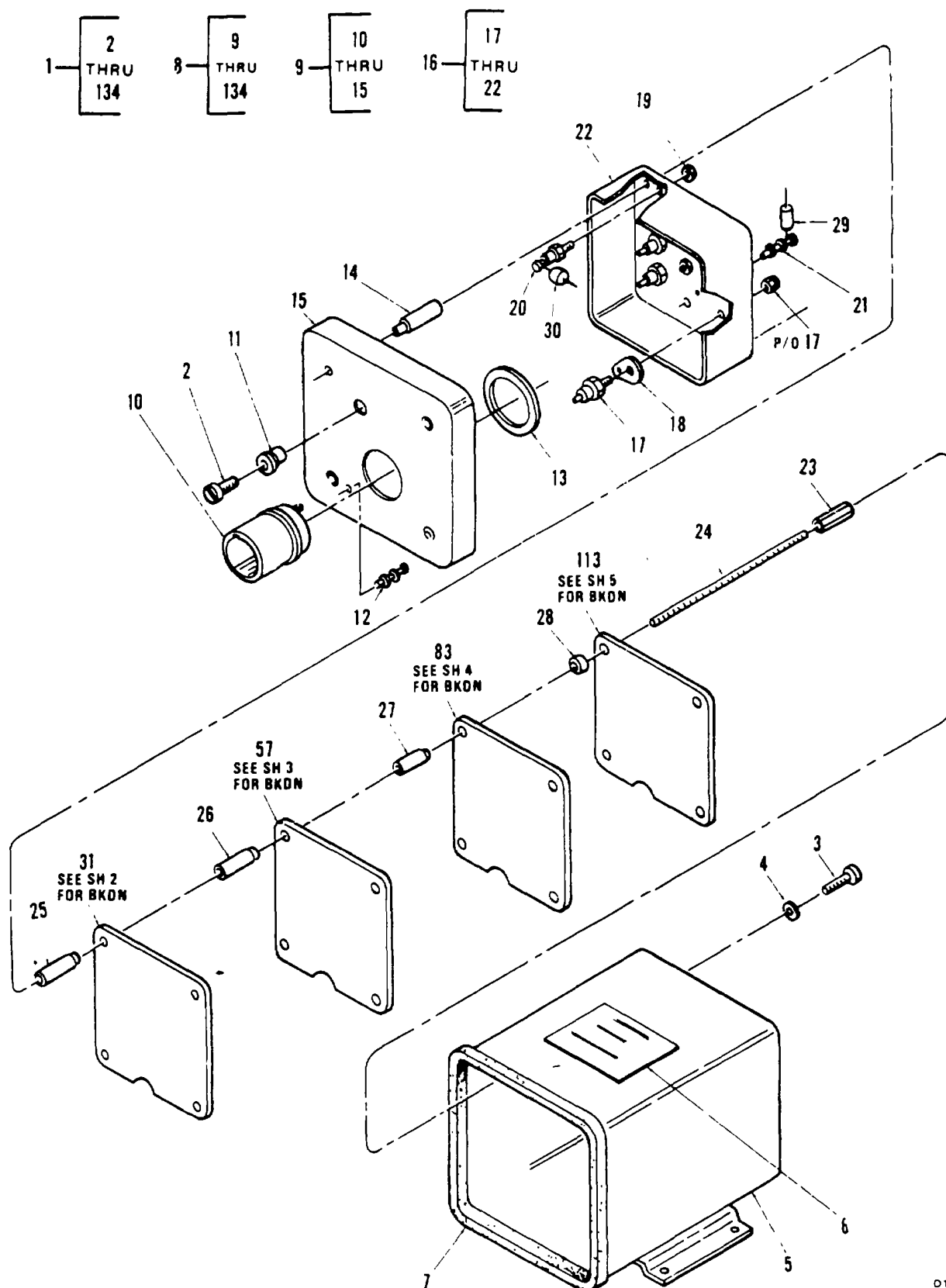
Figure 289. Signal Conditioner, Indicator, Liquid (Sheet 1 of 5)
