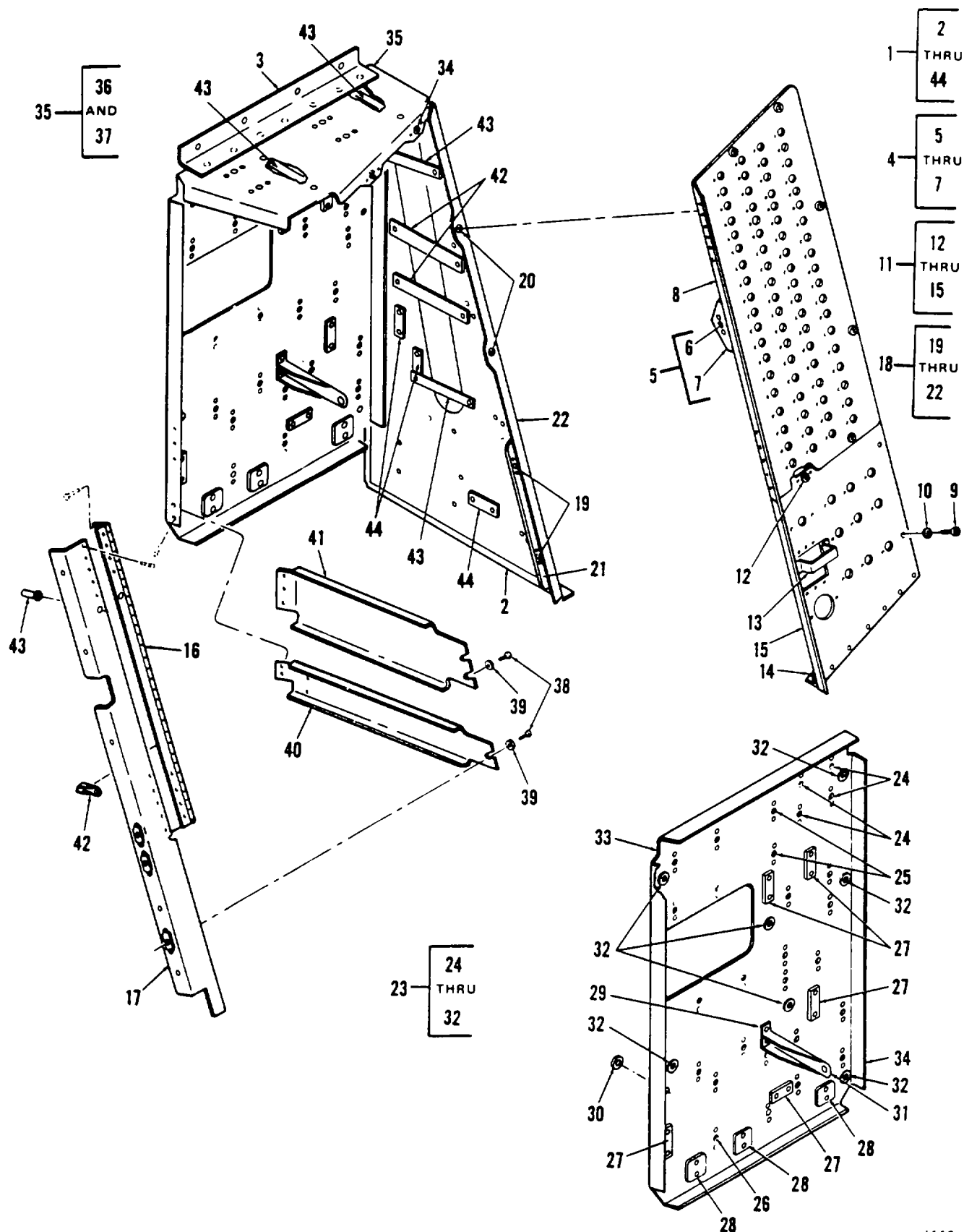
Figure 310. Structure, Power Distribution Panel, RH
