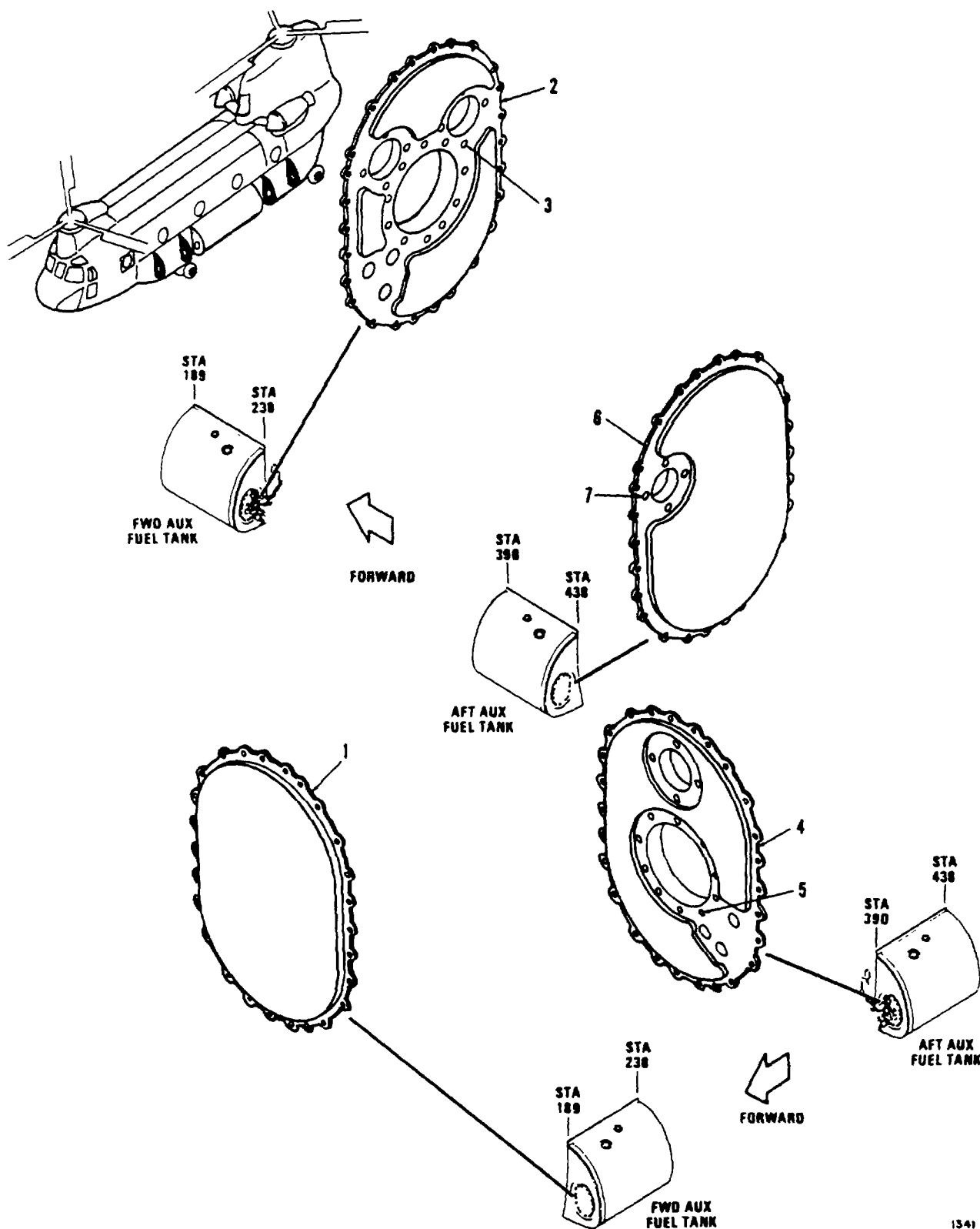
Figure 360. Door, Auxiliary Tank
