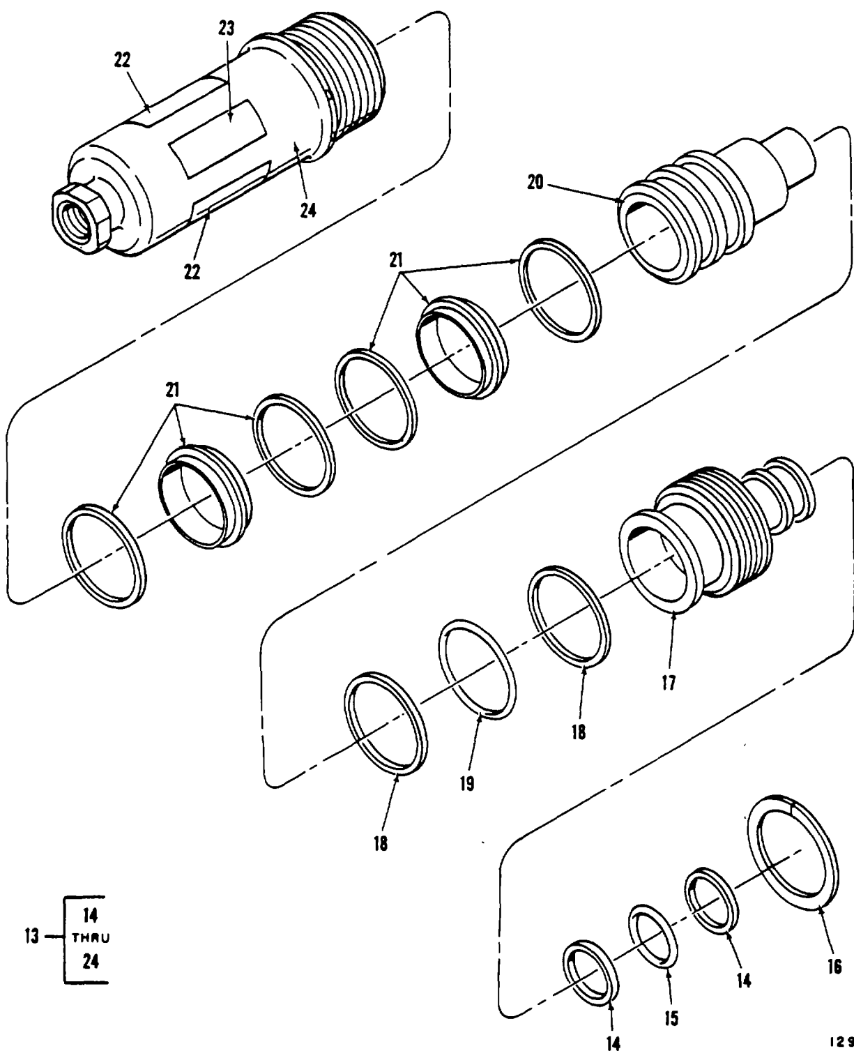
Figure 235. Accumulator, Hydraulic (Sheet 2 of 2)
