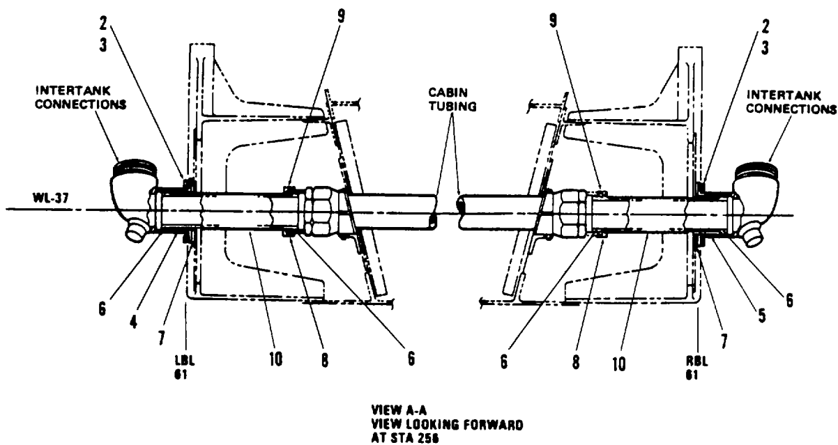
Figure 351. Plumbing Instl, Fuel, Fuselage (Sheet 1 of 5)
