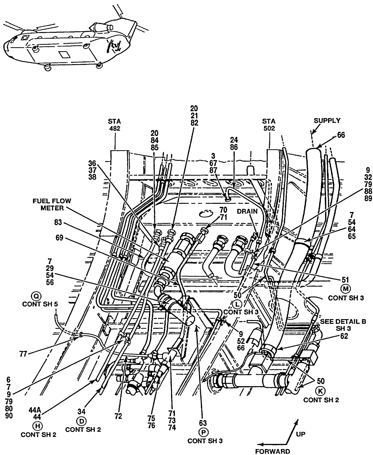
Figure 357. Tubing Instl, Aft Fuselage (Sheet 4 of 5)
