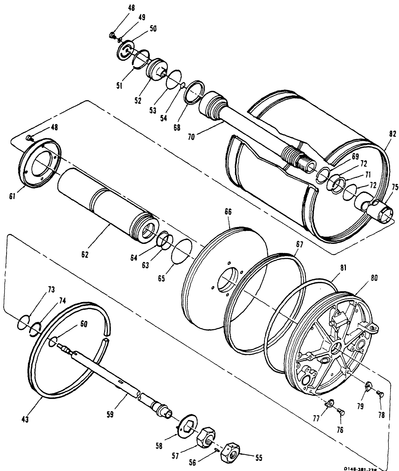
Figure 217. Reservoir/ Cooler 1711019-002 (Sheet 3 of 3)
