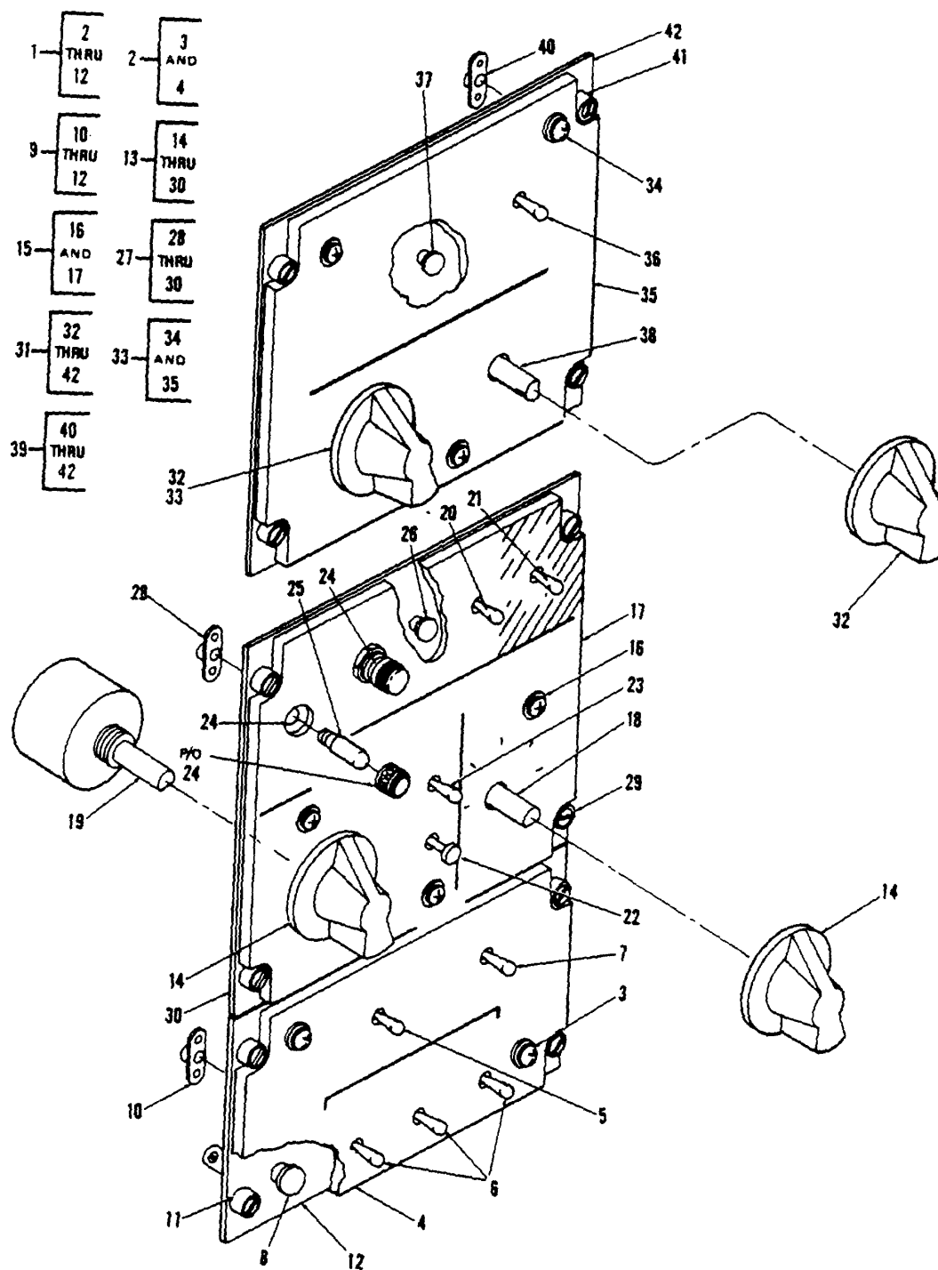
Figure 313. Panel , Electrical Power, Heating and Lighting and Troop Warning /Heater
