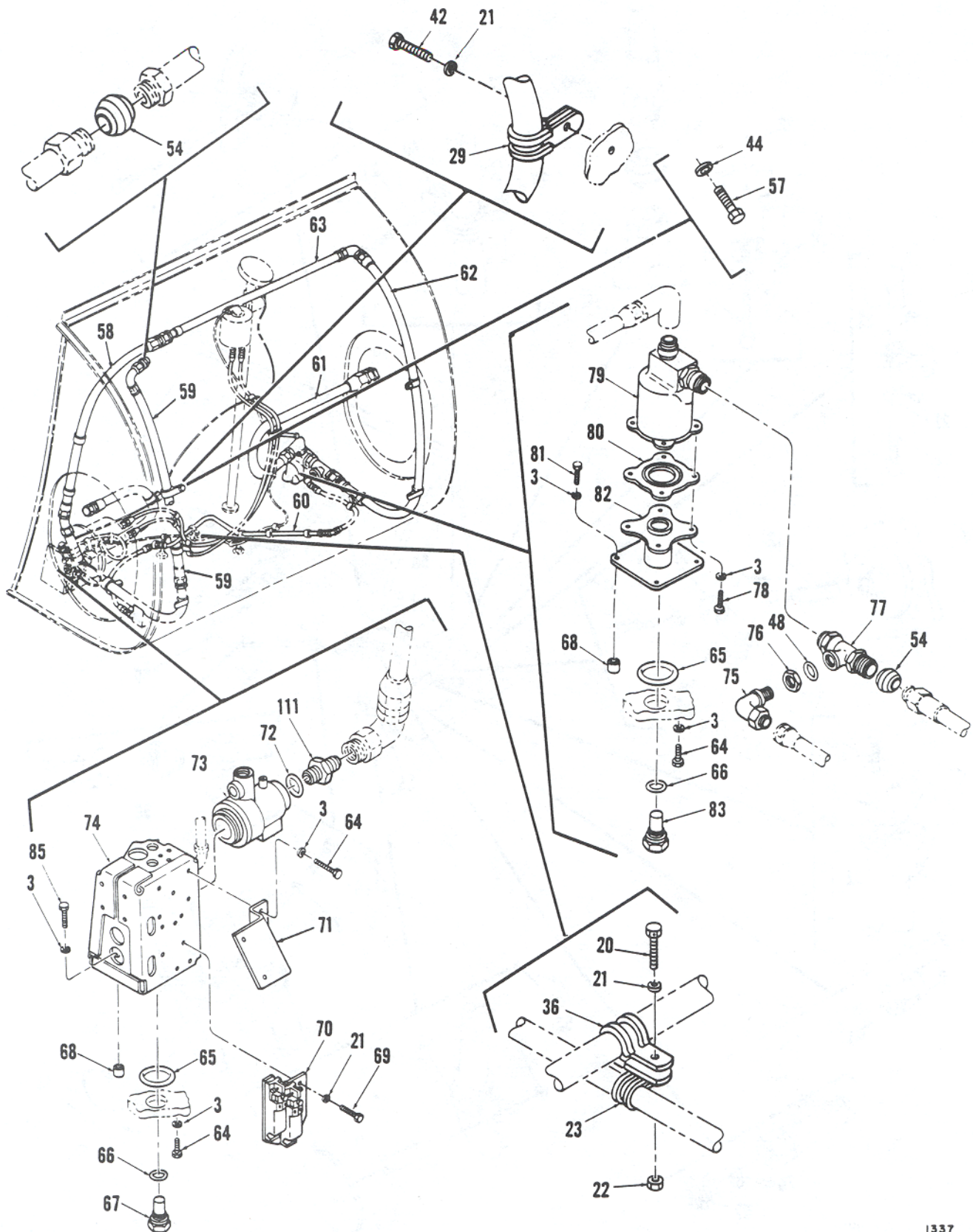
Figure 346. Fuel Cell, Aft Auxiliary (Sheet 4 of 6)
