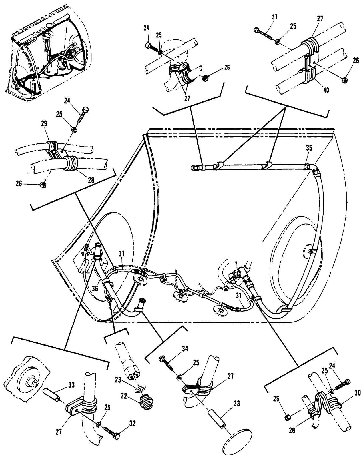
Figure 340. Fuel Cell, Fwd Auxiliary (Sheet 2 of 9)
