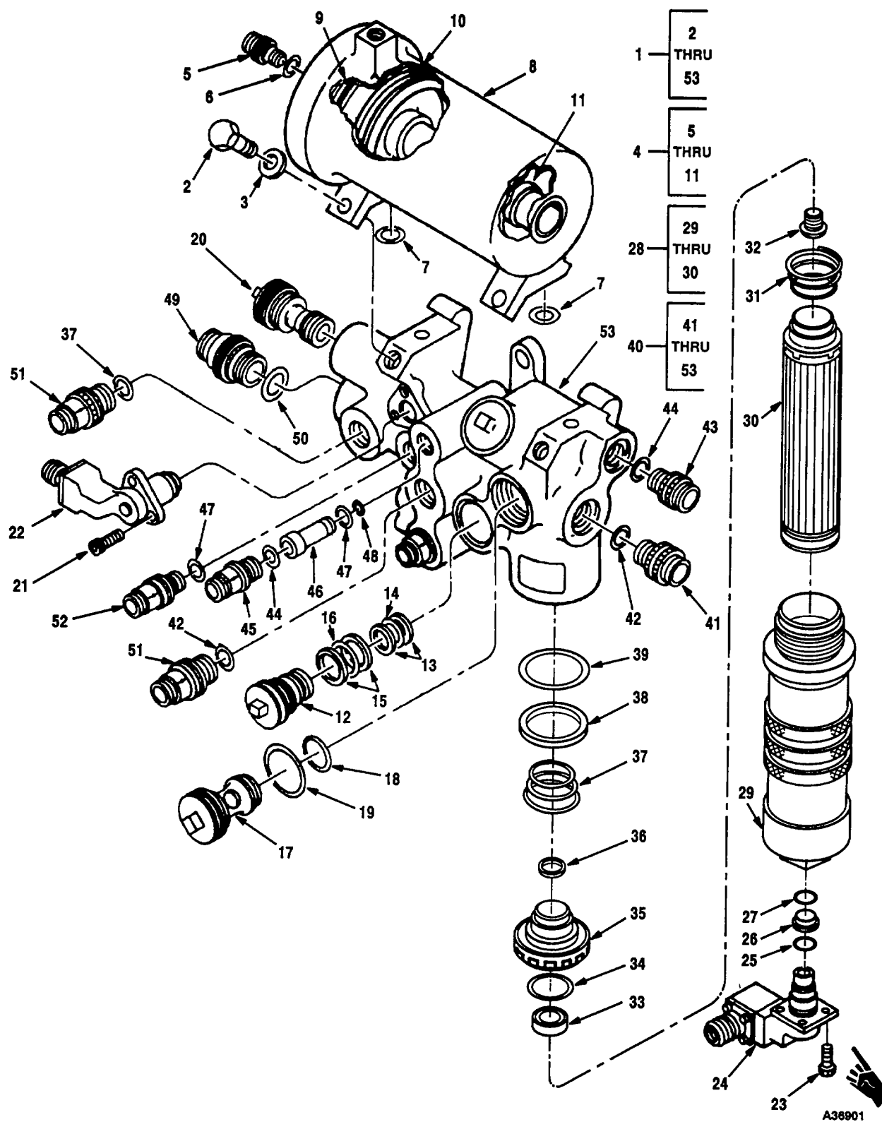
Figure 227. Module, Return AE-620-23
