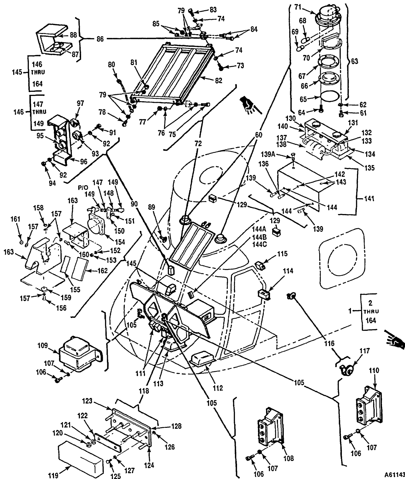
Figure 303. Equipment Instl, Nose, Electrical (Sheet 2 of 2)
