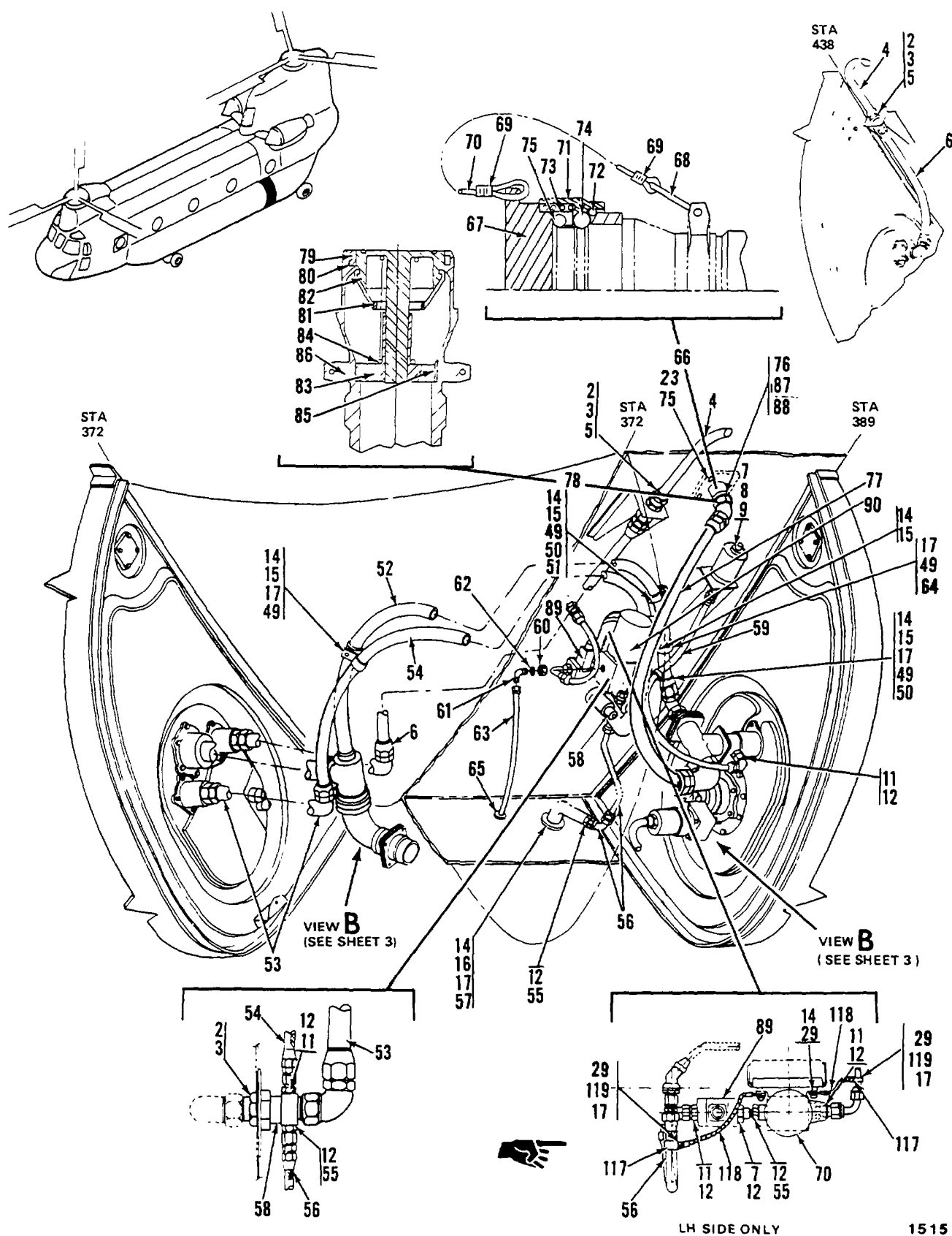
Figure 347. Intertank connection Instl, LH (Sheet 2 of 5)
