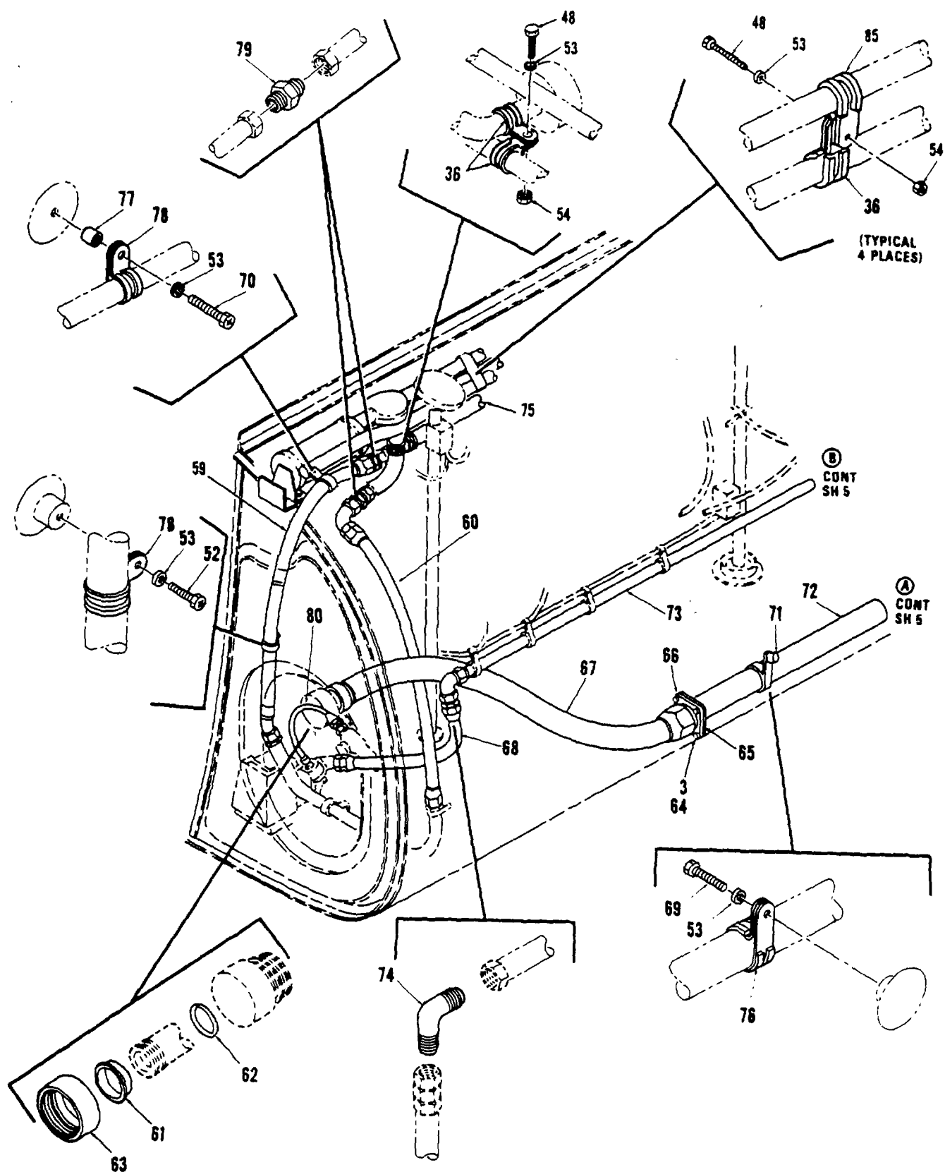
Figure 345. Fuel Cell, Main (Sheet 4 of 8)
