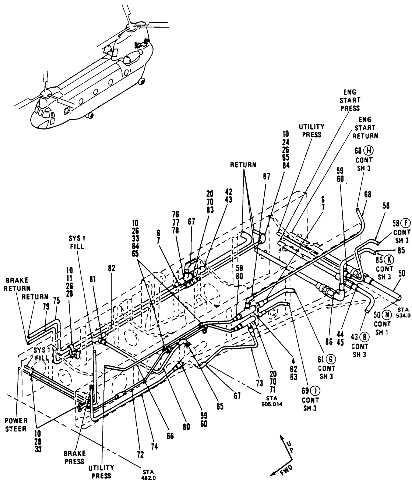
Figure 269. Tubing Instl, Hydraulic, Aft Crown Panel, LH Sta 440 to 594 (Sheet 4 of 4)
