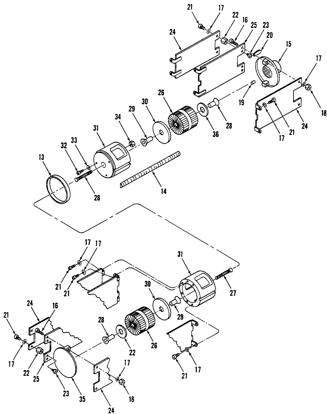
Figure 290. Power Supply, Fuel Flow (Sheet 2 of 2)
