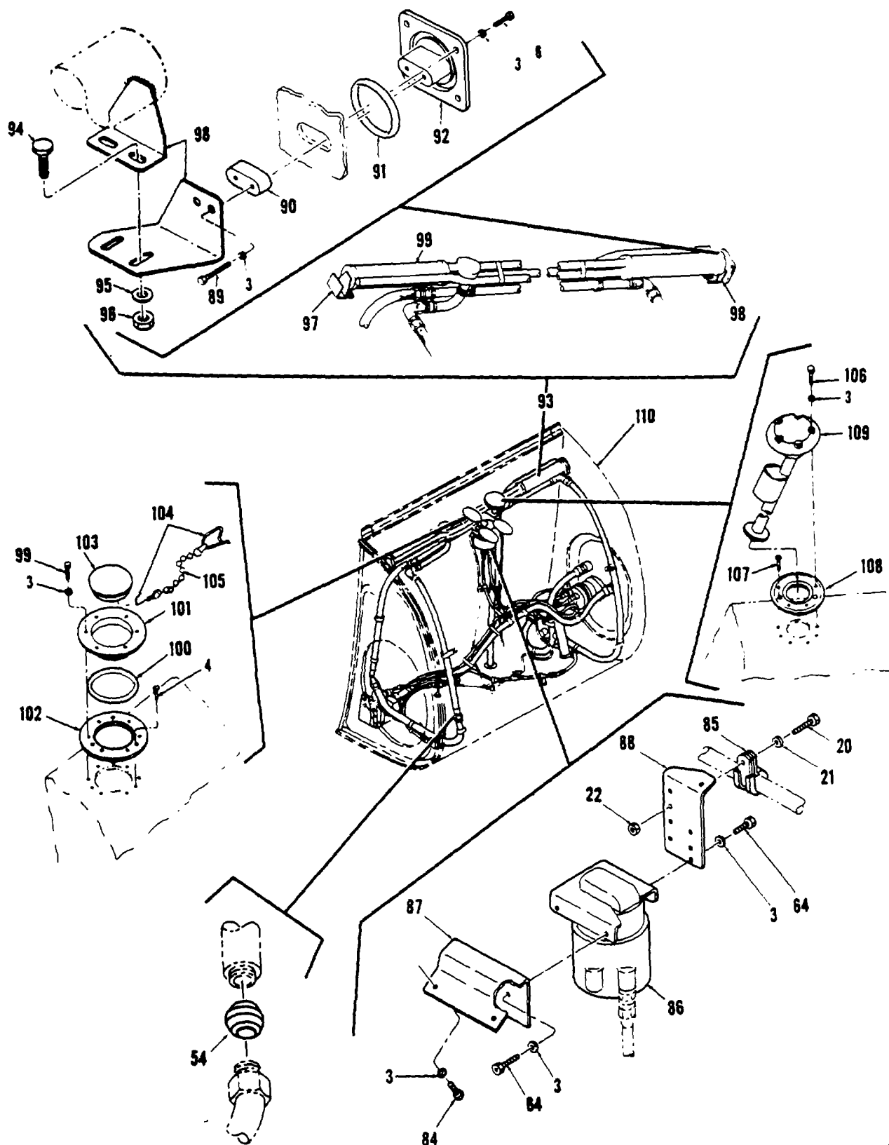
Figure 346. Fuel Cell, Aft Auxiliary (Sheet 6 of 6)
