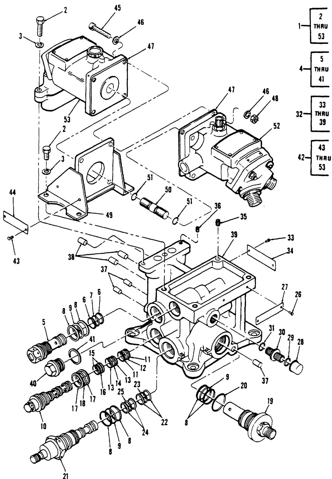
Figure 219. Power Transfer Unit
